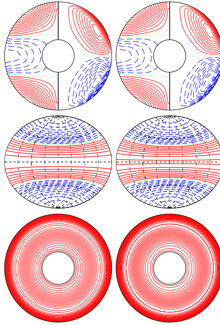
a.e03p10t03r-50000m1n2N2z4e3Y E_{\text{kin}}
