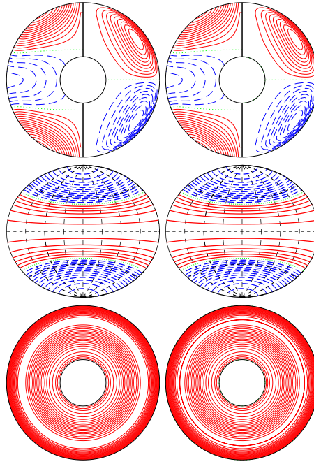
a.e03p01t03r-50000m1n2N2z4e2Y E_{\text{kin}}
