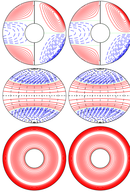
a.e03p05t03r-50000m1n2N2z4e2Y E_{\text{kin}}
