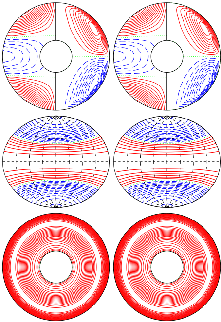
a.e03p01t03r-50000m1n2N2z4e3Y E_{kin}
