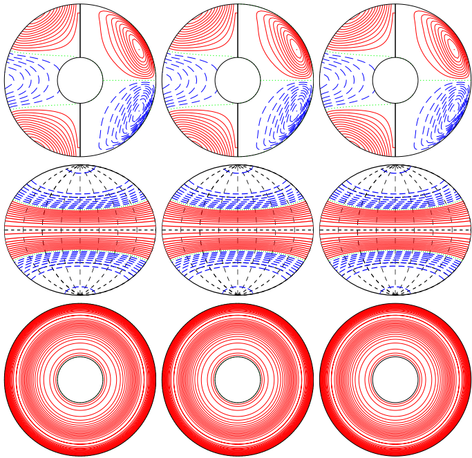
a.e03p01t03r-50000m1n2N2z4e4Y E_{\text{kin}}
