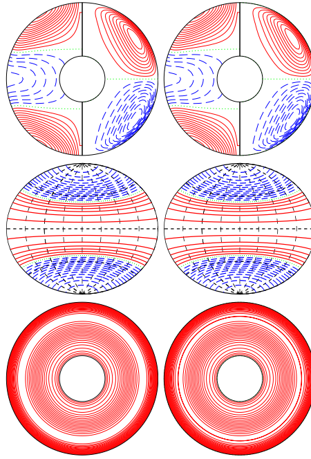
a.e03p01t03r-50000m1n2N2z4e1Y E_{\text{kin}}
