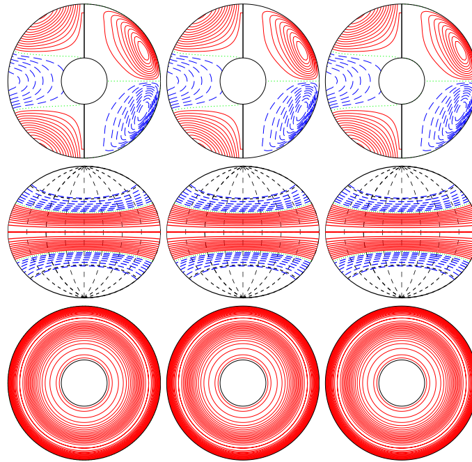
a.e03p05t03r-50000m1n2N2z4e4Y E_{\text{kin}}
