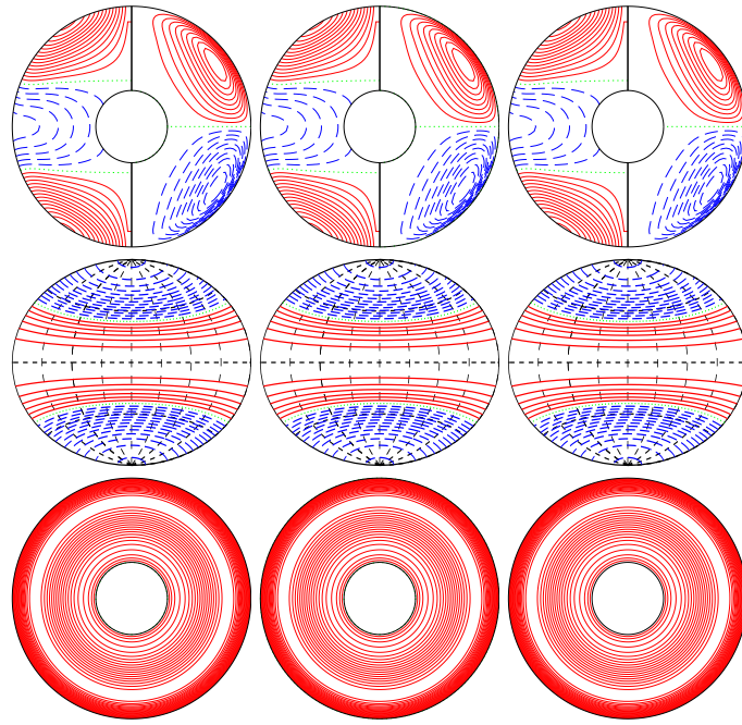
a.e03p01t03r-50000m1n2N2z4e3Y E_{\text{kin}}
