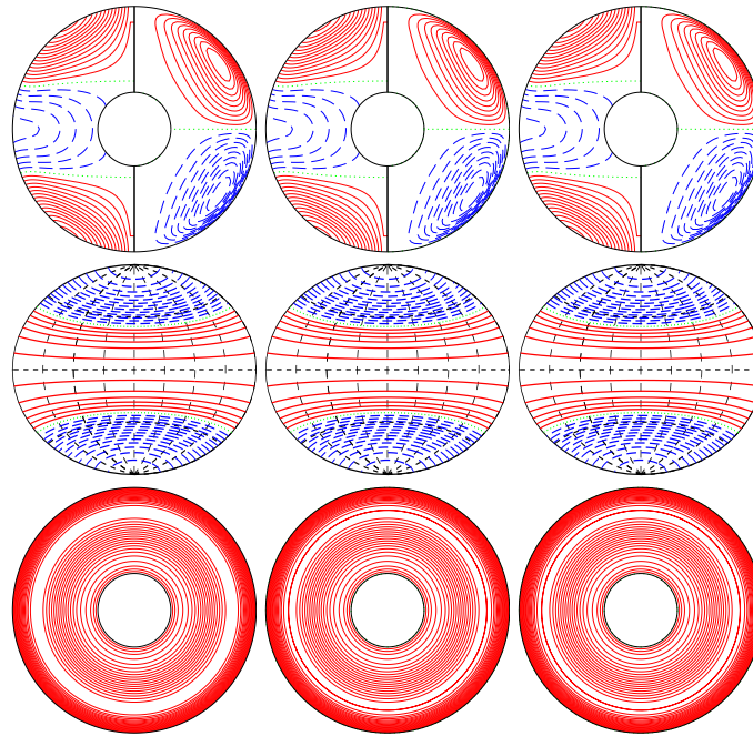
a.e03p01t03r-50000m1n2N2z4e1Y E_{\text{kin}}
