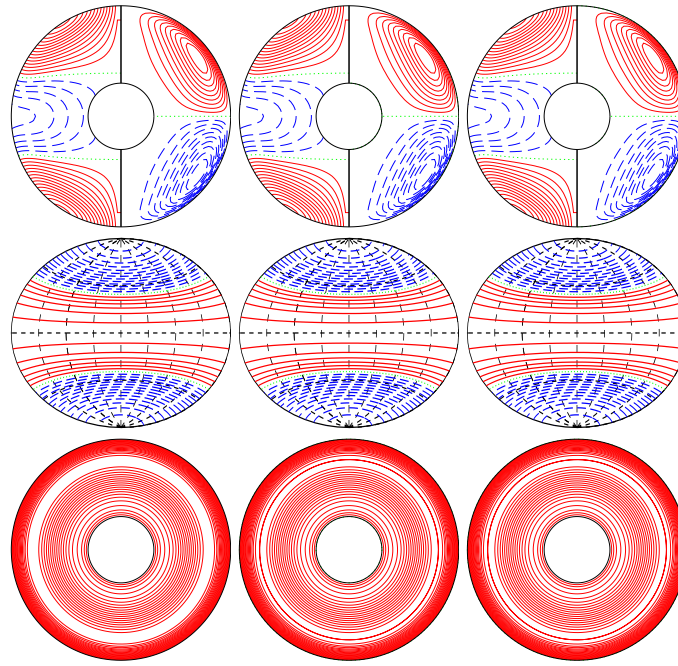
a.e03p01t03r-50000m1n2N2z4e2Y E_{\text{kin}}
