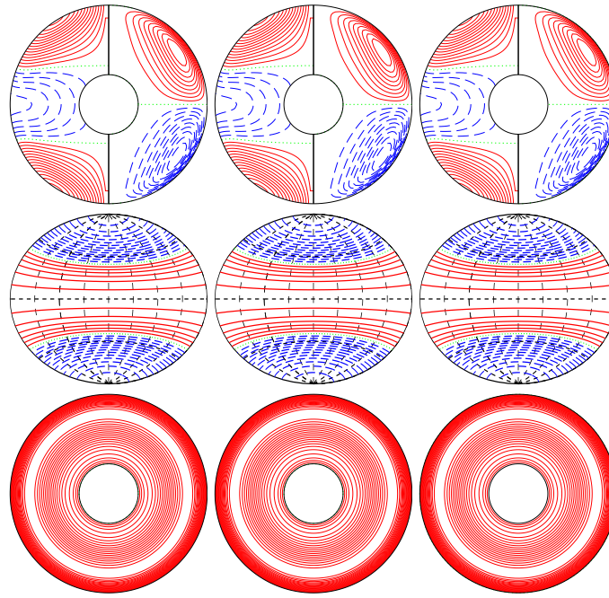
a.e03p05t03r-50000m1n2N2z4e2Y E_{\text{kin}}
