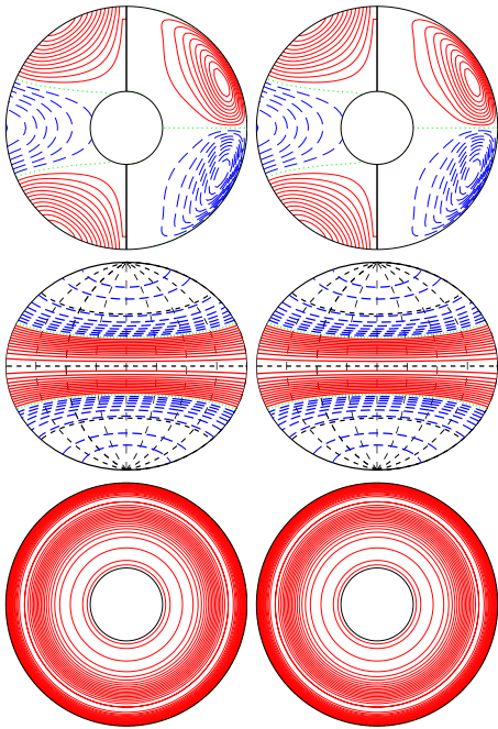
a.e03p01t03r-50000m1n2N2z6e4Y E_{kin}
