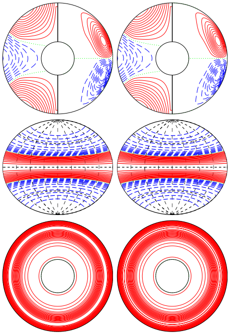
a.e03p01t03r-50000m1n2N2z10e4Y E_{\text{kin}}
