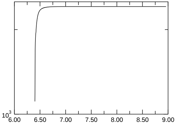
E_{kin,asymm.}
