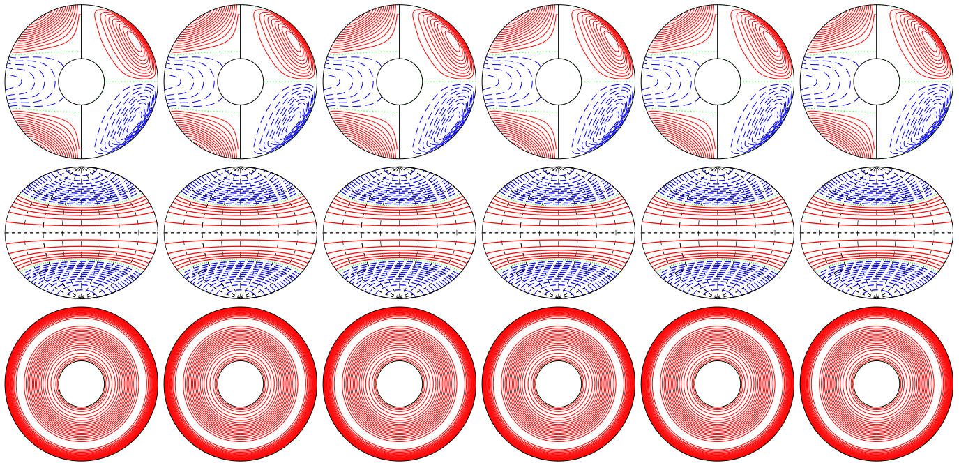
a.e03p05t03r-50000m1n2N2z4e2Y E_{\text{kin}}
