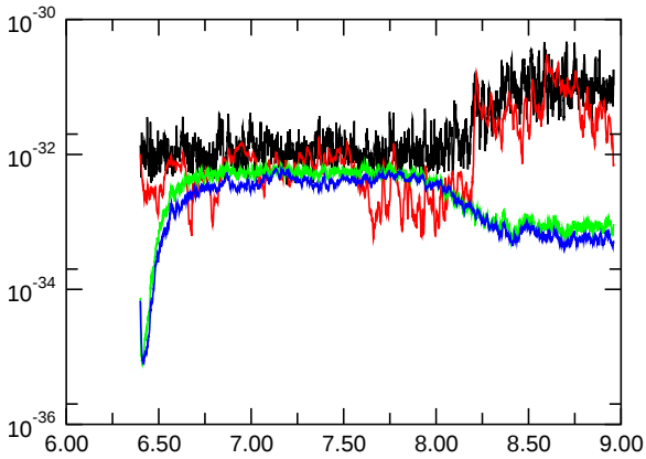
E_{kin,asymm.}
