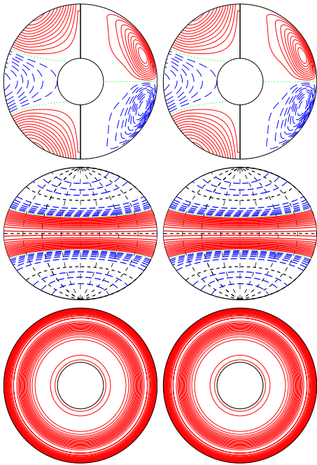
a.e03p01t03r-50000m1n2N2z8e4Y E_{\text{kin}}
