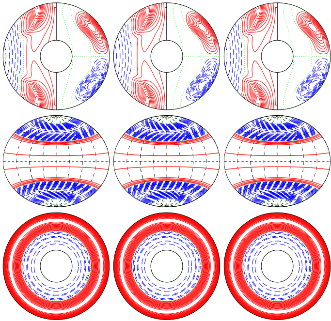
a.e03p01t03r-50000m1n2N2z20e4Y E_{kin}
