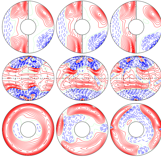
a.e03p01t03r-50000m1n2N2z60e4Y E_{\text{kin}}
