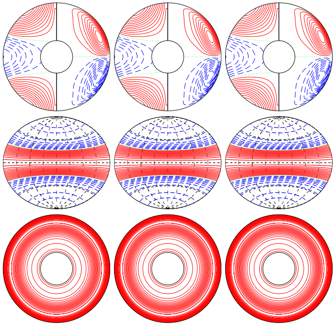
a.e03p01t03r-50000m1n2N2z6e4Y E_{\text{kin}}
