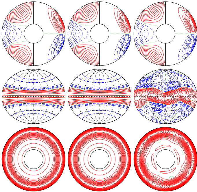
a.e03p01t03r-50000m1n2N2z10e4Y E_{\text{kin}}
