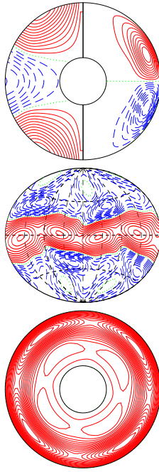
a.e03p01t03r-50000m1n2N2z9.5e4a E_{\text{kin}}
