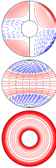
a.e03p1t03r-10000m1n2N2z5.0e3Y E_{\text{kin}}
