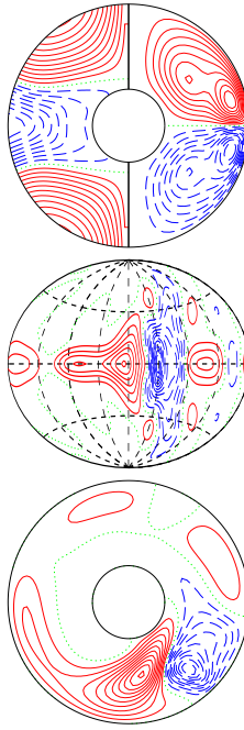
a.e03p1t03r-50000m1n2N1z6.0e4Y E_{\text{kin}}
