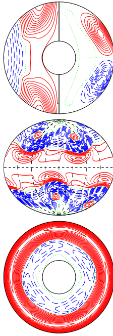
a.e03p01t03r-50000m1n2N2z20e4b E_{kin}
