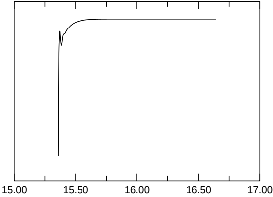
E_{kin,asymm.}
