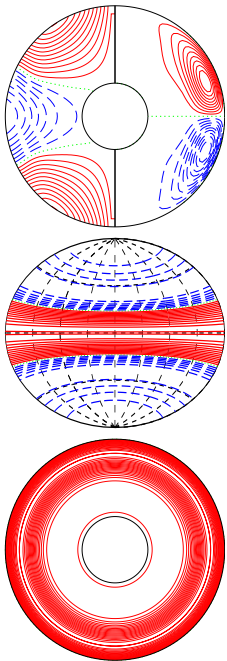
a.e03p01t03r-50000m1n2N2z9.5e4b E_{\text{kin}}
