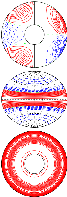
a.e03p01t03r-50000m1n2N2z8.5e4b E_{kin}
