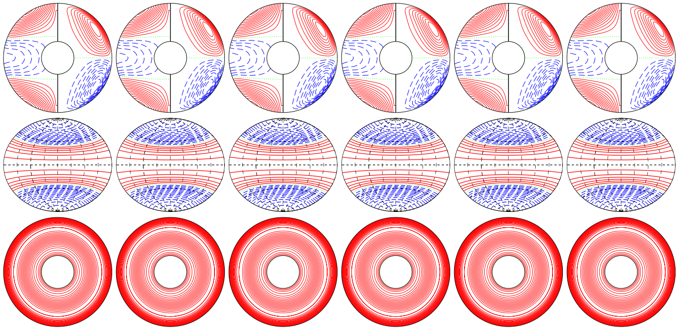
a.e03p01t03r-50000m1n2N2z4e2Y E_{\text{kin}}
