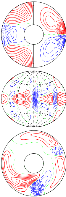
a.e03p1t03r-50000m1n2N1.5z6.0e4Y E_{\text{kin}}
