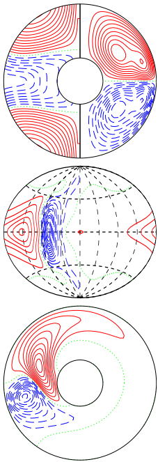
a.e03p1t03r-50000m1n2N0.5z6.0e4Y E_{kin}
