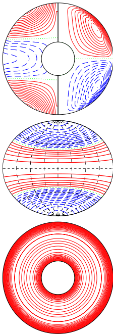
a.e03p1t03r-10000m1n2N2z7.0e3Y E_{kin}
