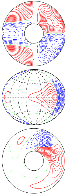
a.e03p1t03r-50000m1n2N0.1z6.0e4Y E_{\text{kin}}
