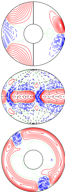
a.e03p1t03r-50000m1n2N3z6.0e4Y E_{kin}
