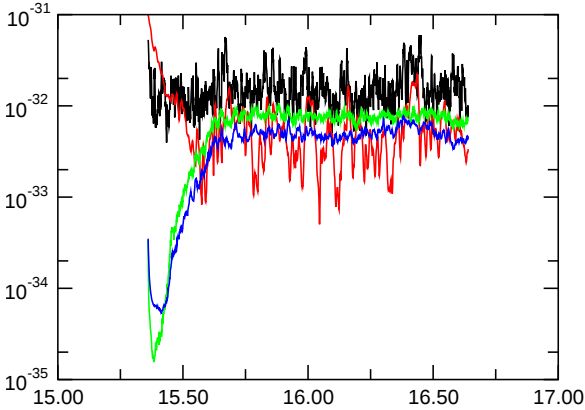
E_{kin,asymm.}
