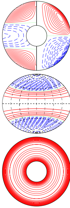
a.e03p1t03r-10000m1n2N2z3.0e3Y E_{\text{kin}}
