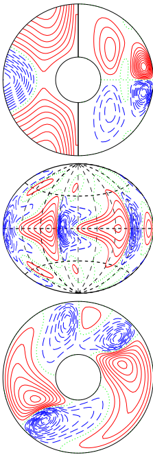
a.e03p1t03r-10000m1n2N2z2.5e4Yb E_{\text{kin}}
