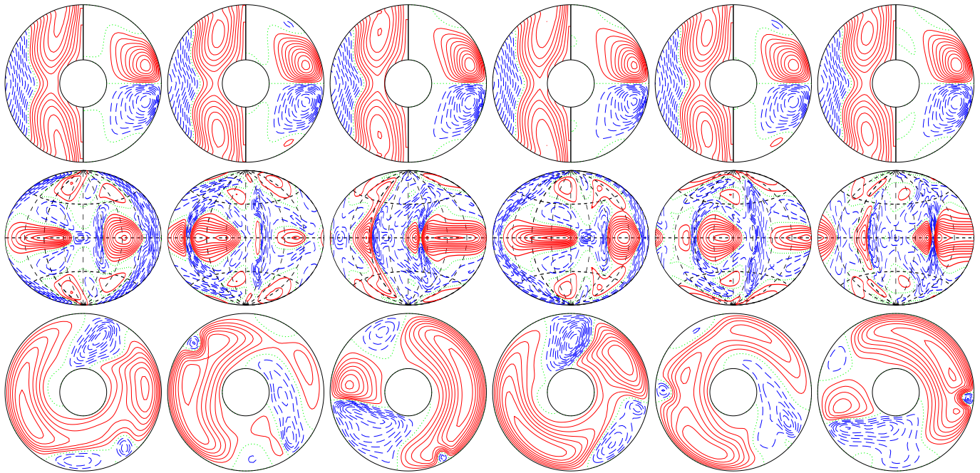
a.e03p1t03r-10000m1n2N2z5.0e4Y E_{kin}
