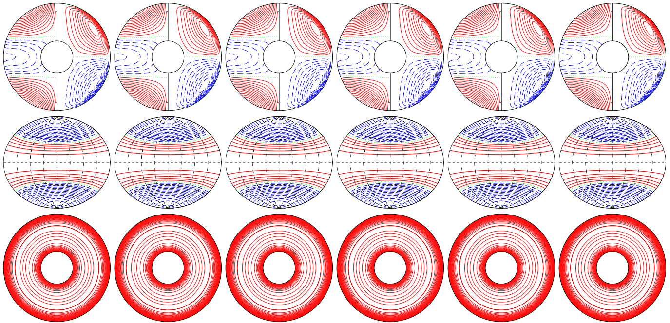
a.e03p1t03r-10000m1n2N2z3.0e3Y E_{\text{kin}}
