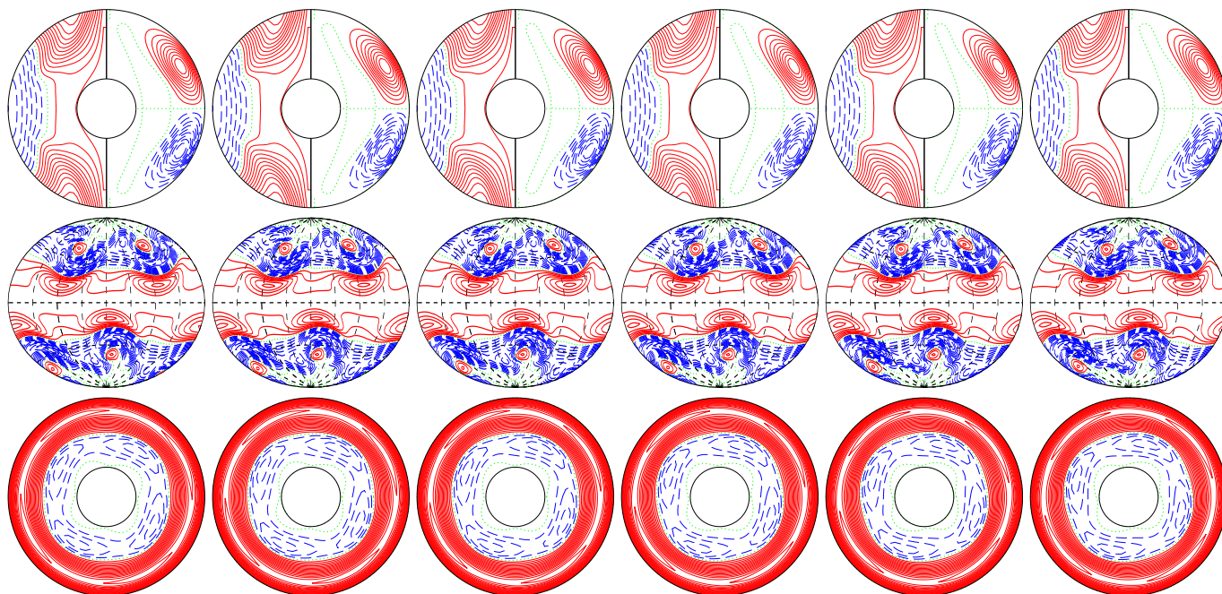
a.e03p01t03r-50000m1n2N2z20e4b E_{\text{kin}}
