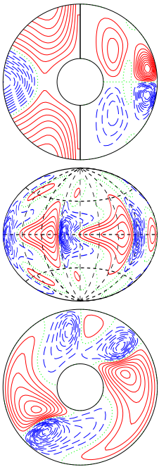
a.e03p1t03r-10000m1n2N2z2.5e4Yb E_{\text{kin}}
