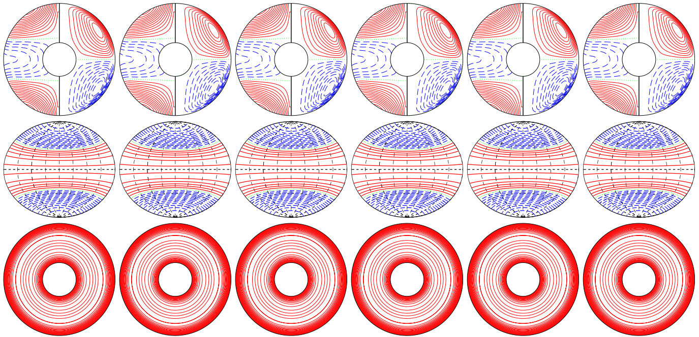
a.e03p1t03r-10000m1n2N2z5.0e3Y E_{kin}
