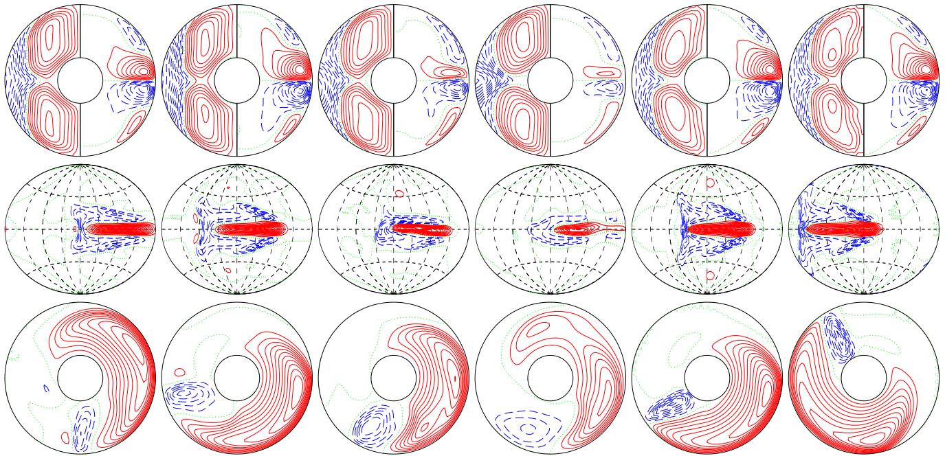
a.e03p5t03r-50000m1n2N2z6e4Y E_{\text{kin}}
