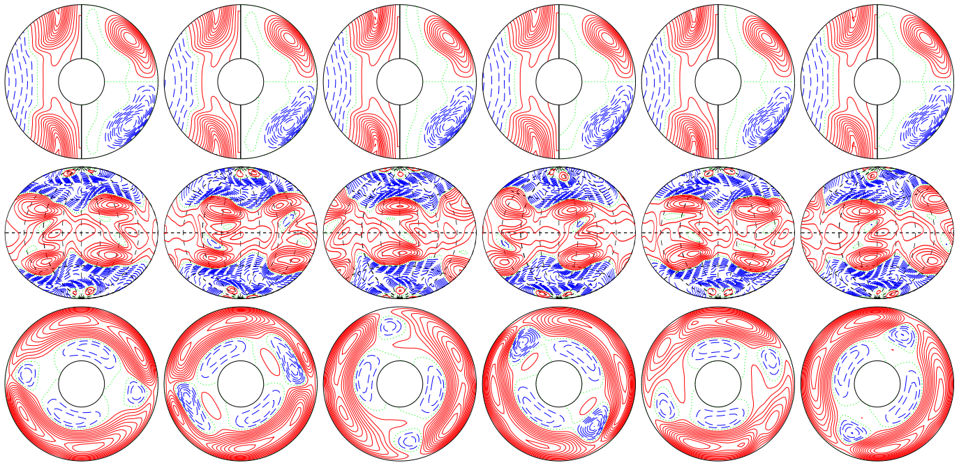
a.e03p01t03r-50000m1n2N2z35e4b E_{\text{kin}}
