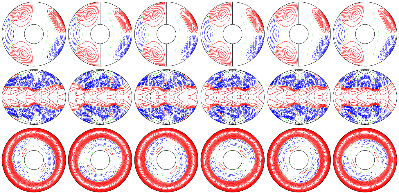
a.e03p01t03r-50000m1n2N2z15e4b E_{\text{kin}}
