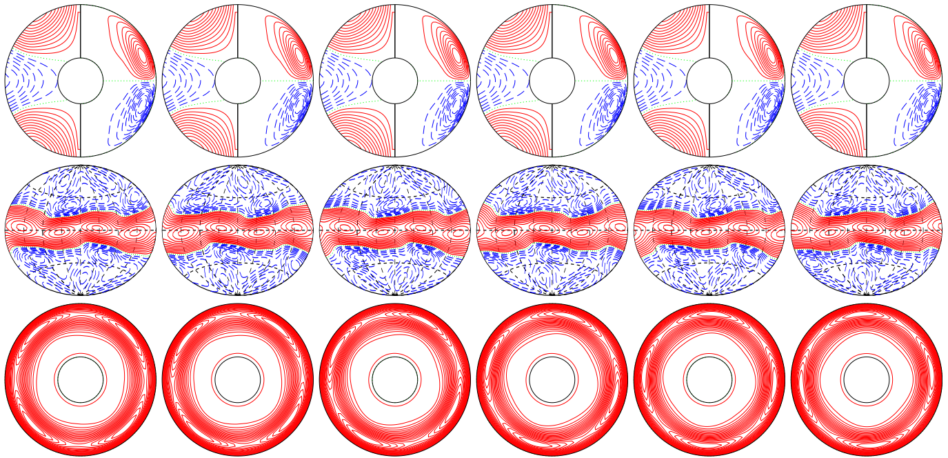
a.e03p01t03r-50000m1n2N2z8.5e4b E_{\text{kin}}
