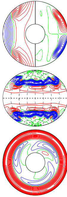
a.e03p01t1r-100000m1n1.5N3z5e5 E_{kin}
