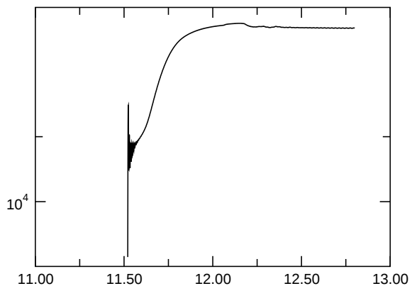
E_{kin,asymm.}
