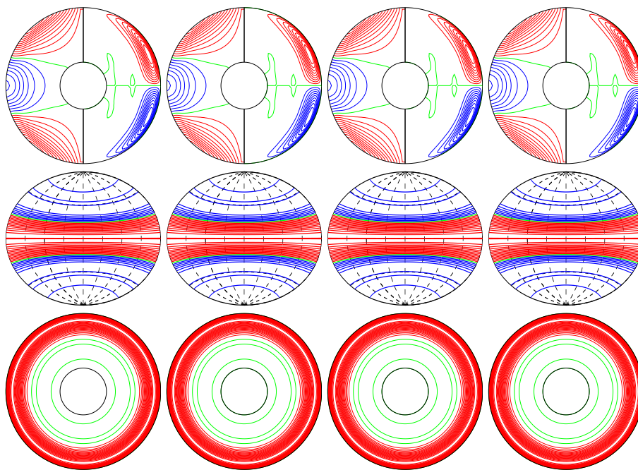
a.e03p01t1r-100000m1n1.5N3z2e5 E_{\text{kin}}
