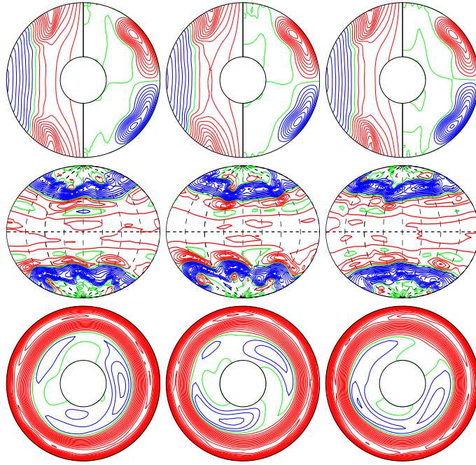
a.e03p01t1r-100000m1n1.5N3z7e5 E_{\text{kin}}
