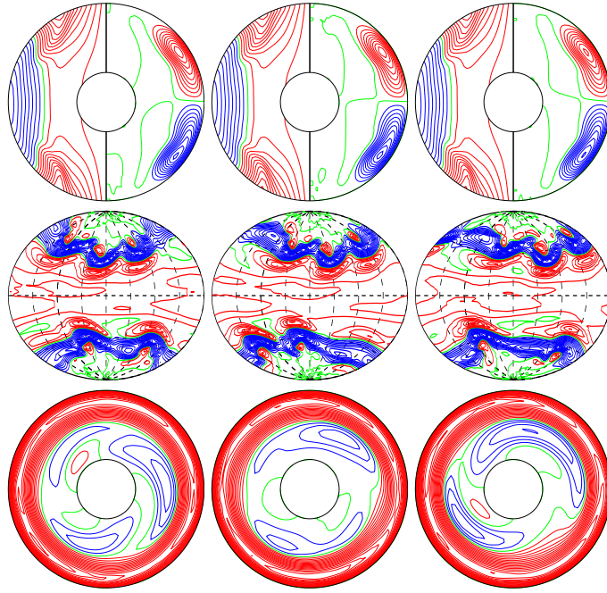
a.e03p01t1r-100000m1n1.5N3z6e5 E_{\text{kin}}
