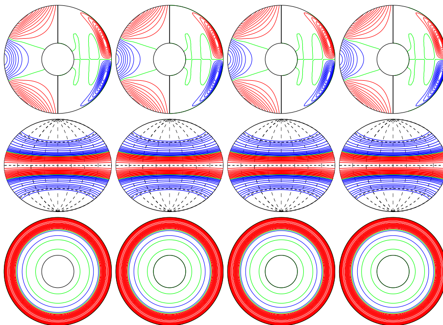
a.e03p01t1r-100000m1n1.5N3z4e5 E_{\text{kin}}
