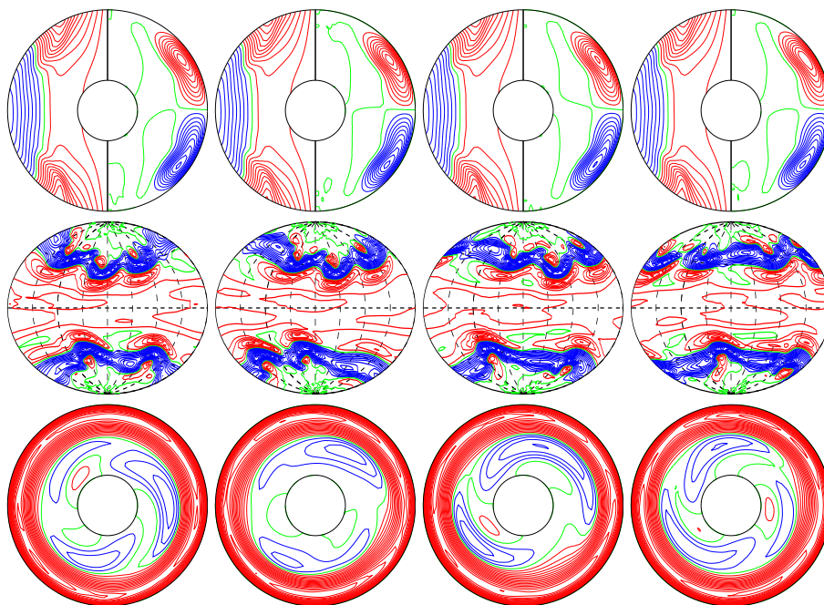
a.e03p01t1r-100000m1n1.5N3z6e5 E_{\text{kin}}
