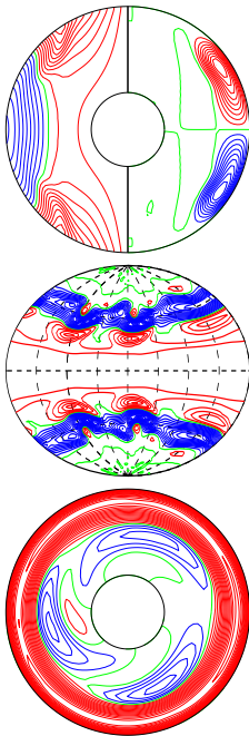
a.e03p01t1r-100000m1n1.5N3z4.8e5 E_{\text{kin}}
