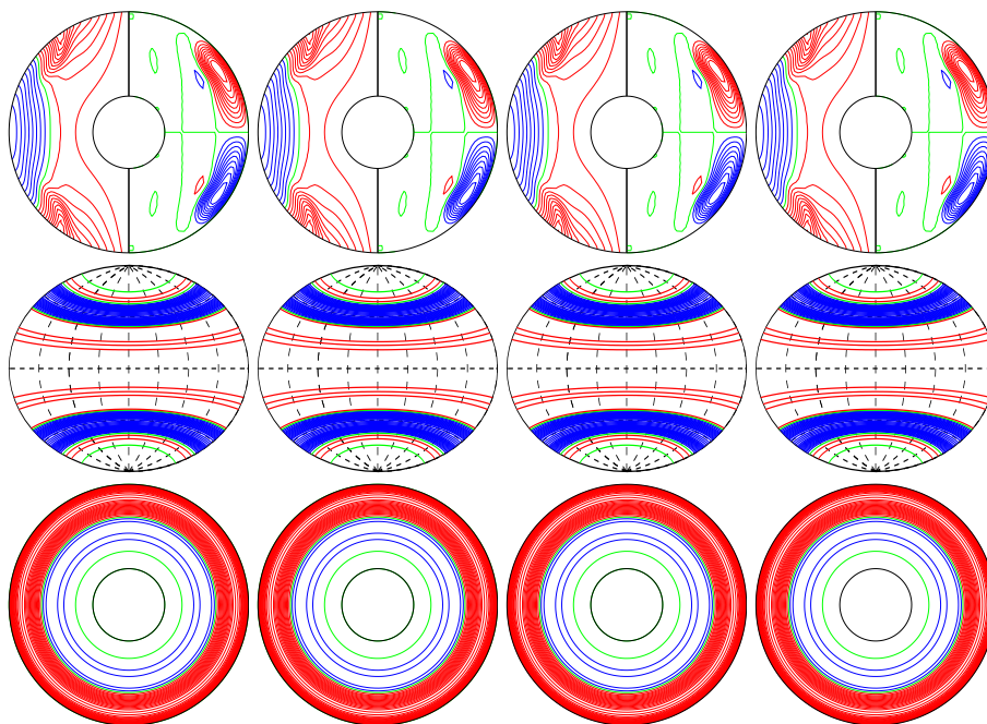
a.e03p01t1r-100000m1n1.5N3z4.5e5 E_{\text{kin}}
