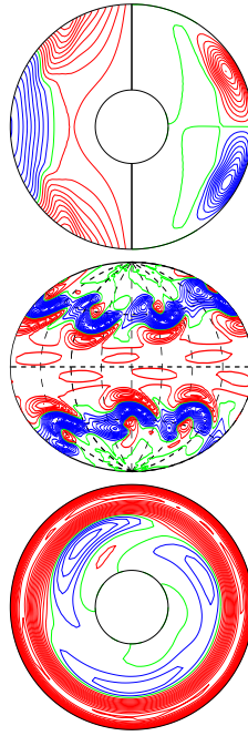
a.e03p01t1r-100000m1n1.5N3z5.3e5 E_{\text{kin}}
