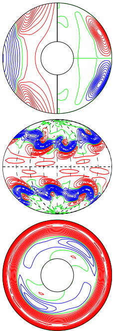
a.e03p01t1r-100000m1n1.5N3z5.4e5 E_{\text{kin}}
