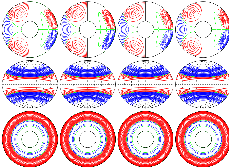
a.e03p01t03r-50000m1n2N2z12e4 E_{\text{kin}}
