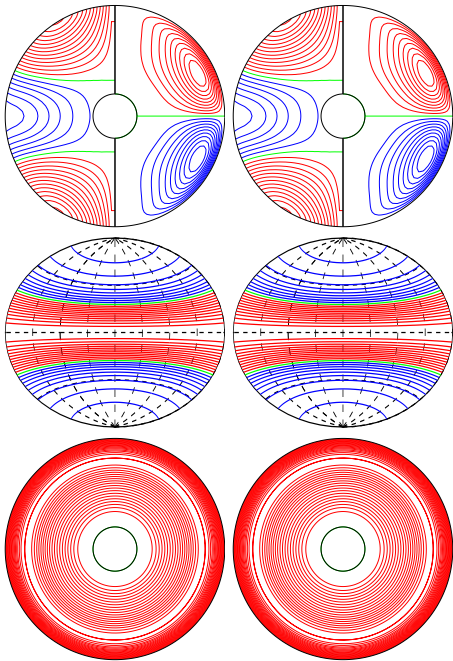
a.e02p001t03r-50000m1n2N2z9e4 E_{\text{kin}}
