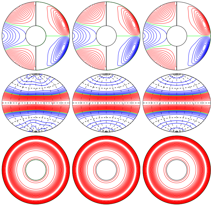
a.e03p01t03r-50000m1n2N2z7.5e4Y E_{\text{kin}}
