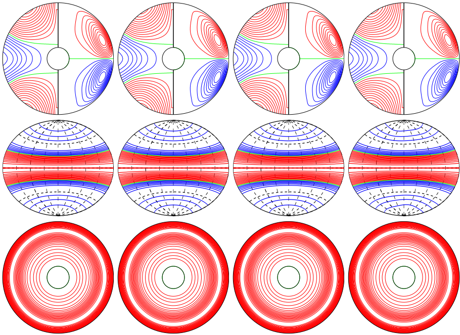
a.e02p001t03r-50000m1n2N2z15e4 E_{\text{kin}}
