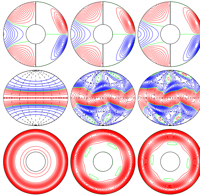
a.e03p01t03r-50000m1n2N2z10.4e4 E_{\text{kin}}
