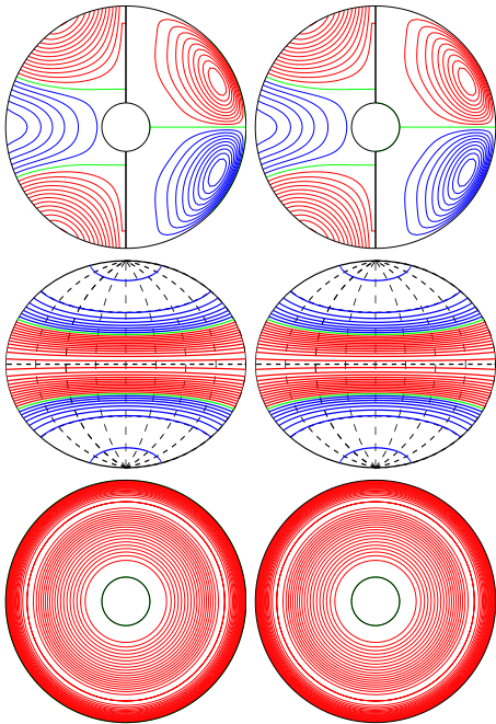
a.e02p001t03r-50000m1n2N2z1e5 E_{\text{kin}}
