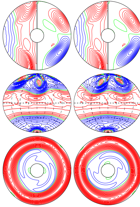
a.e02p001t03r-50000m1n2N2z8e5 E_{\text{kin}}
