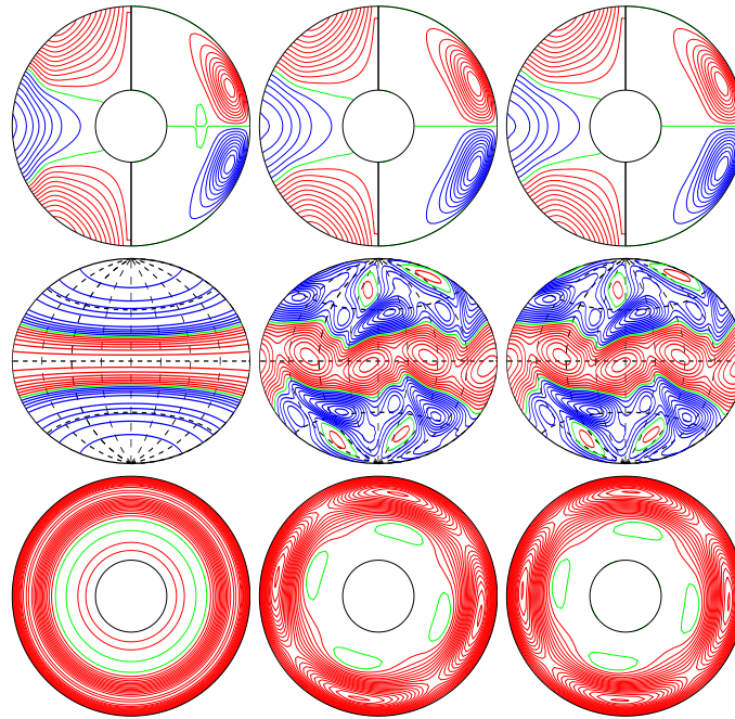
a.e03p01t03r-50000m1n2N2z11e4 E_{\text{kin}}
