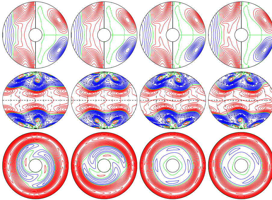
a.e02p005t03r-50000m1n2N2z50e4 E_{\text{kin}}
