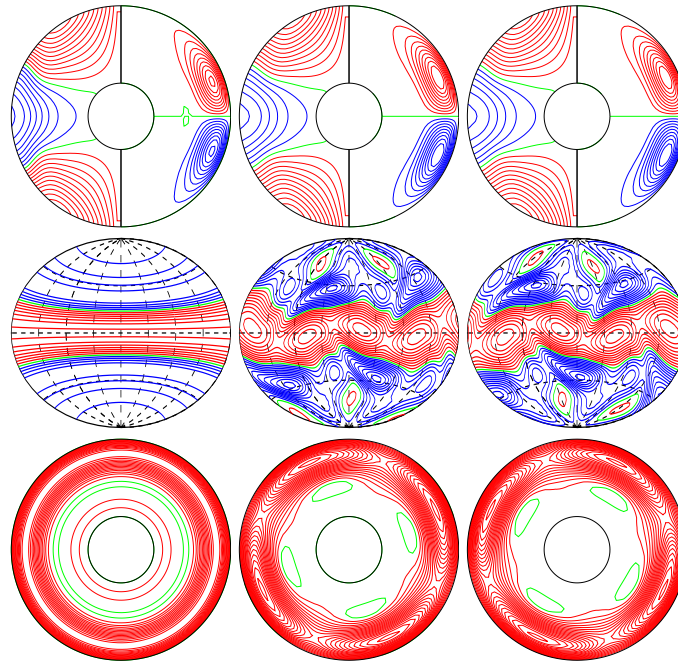
a.e03p01t03r-50000m1n2N2z10.8e4 E_{\text{kin}}
