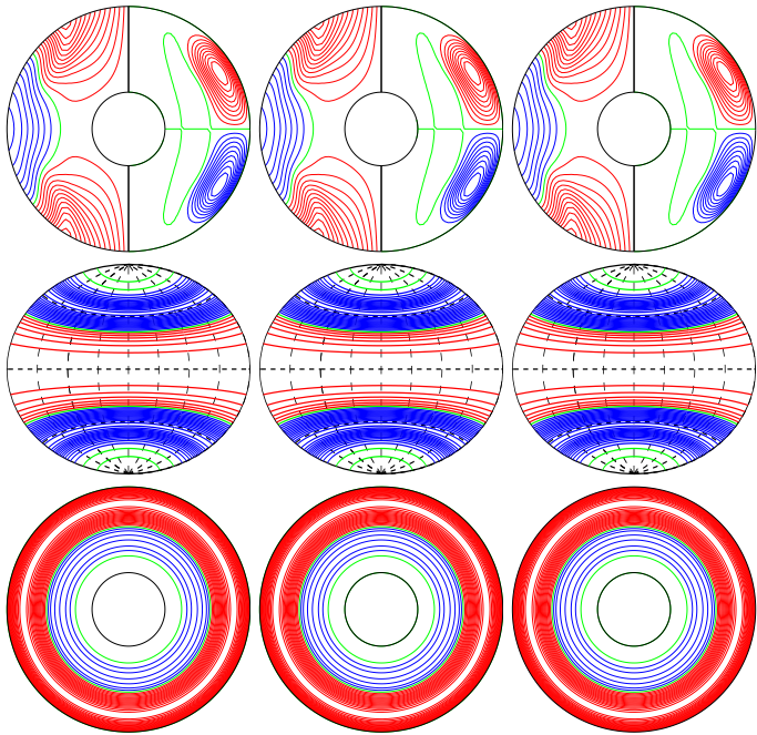
a.e03p01t03r-50000m1n2N2z13e4 E_{\text{kin}}
