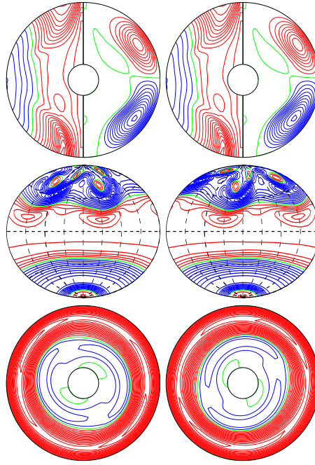
a.e02p001t03r-50000m1n2N2z6e5 E_{\text{kin}}
