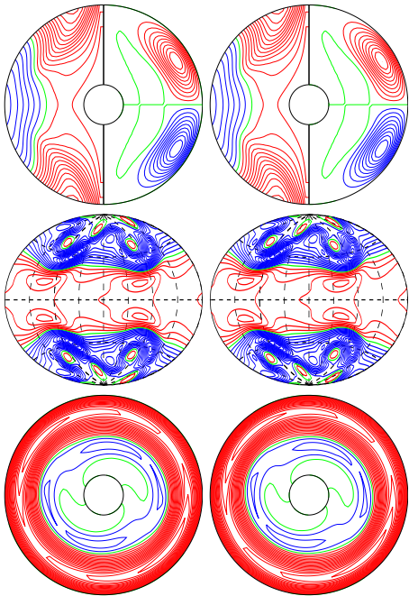
a.e02p001t03r-50000m1n2N2z4e5 E_{\text{kin}}
