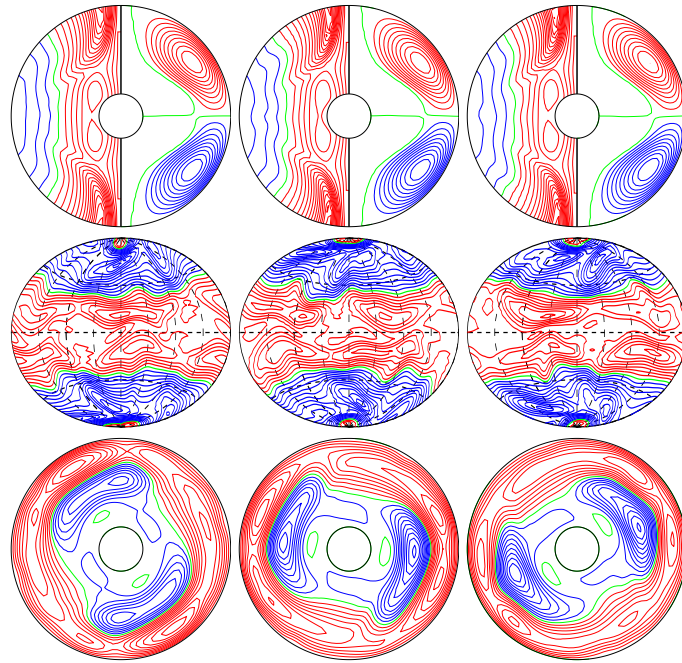
a.e02p001t03r-50000m1n2N2z1.5e6 E_{\text{kin}}
