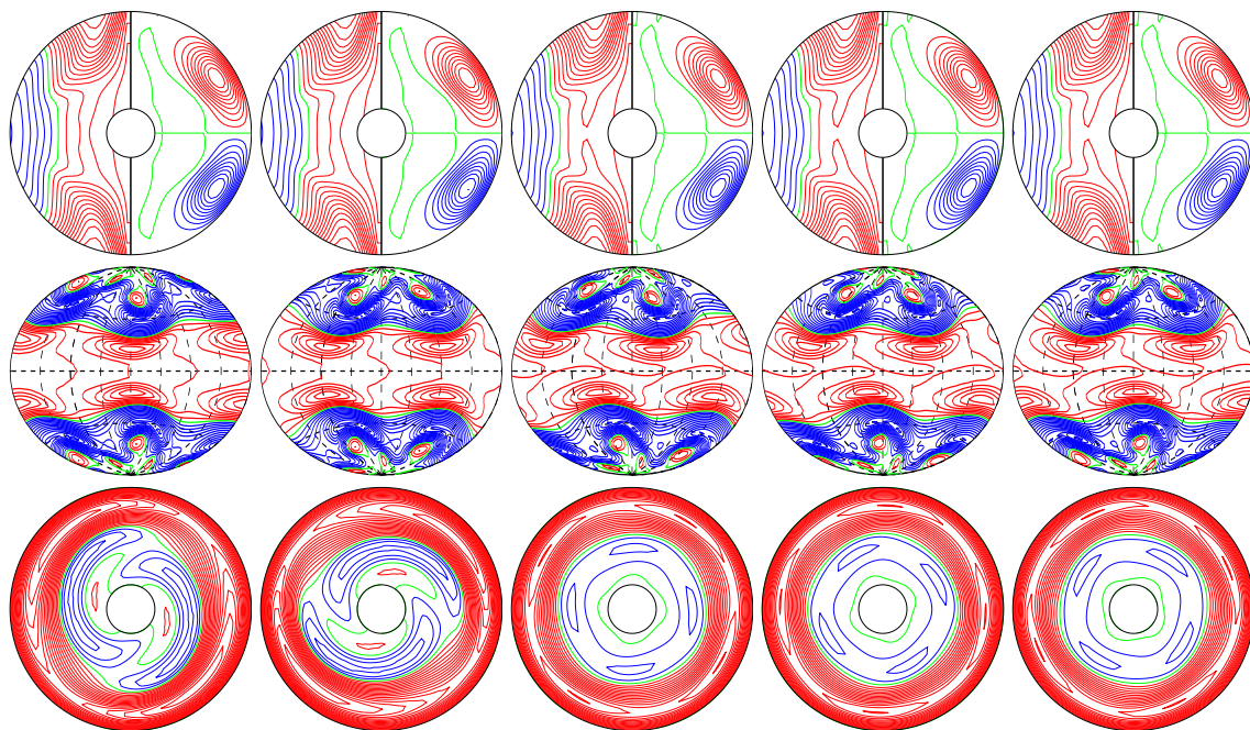
a.e02p005t03r-50000m1n2N2z50e4 E_{\text{kin}}
