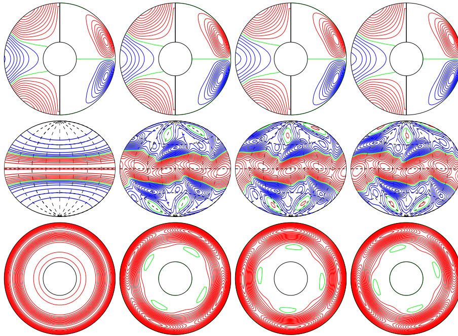
a.e03p01t03r-50000m1n2N2z10.4e4 E_{\text{kin}}
