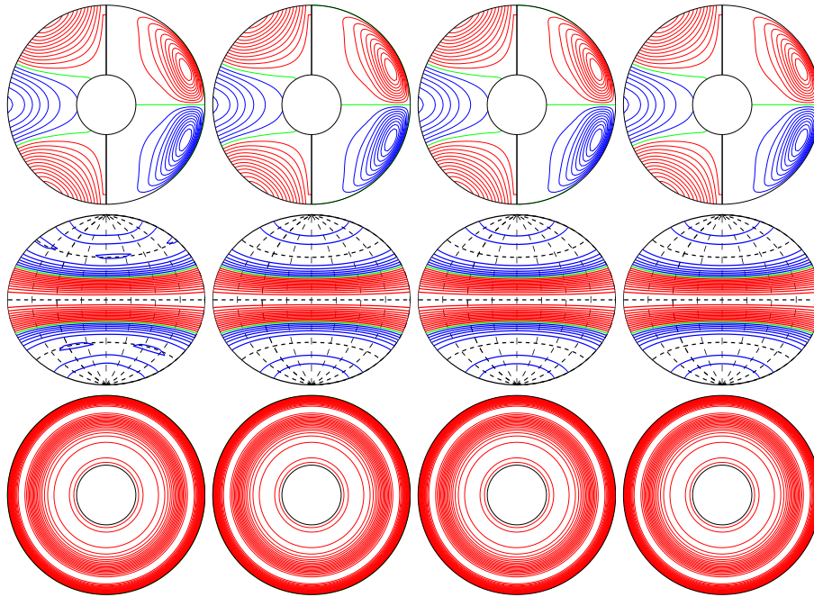
a.e03p01t03r-50000m1n2N2z7e4Y E_{\text{kin}}
