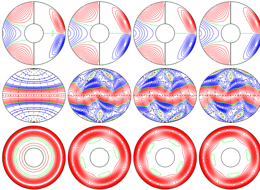
a.e03p01t03r-50000m1n2N2z10.8e4 E_{\text{kin}}
