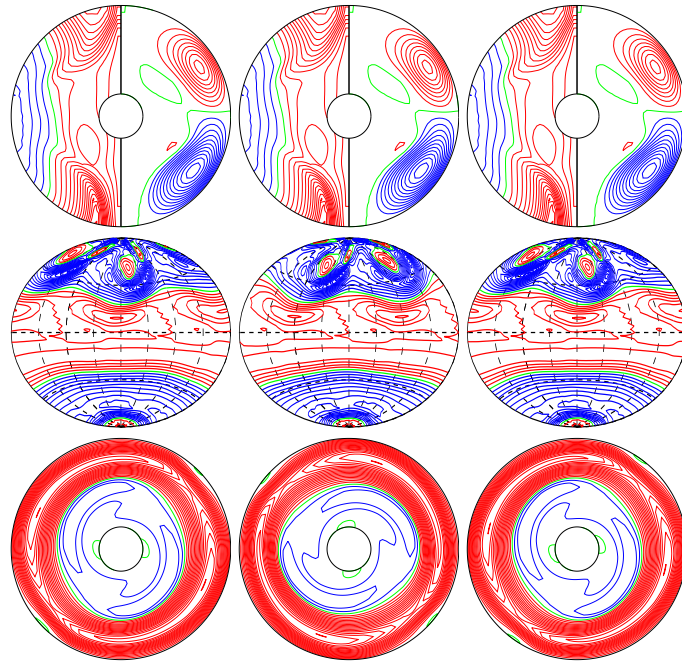
a.e02p001t03r-50000m1n2N2z8e5 E_{\text{kin}}
