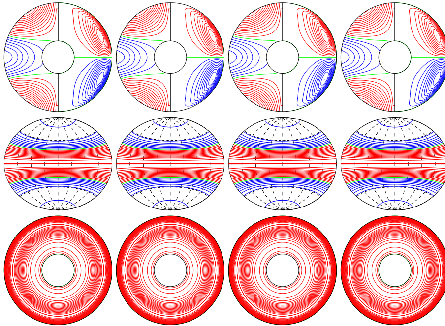
a.e03p01t03r-50000m1n2N2z5e4Y E_{\text{kin}}
