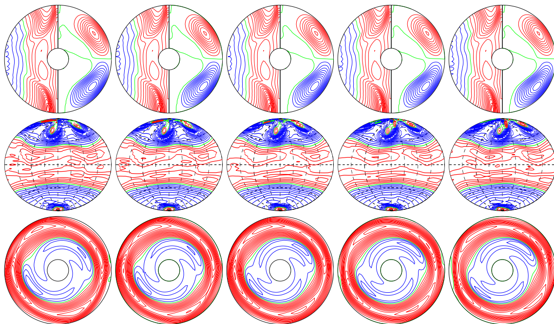
a.e02p001t03r-50000m1n2N2z1e6 E_{\text{kin}}
