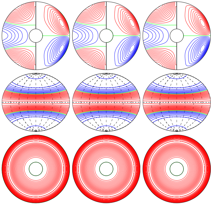
a.e02p001t03r-50000m1n2N2z1e5 E_{\text{kin}}
