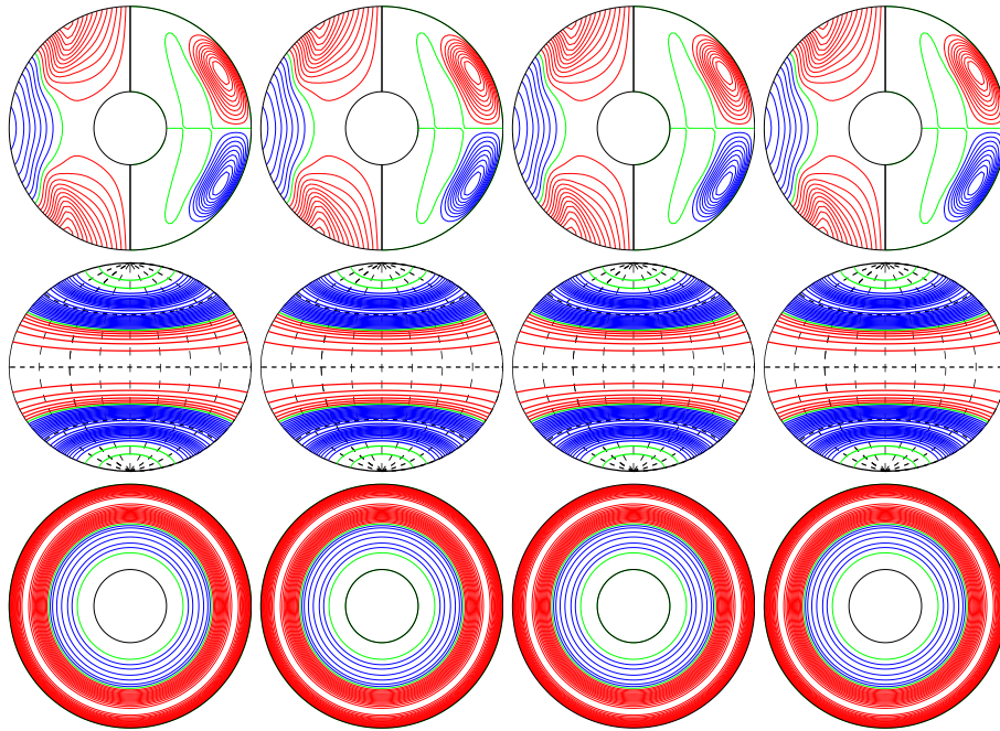
a.e03p01t03r-50000m1n2N2z13e4 E_{\text{kin}}
