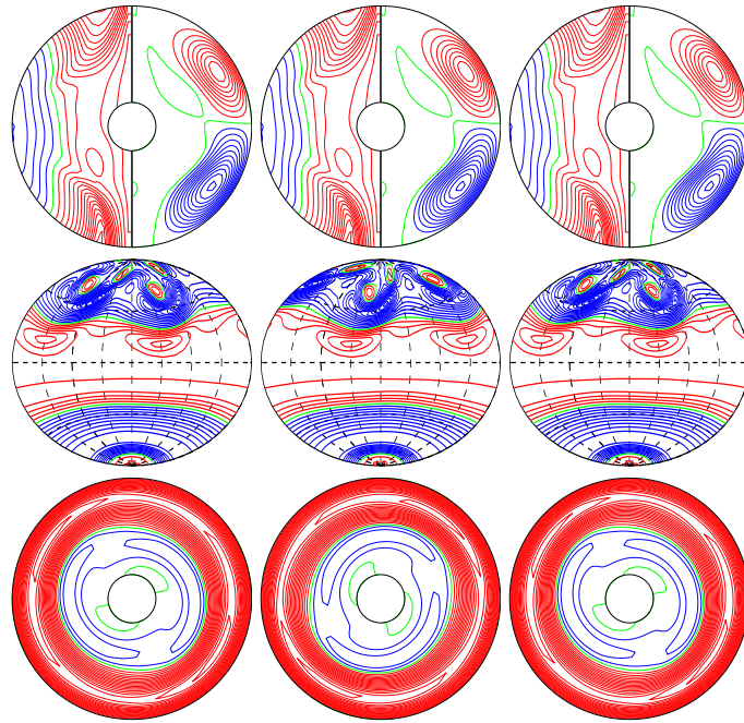
a.e02p001t03r-50000m1n2N2z6e5 E_{\text{kin}}
