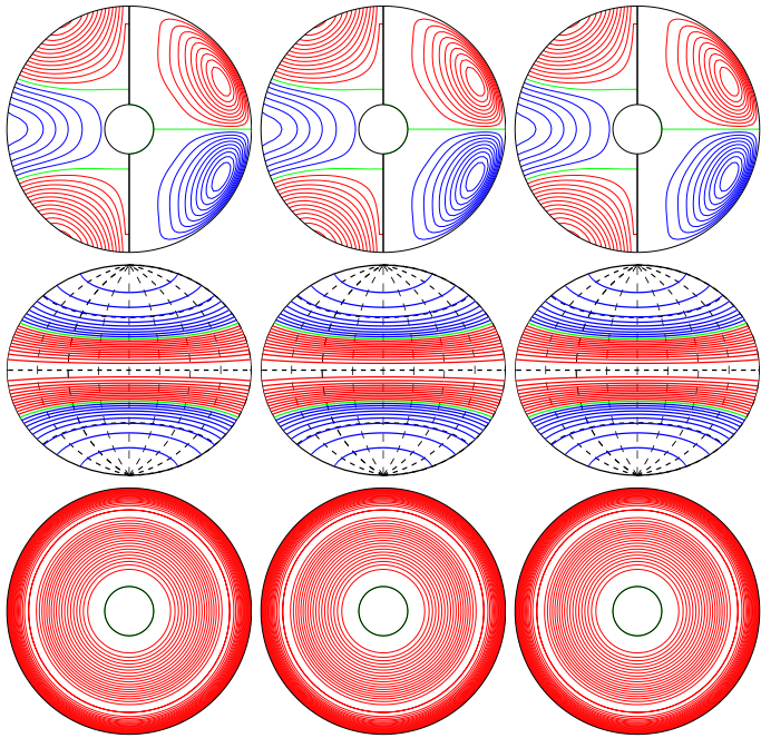
a.e02p001t03r-50000m1n2N2z9e4 E_{\text{kin}}
