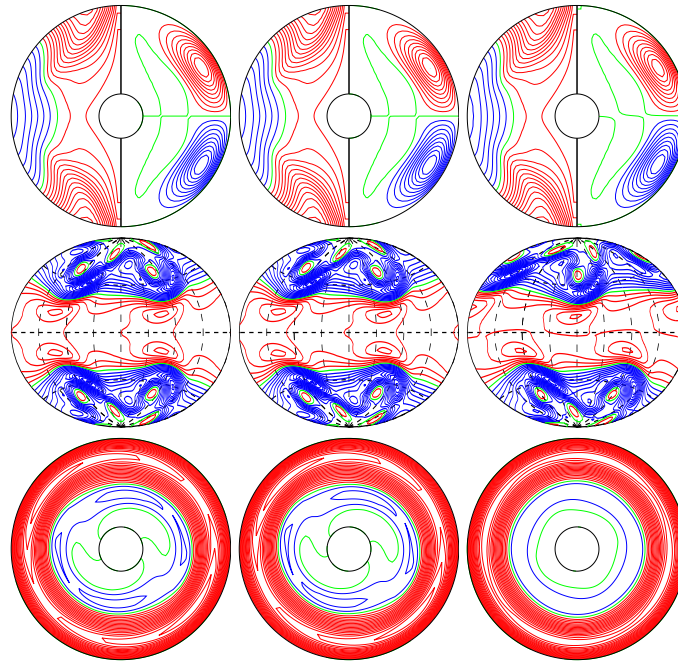
a.e02p001t03r-50000m1n2N2z4e5 E_{\text{kin}}
