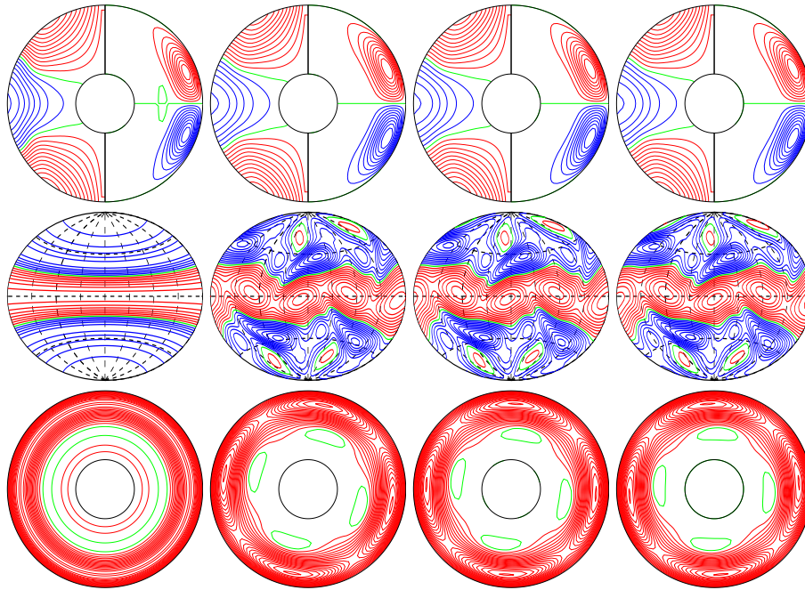
a.e03p01t03r-50000m1n2N2z11e4 E_{\text{kin}}
