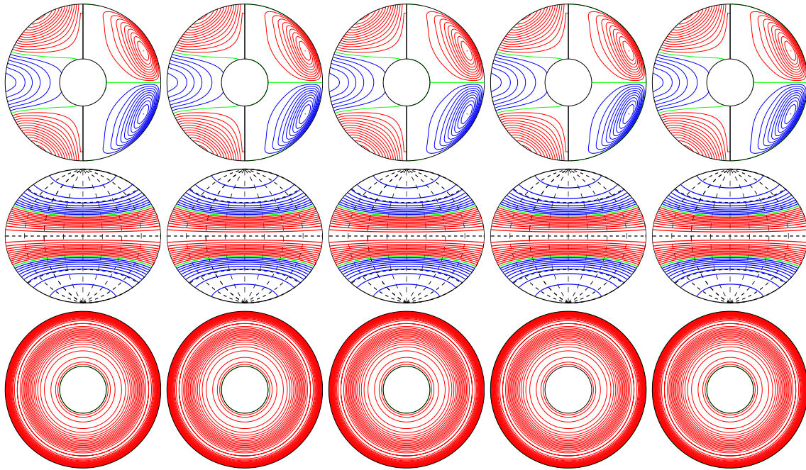
a.e03p01t03r-50000m1n2N2z4.5e4Y E_{\text{kin}}
