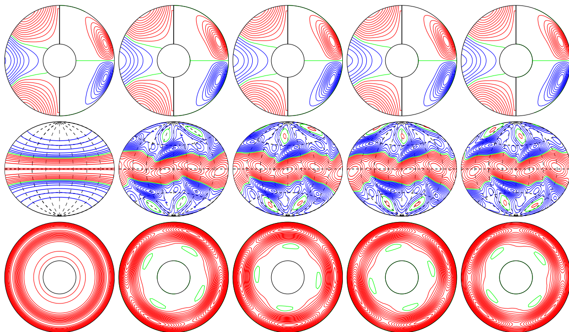
a.e03p01t03r-50000m1n2N2z10.4e4 E_{\text{kin}}
