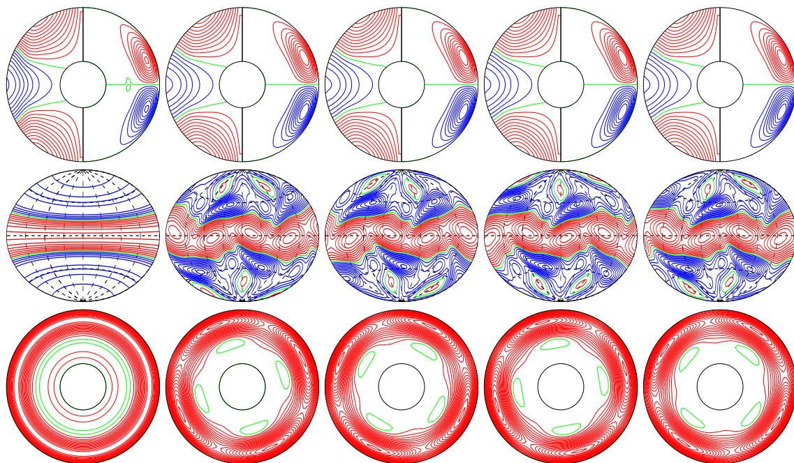
a.e03p01t03r-50000m1n2N2z10.8e4 E_{\text{kin}}
