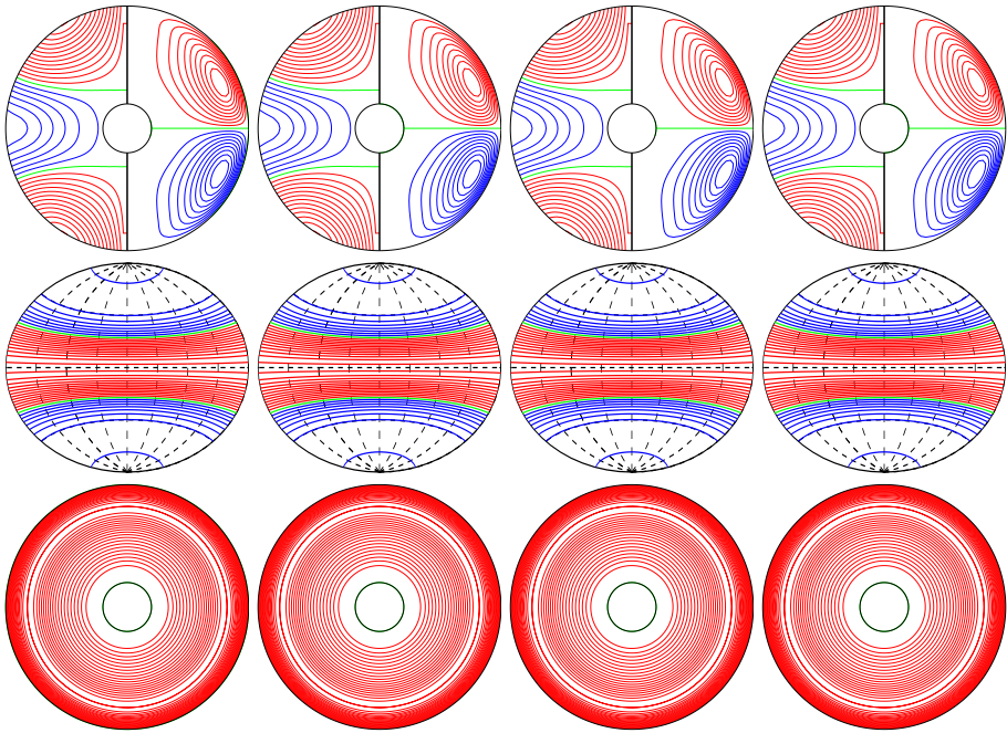
a.e02p001t03r-50000m1n2N2z1e5 E_{\text{kin}}
