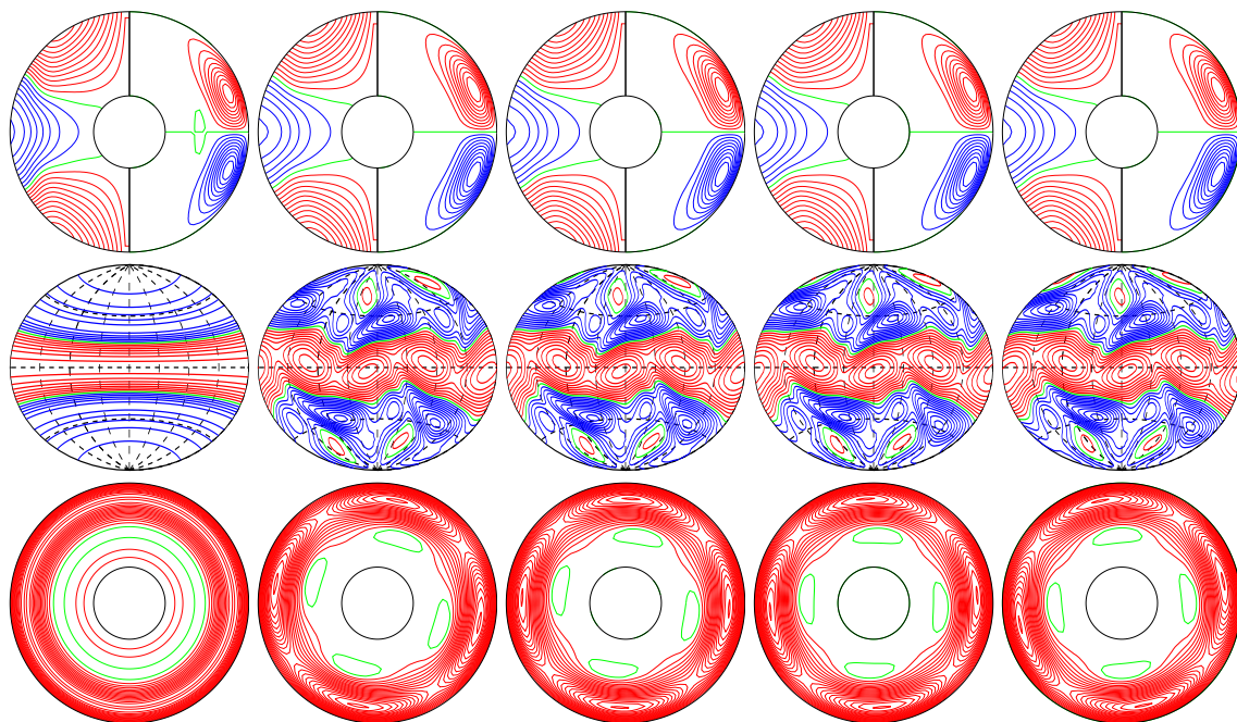
a.e03p01t03r-50000m1n2N2z11e4 E_{\text{kin}}
