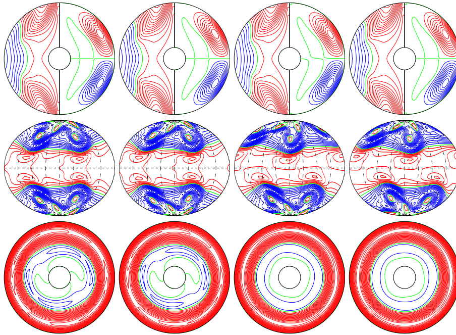
a.e02p001t03r-50000m1n2N2z4e5 E_{\text{kin}}
