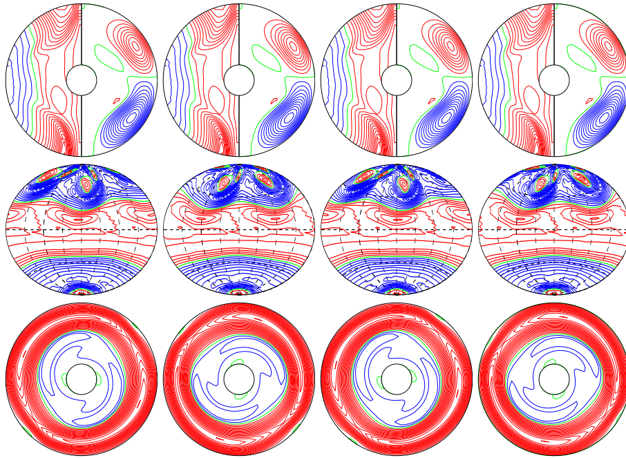
a.e02p001t03r-50000m1n2N2z8e5 E_{\text{kin}}
