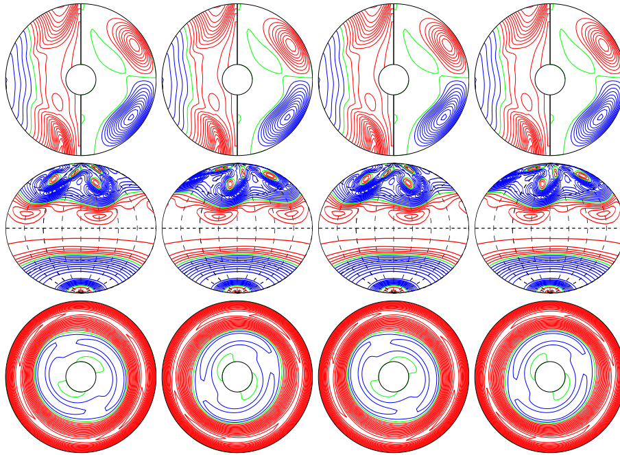
a.e02p001t03r-50000m1n2N2z6e5 E_{\text{kin}}
