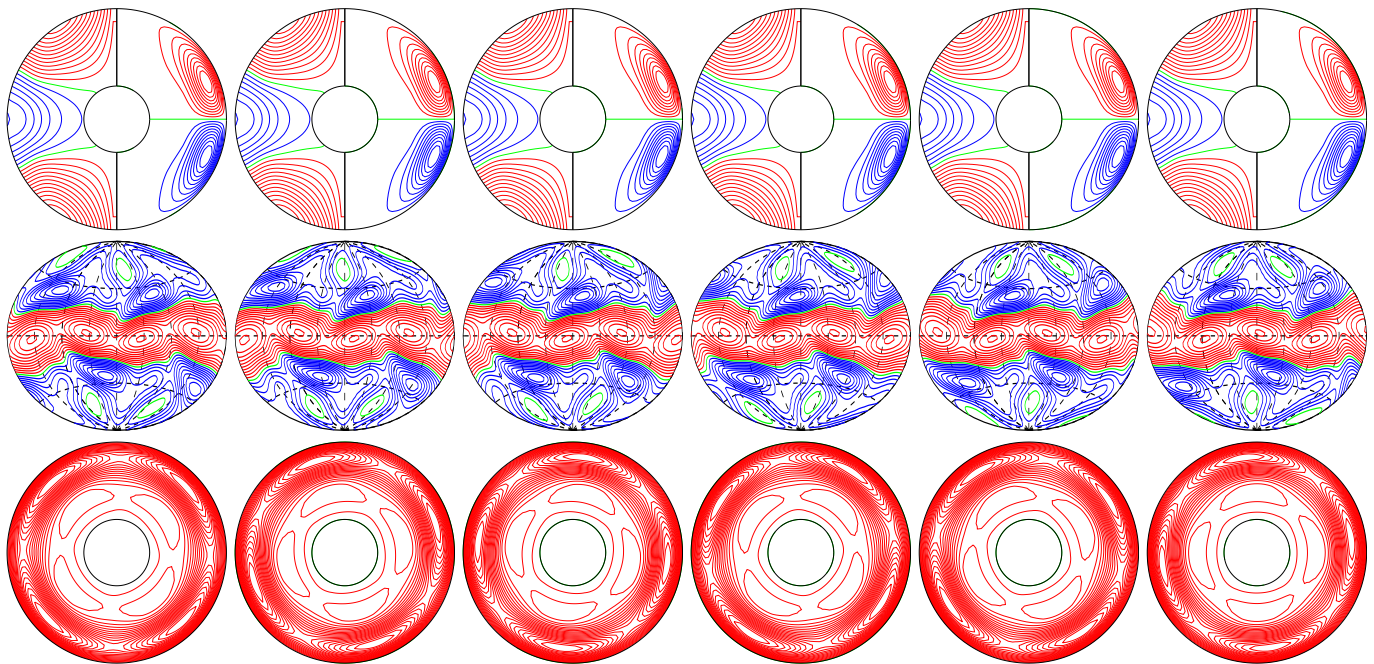
a.e03p01t03r-50000m1n2N2z9.5e4b E_{\text{kin}}
