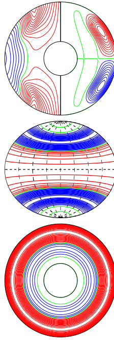
a.e03p01t03r-50000m1n2N2z14e4b E_{\text{kin}}
