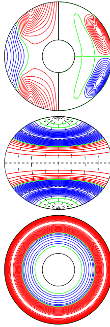
a.e03p01t03r-50000m1n2N2z13e4a E_{\text{kin}}
