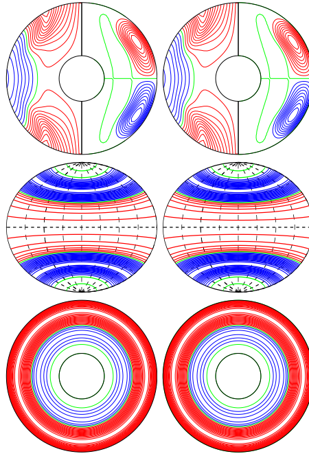
a.e03p01t03r-50000m1n2N2z14e4b E_{\text{kin}}
