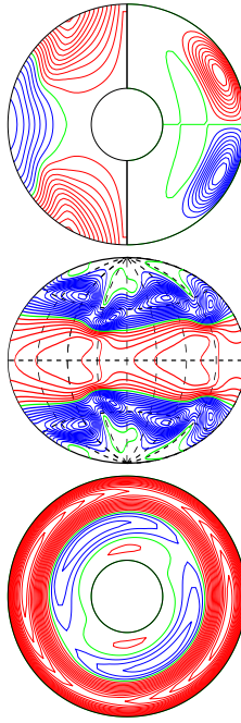
a.e03p01t03r-50000m1n2N2z13.5e4a E_{\text{kin}}
