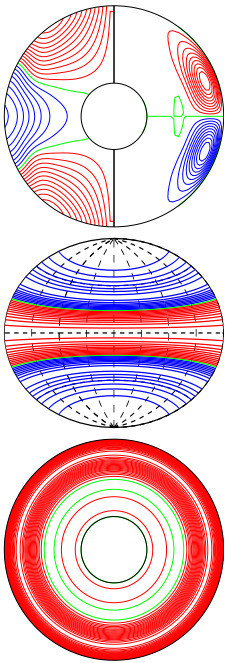
a.e03p01t03r-50000m1n2N2z11e4a E_{\text{kin}}
