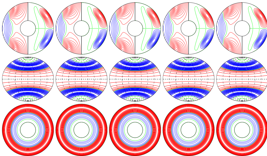
a.e03p01t03r-50000m1n2N2z14e4b E_{\text{kin}}
