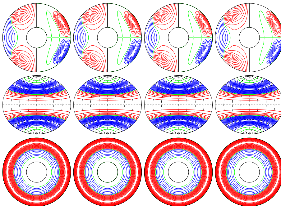
a.e03p01t03r-50000m1n2N2z13e4a E_{\text{kin}}
