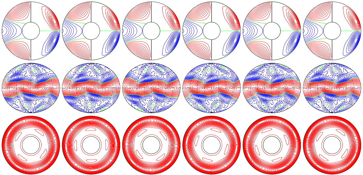
a.e03p01t03r-50000m1n2N2z9e4b E_{\text{kin}}
