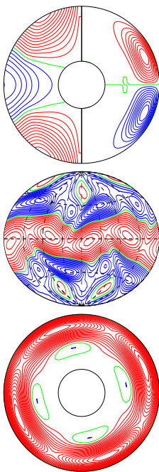
a.e03p01t03r-50000m1n2N2z11.5e4 E_{\text{kin}}
