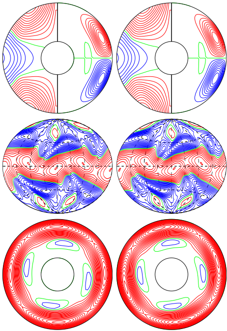
a.e03p01t03r-50000m1n2N2z12.5e4b E_{\text{kin}}
