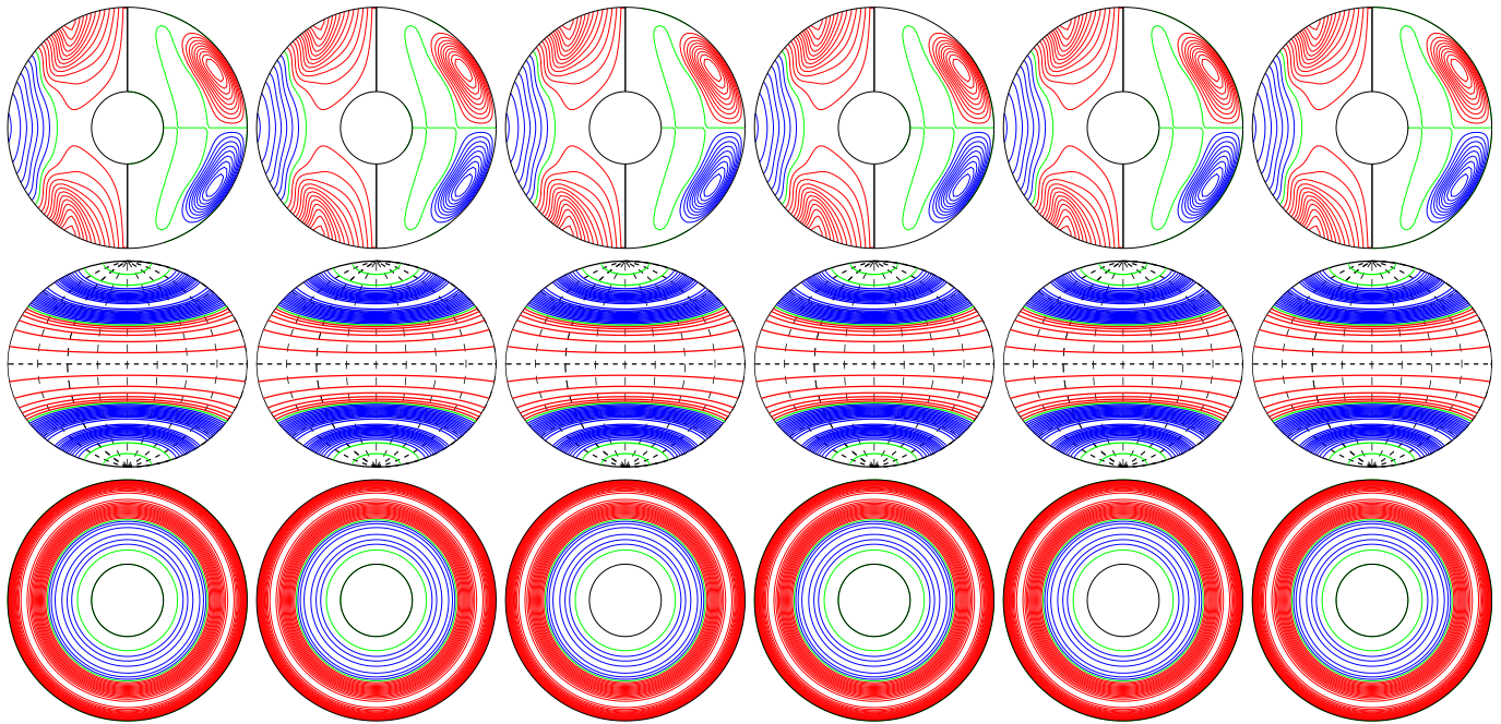
a.e03p01t03r-50000m1n2N2z14e4b E_{\text{kin}}
