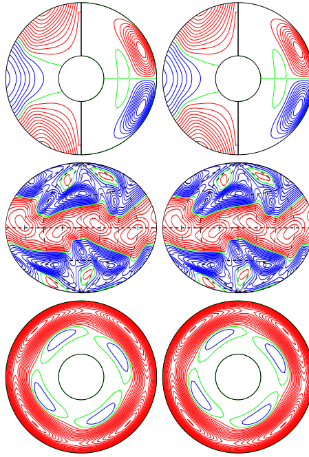
a.e03p01t03r-50000m1n2N2z13e4b E_{\text{kin}}
