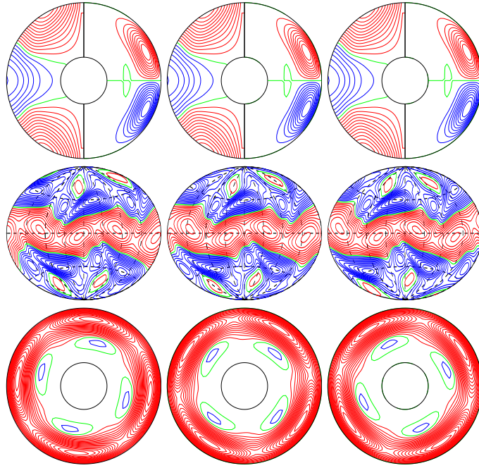
a.e03p01t03r-50000m1n2N2z12e4b E_{\text{kin}}
