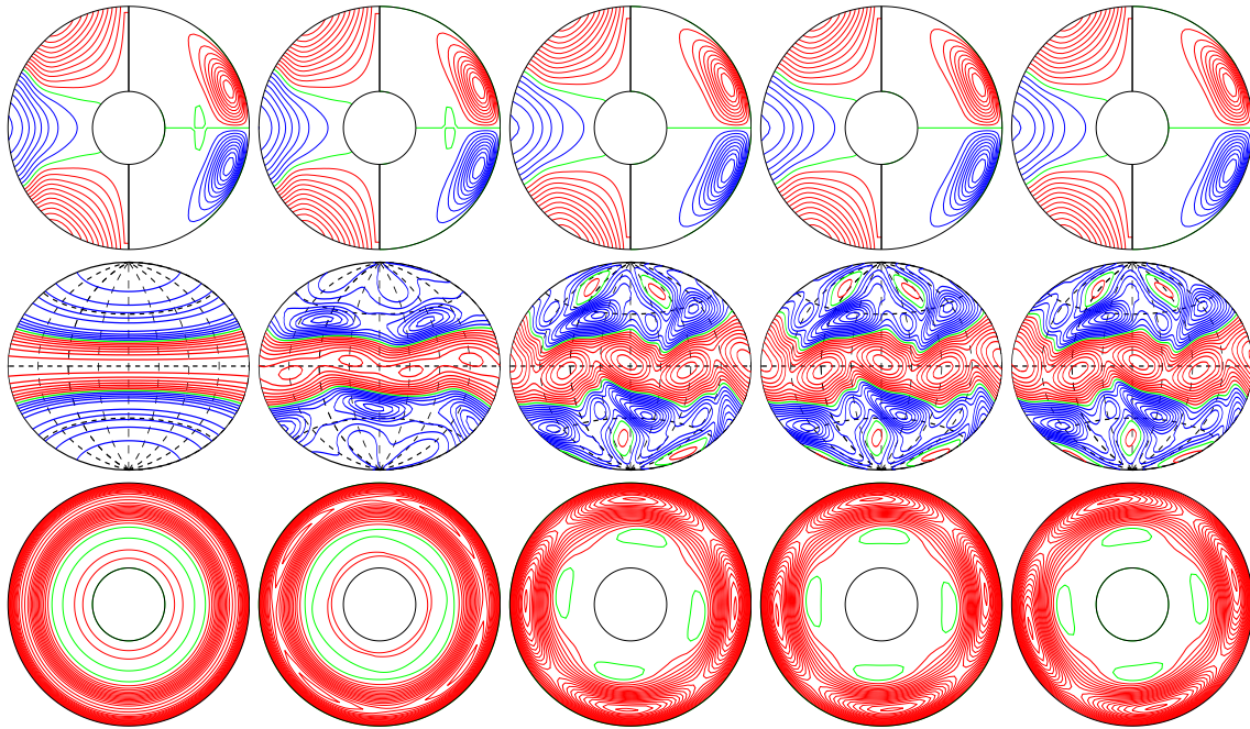
a.e03p01t03r-50000m1n2N2z11e4a E_{\text{kin}}
