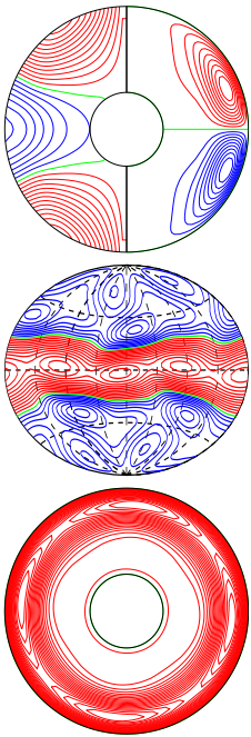
a.e03p01t03r-50000m1n2N2z8.4e4a E_{kin}
