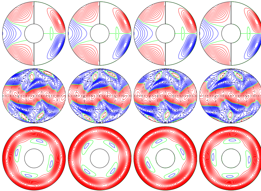
a.e03p01t03r-50000m1n2N2z12e4b E_{\text{kin}}
