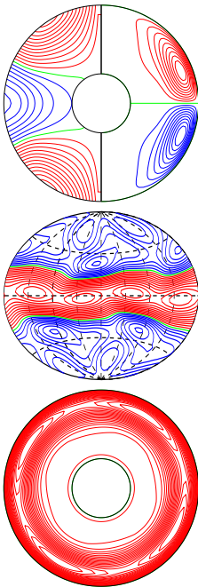
a.e03p01t03r-50000m1n2N2z8.3e4a E_{kin}
