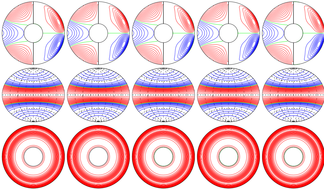
a.e03p01t03r-50000m16n2N2z8.5e4b E_{\text{kin}}
