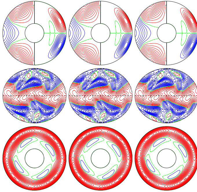
a.e03p01t03r-50000m1n2N2z13e4b E_{\text{kin}}
