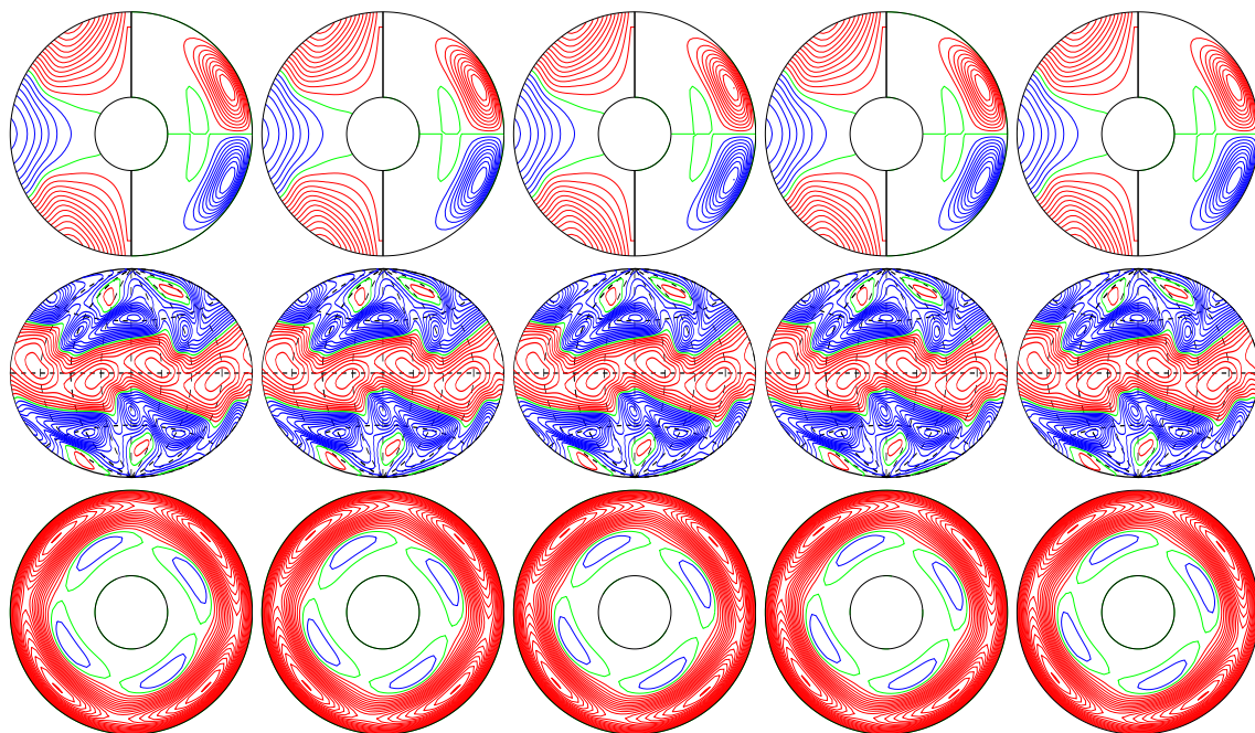
a.e03p01t03r-50000m1n2N2z13e4b E_{\text{kin}}
