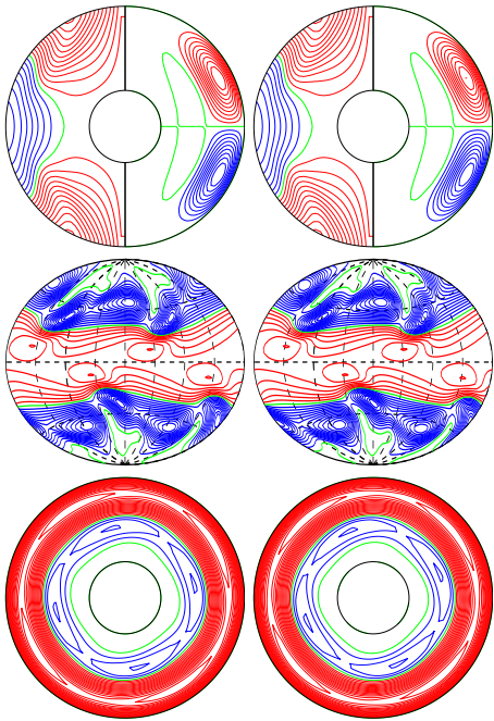
a.e03p01t03r-50000m1n2N2z14e4bb E_{\text{kin}}
