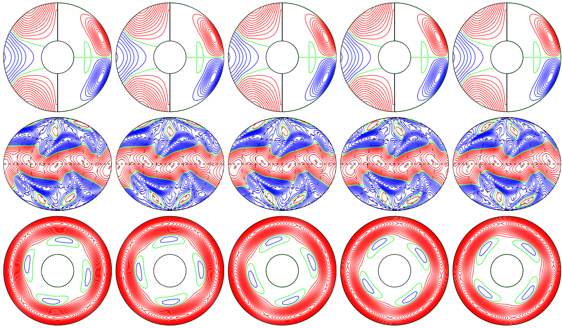
a.e03p01t03r-50000m1n2N2z12.5e4b E_{\text{kin}}
