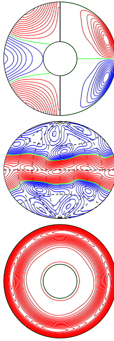
a.e03p01t03r-50000m1n2N2z8.4e4a E_{\text{kin}}
