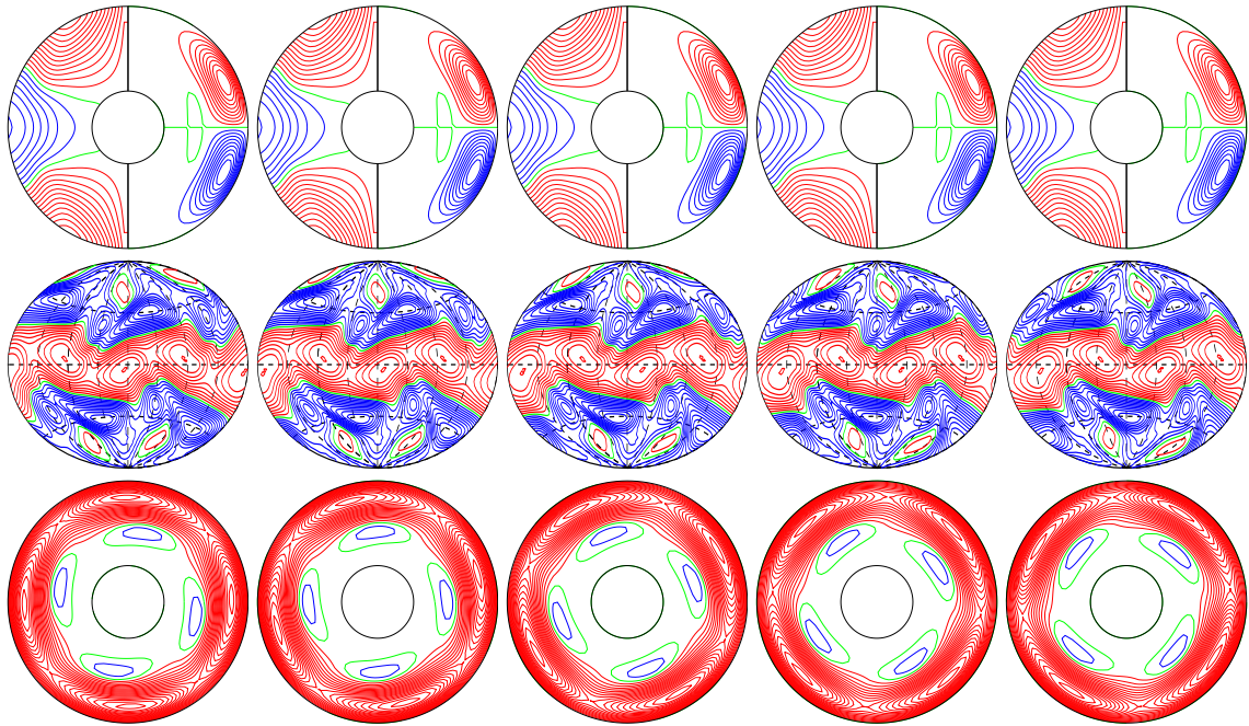
a.e03p01t03r-50000m1n2N2z12.5e4b E_{\text{kin}}
