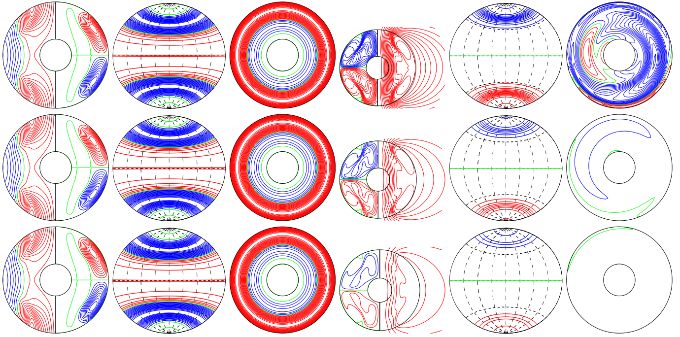
a.e03p01t03r-50000m1p5n2N2z15e4
