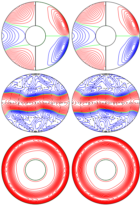
a.e03p01t03r-50000m1n2N2z8.3e4a E_{\text{kin}}
