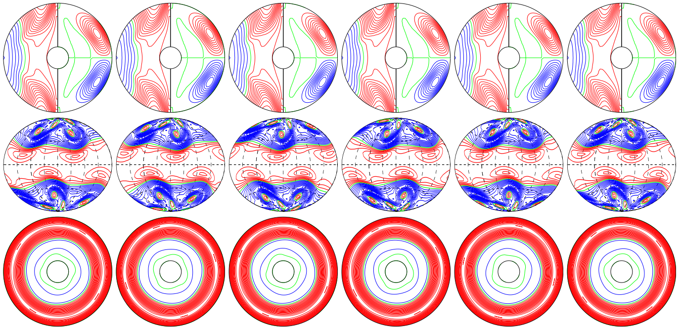
a.e02p001t03r-50000m1n2N2z5e5 E_{\text{kin}}
