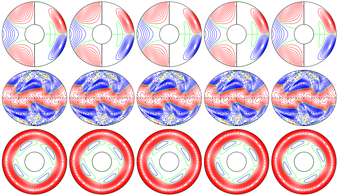
a.e03p01t03r-50000m1n2N2z13e4b E_{\text{kin}}
