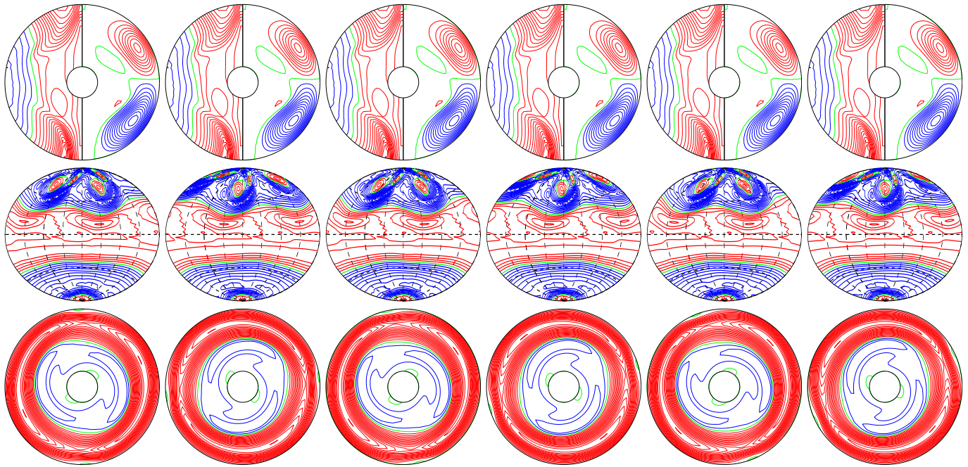
a.e02p001t03r-50000m1n2N2z8e5 E_{\text{kin}}
