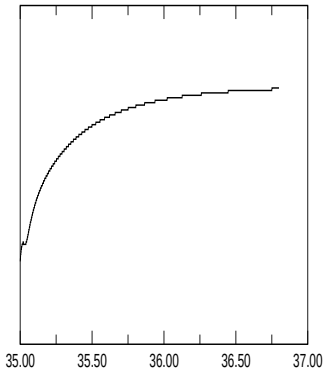
a.e03p01t03r-50000m1p5n2N2z15e4
