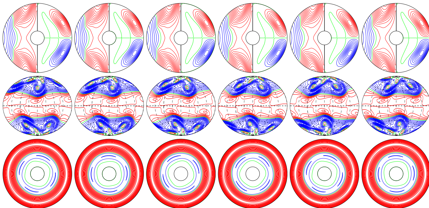
a.e02p001t03r-50000m1n2N2z4e5 E_{\text{kin}}
