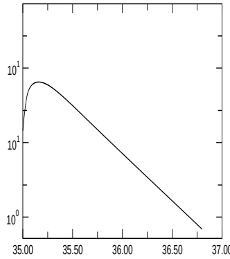
a.e03p01t03r-50000m1p5n2N2z15e4
