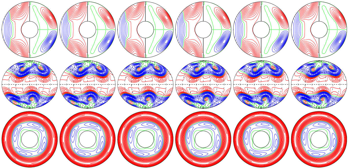
a.e03p01t03r-50000m1n2N2z20e4b E_{\text{kin}}
