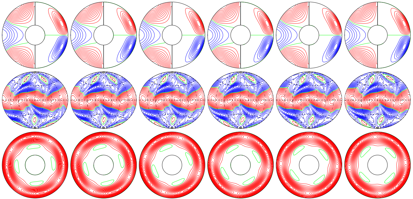
a.e03p01t03r-50000m1n2N2z11e4a E_{\text{kin}}
