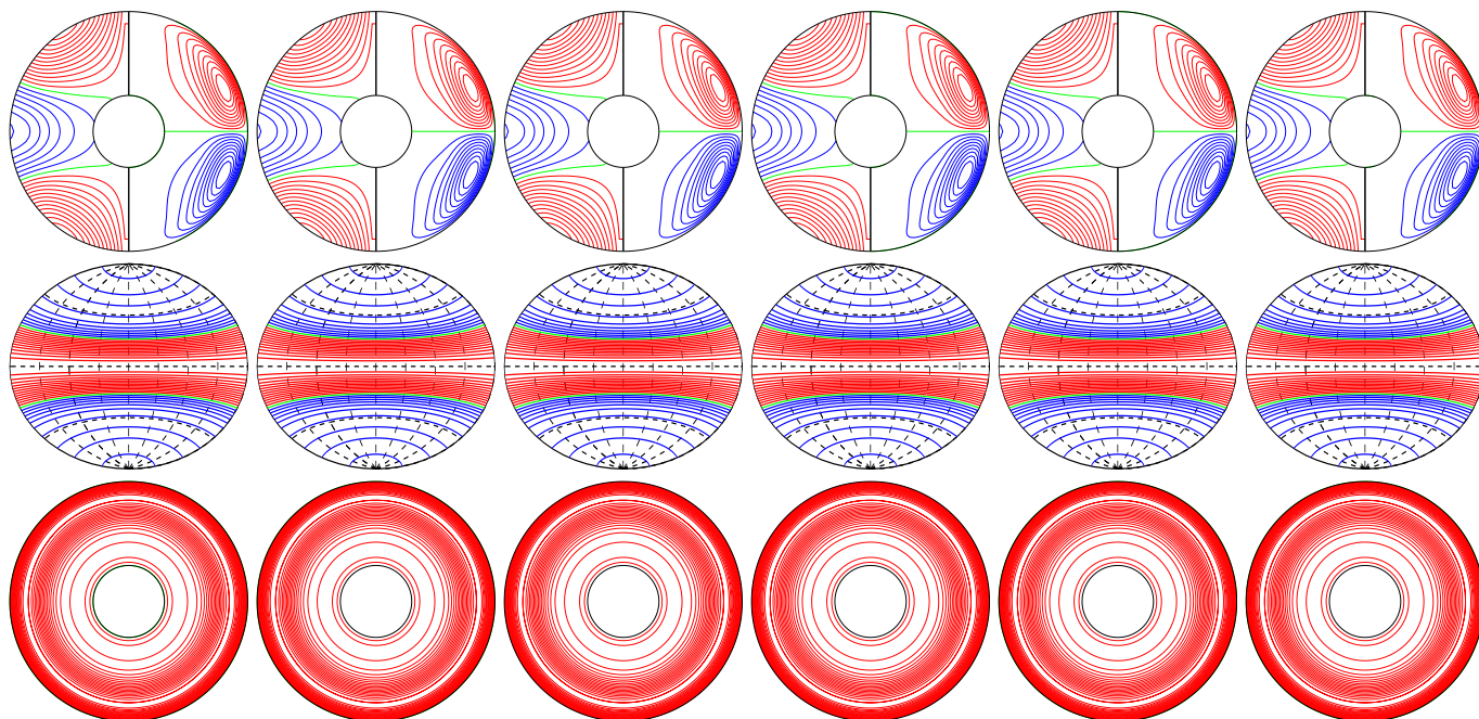
a.e03p01t03r-50000m1n2N2z6.5e4Y E_{\text{kin}}
