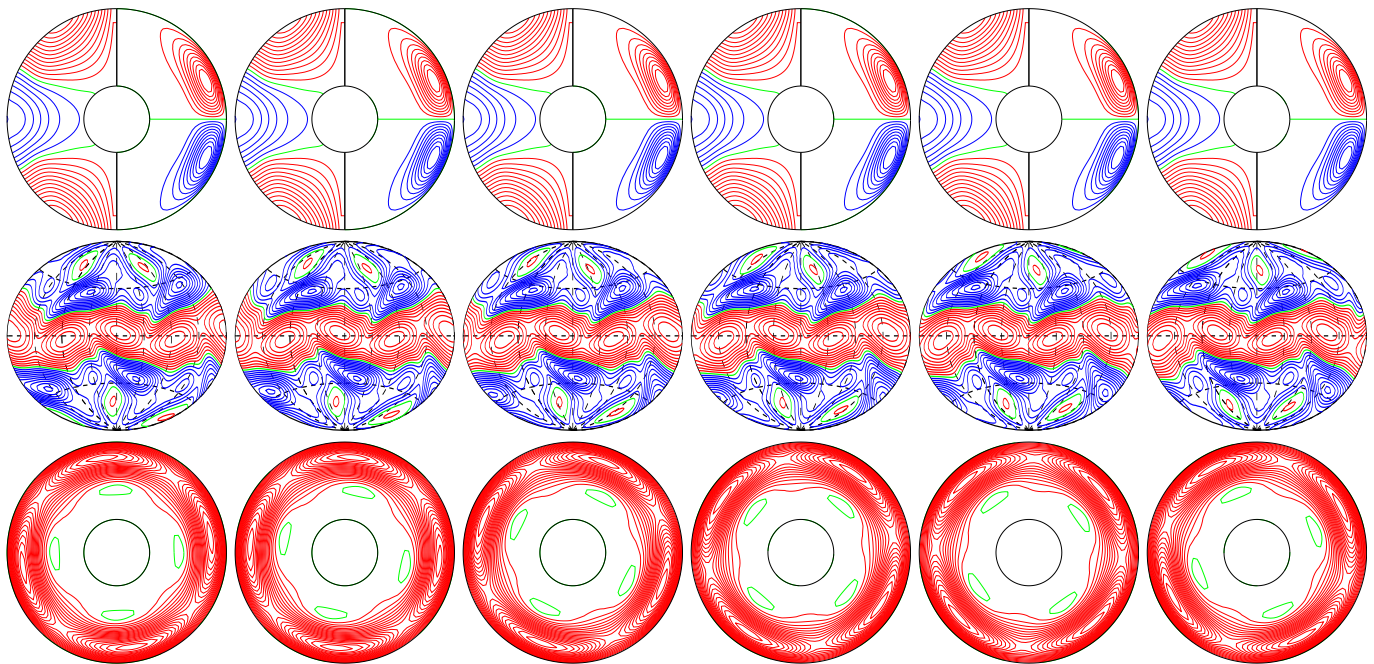
a.e03p01t03r-50000m1n2N2z10.4e4 E_{\text{kin}}
