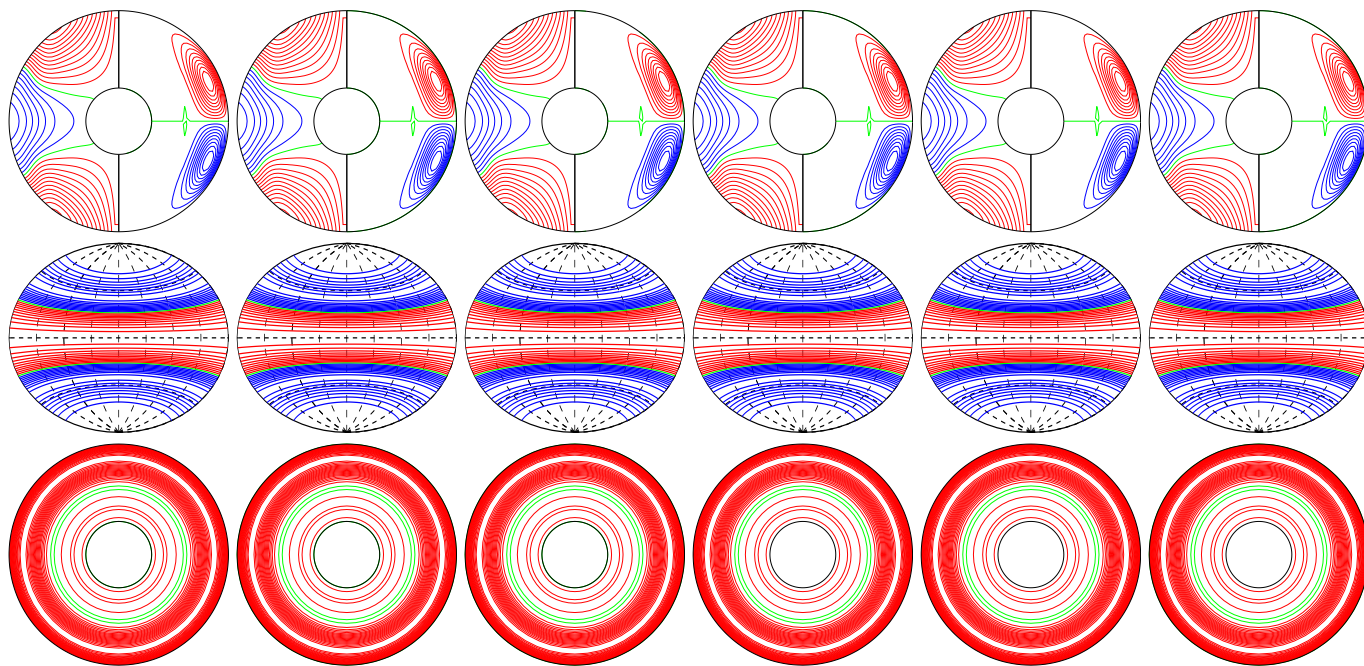
a.e03p01t03r-50000m16n2N2z12e4a E_{\text{kin}}
