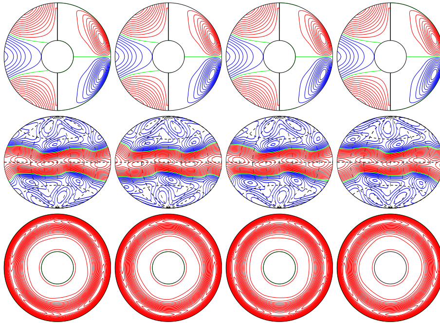
a.e03p01t03r-50000m1n2N2z8.3e4a E_{\text{kin}}
