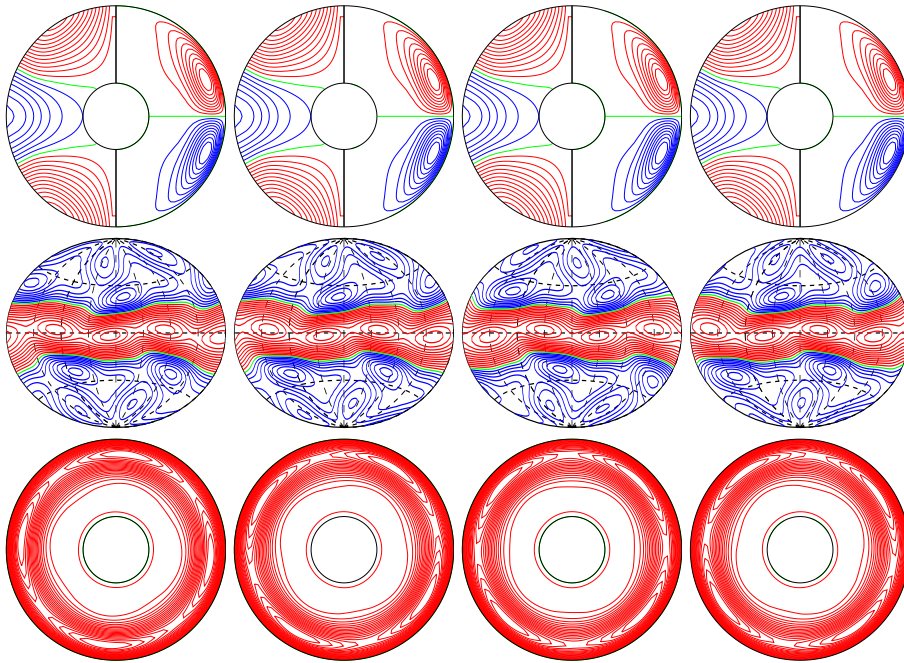
a.e03p01t03r-50000m1n2N2z8.4e4a E_{\text{kin}}
