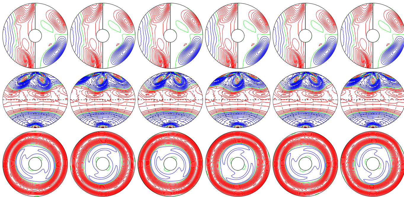
a.e02p001t03r-50000m1n2N2z8e5 E_{\text{kin}}
