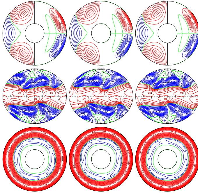
a.e03p01t03r-50000m1n2N2z13.5e4b E_{\text{kin}}
