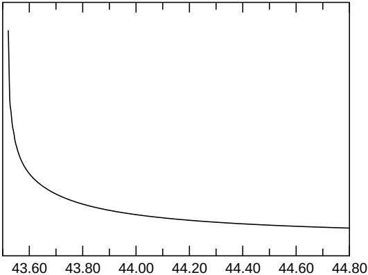
E_{kin,asymm.}
