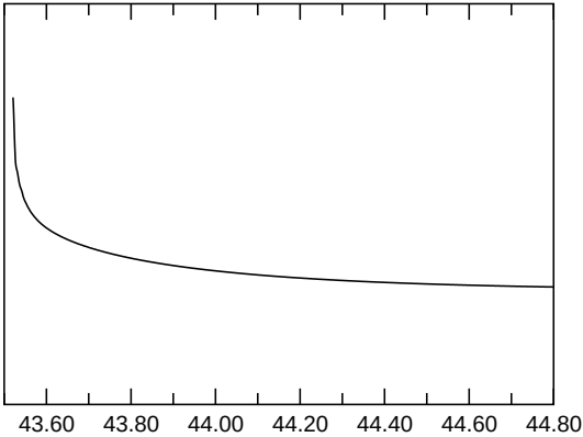
E_{kin,asymm.}
