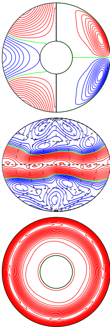
a.e03p01t03r-50000m1n2N2z8.2e4a E_{kin}
