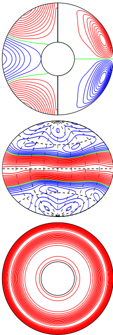
a.e03p01t03r-50000m1n2N2z7.9e4a E_{kin}
