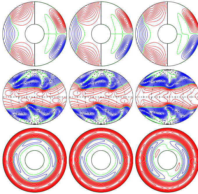
a.e03p01t03r-50000m1n2N2z14e4bb E_{\text{kin}}
