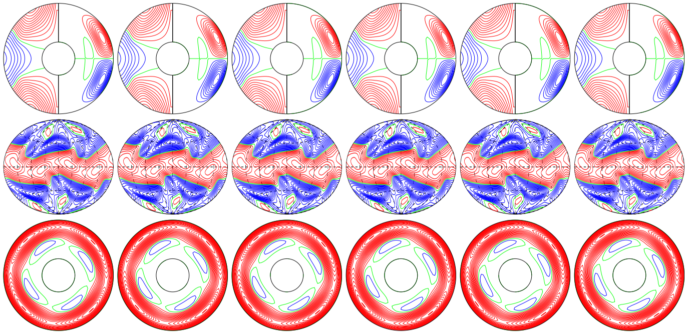
a.e03p01t03r-50000m1n2N2z13e4b E_{\text{kin}}
