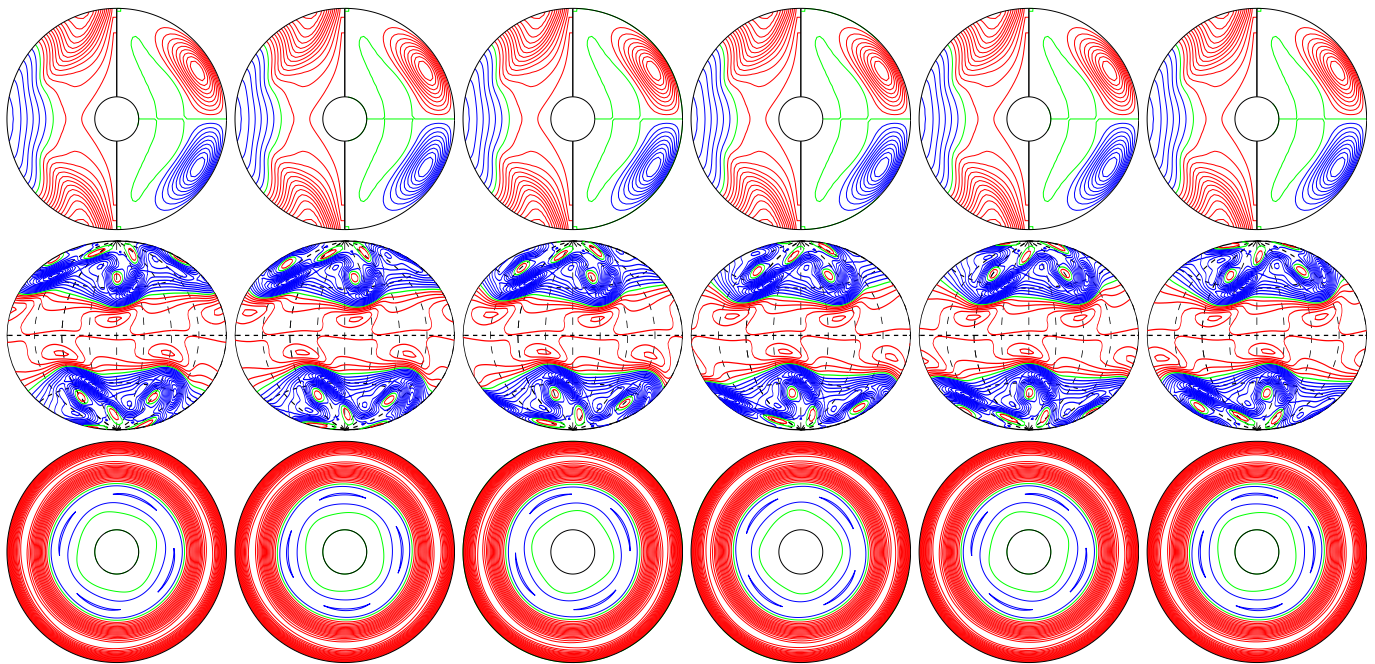
a.e02p001t03r-50000m1n2N2z4e5 E_{\text{kin}}
