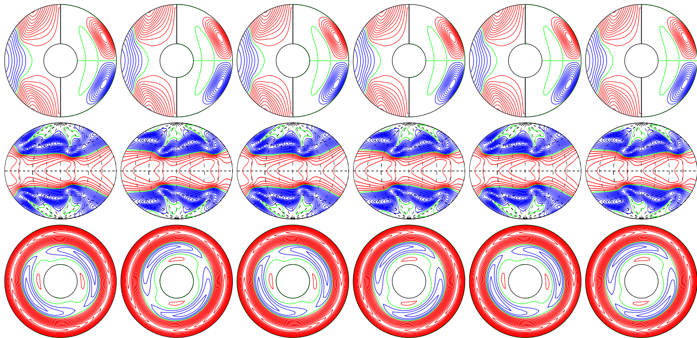
a.e03p01t03r-50000m1n2N2z13.5e4a E_{\text{kin}}
