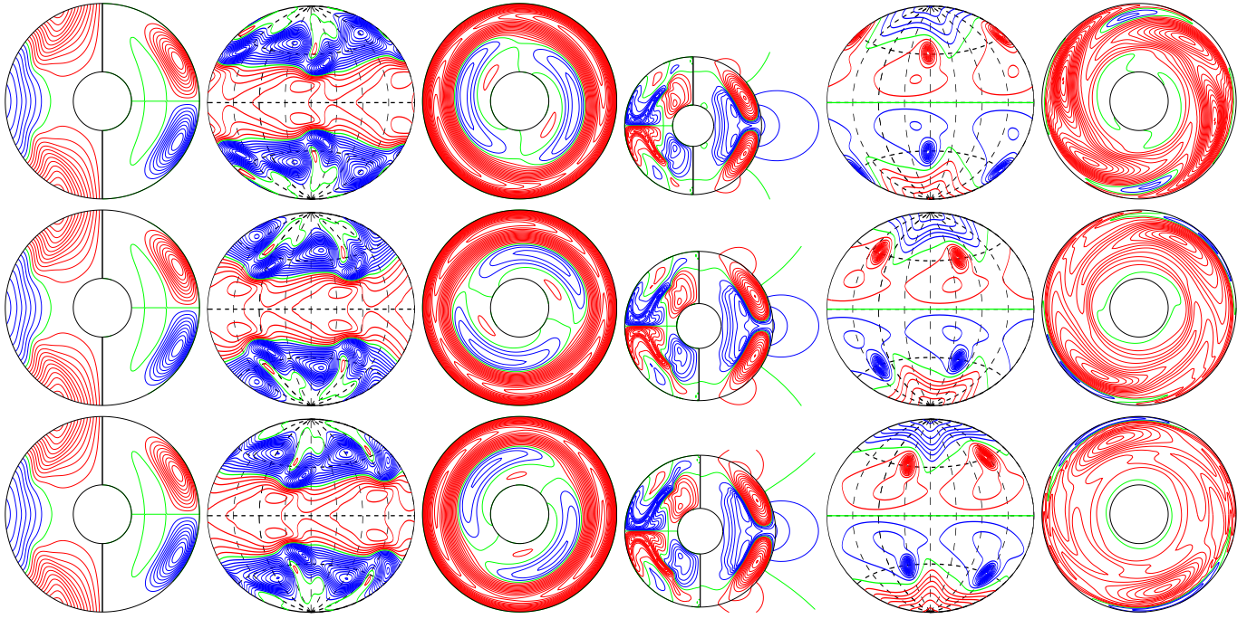
a.e03p01t03r-50000m2p18n2N2z15e4r E_{kin}
