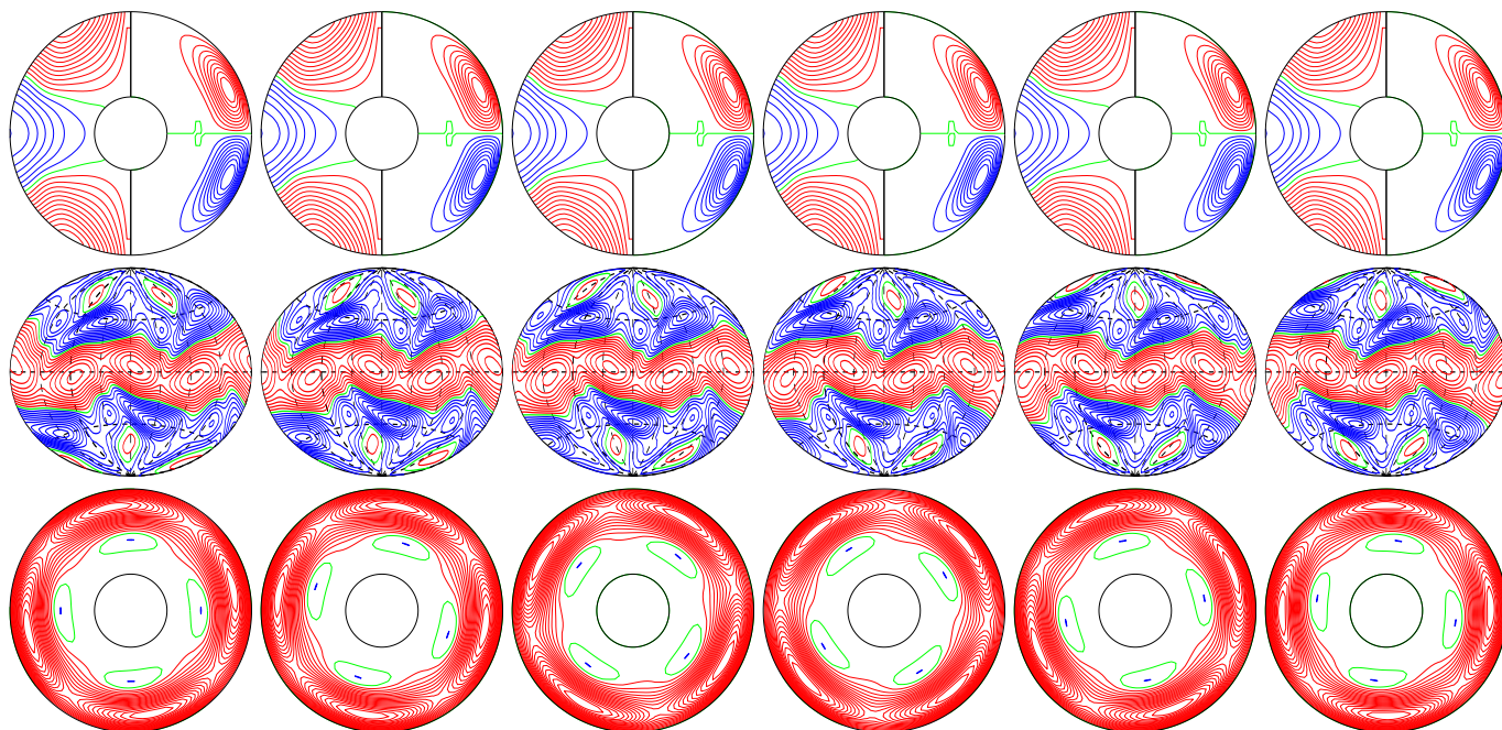
a.e03p01t03r-50000m1n2N2z11.5e4 E_{\text{kin}}
