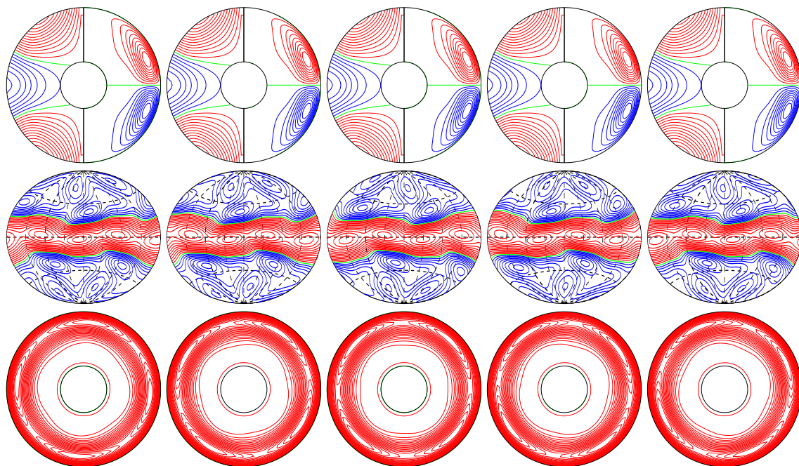
a.e03p01t03r-50000m1n2N2z8.4e4a E_{\text{kin}}
