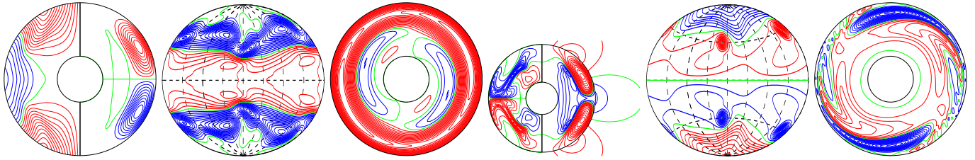
a.e03p01t03r-50000m2p14n2N2z15e4r E_{\text{kin}}
