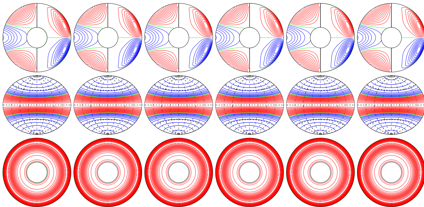
a.e03p01t03r-50000m1n2N2z6.5e4Y E_{\text{kin}}
