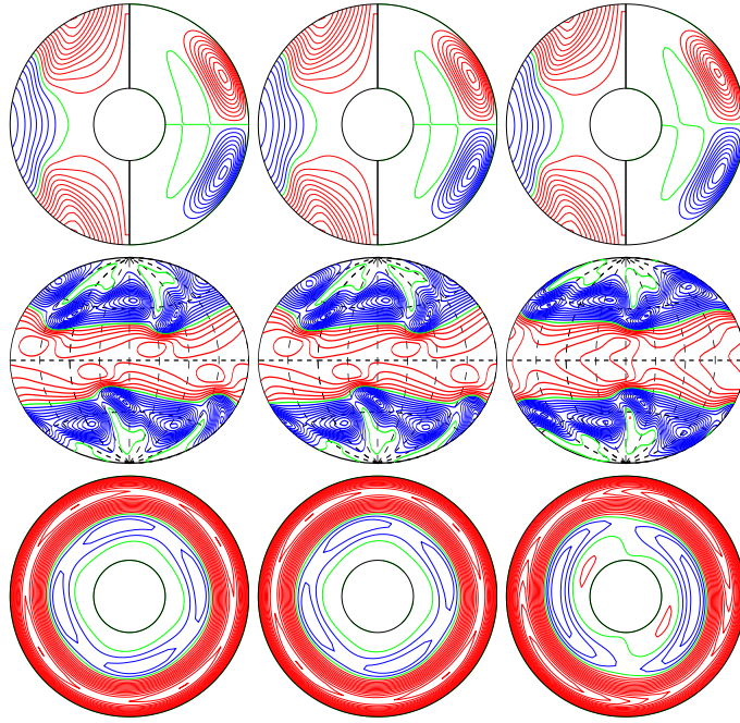
a.e03p01t03r-50000m1n2N2z14e4bb E_{\text{kin}}
