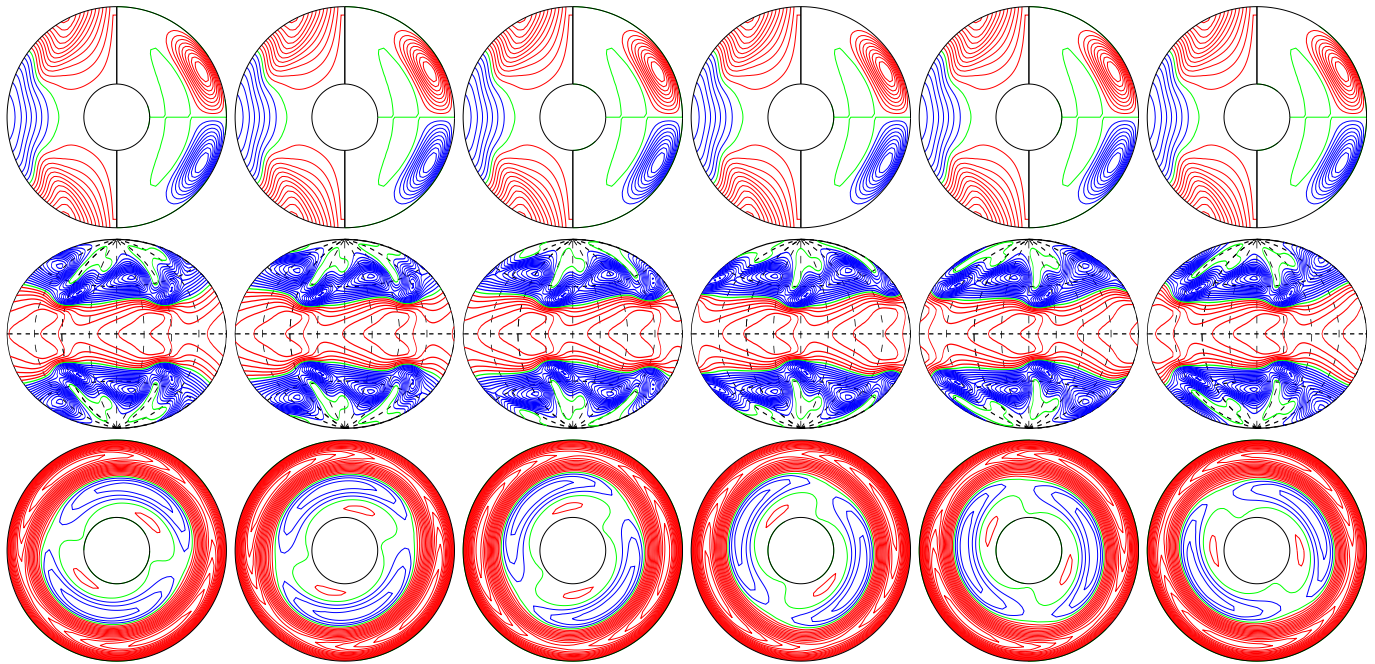
a.e03p01t03r-50000m1n2N2z14e4a E_{\text{kin}}
