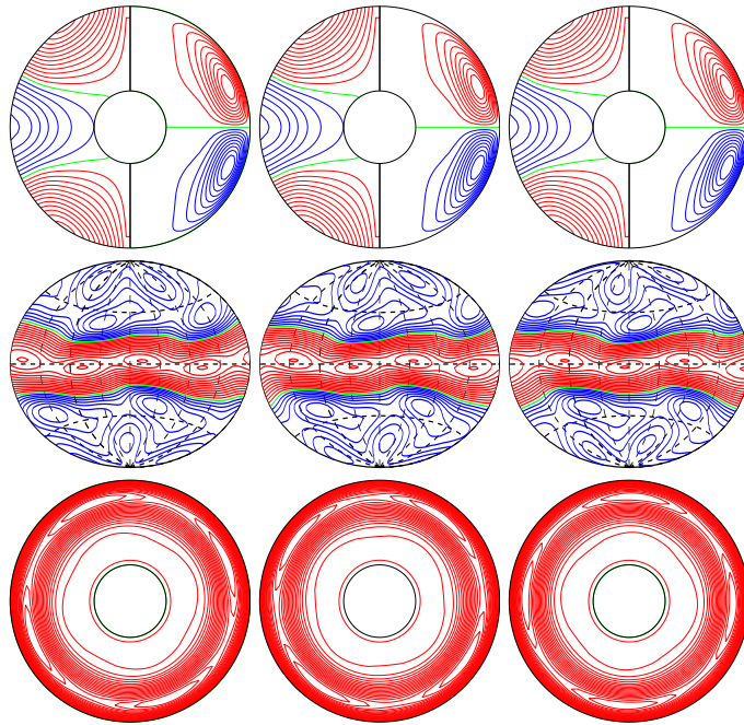
a.e03p01t03r-50000m1n2N2z8.2e4a E_{\text{kin}}
