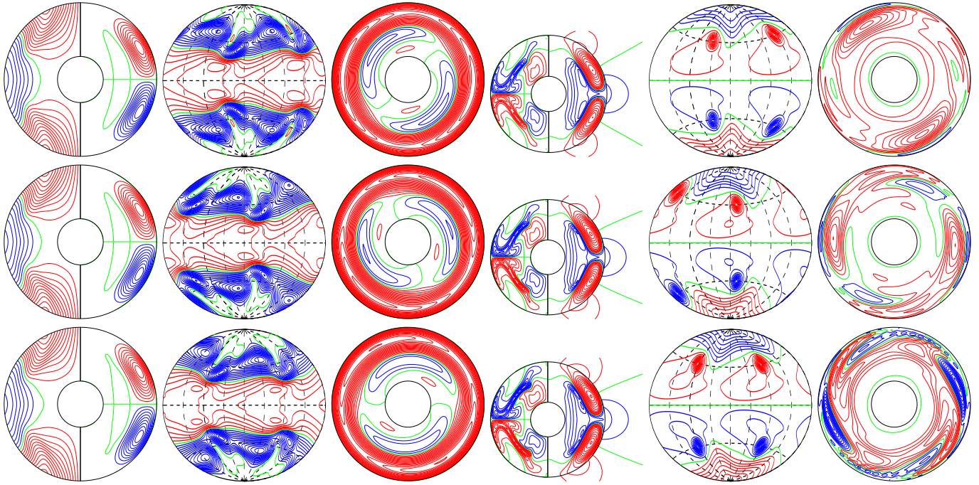
a.e03p01t03r-50000m2p16n2N2z15e4r E_{kin}
