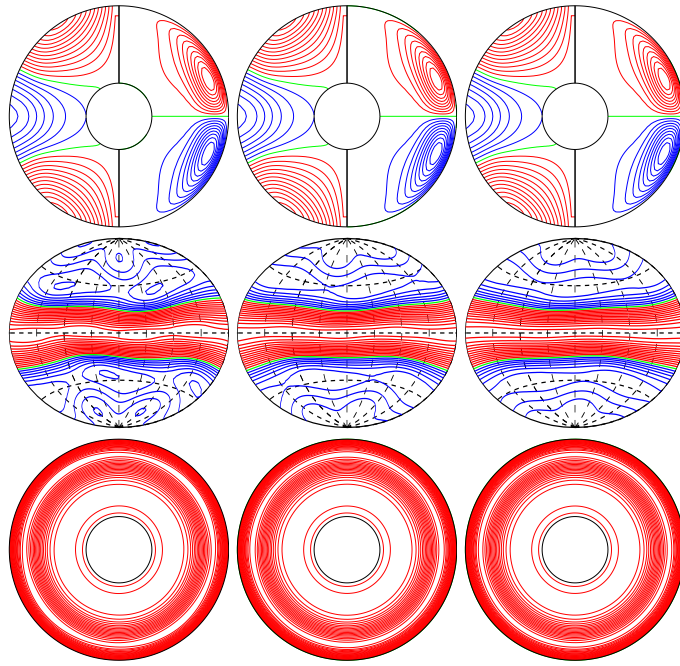
a.e03p01t03r-50000m1n2N2z7.9e4a E_{\text{kin}}
