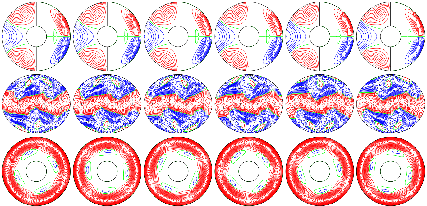
a.e03p01t03r-50000m1n2N2z12e4b E_{\text{kin}}
