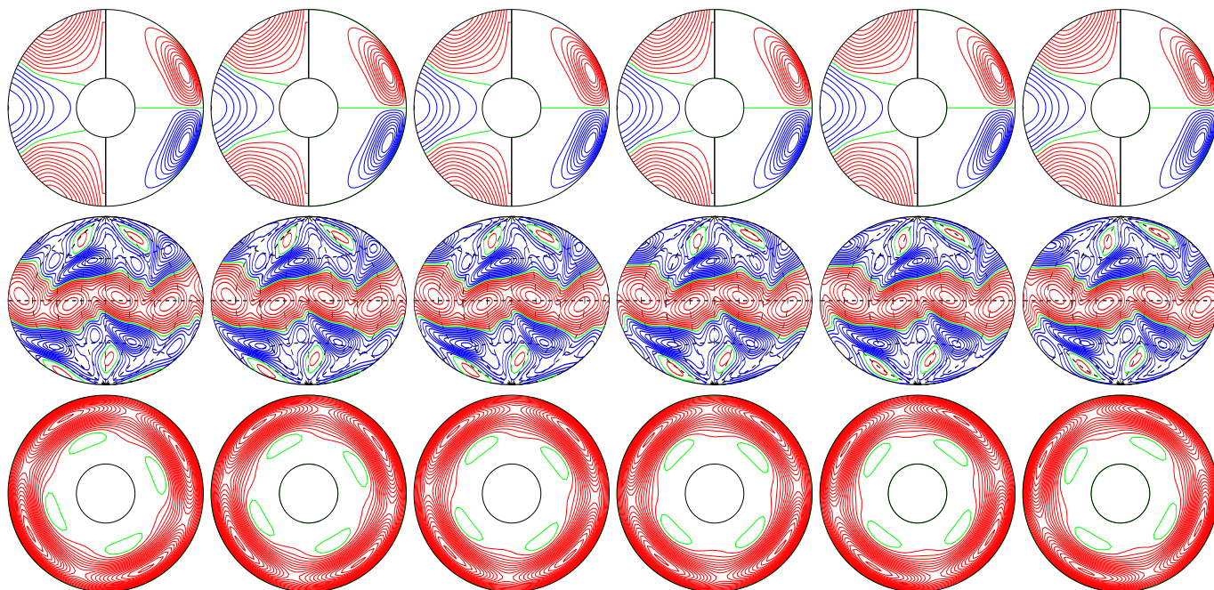
a.e03p01t03r-50000m1n2N2z11e4a E_{\text{kin}}
