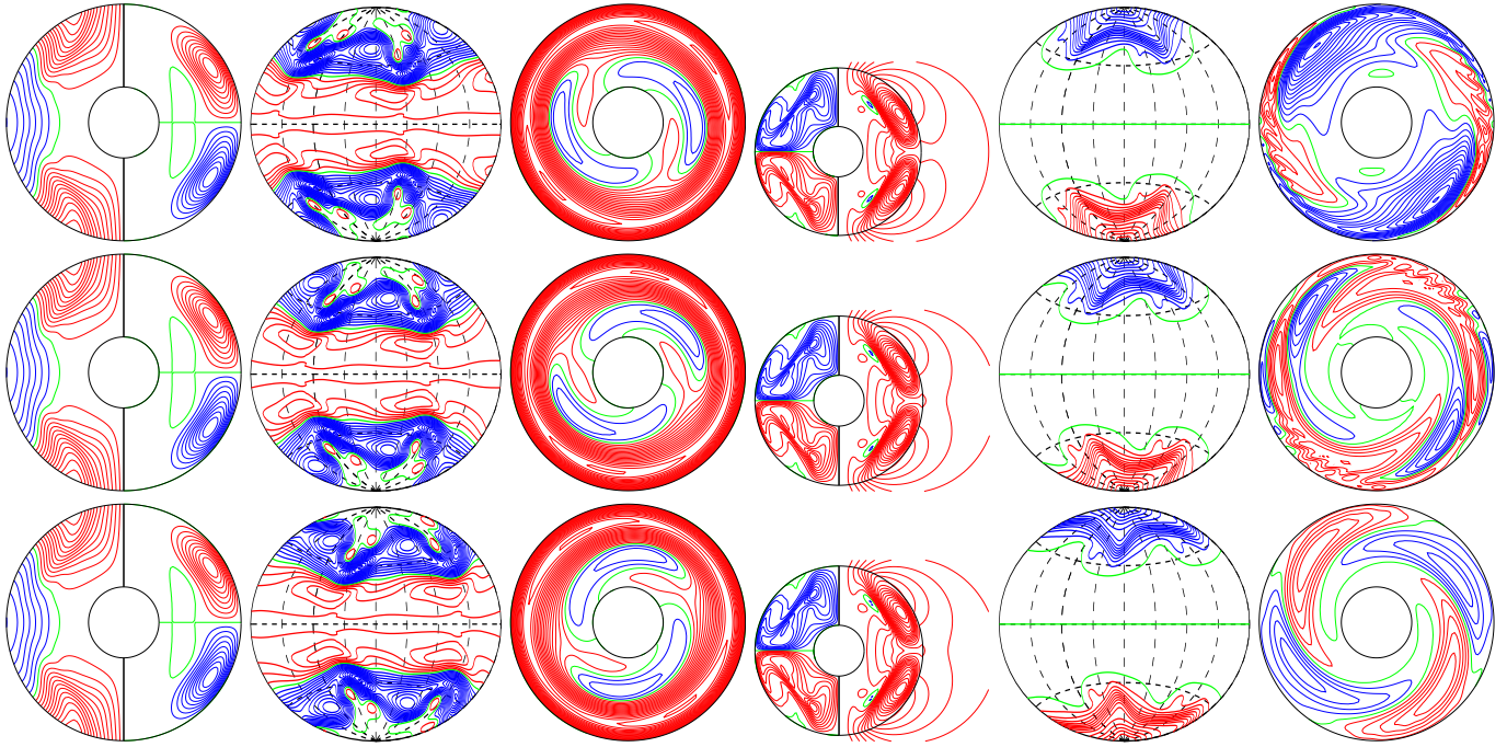
a.e03p008t03r-50000m2p6n2N2z20e4s E_{\text{kin}}
