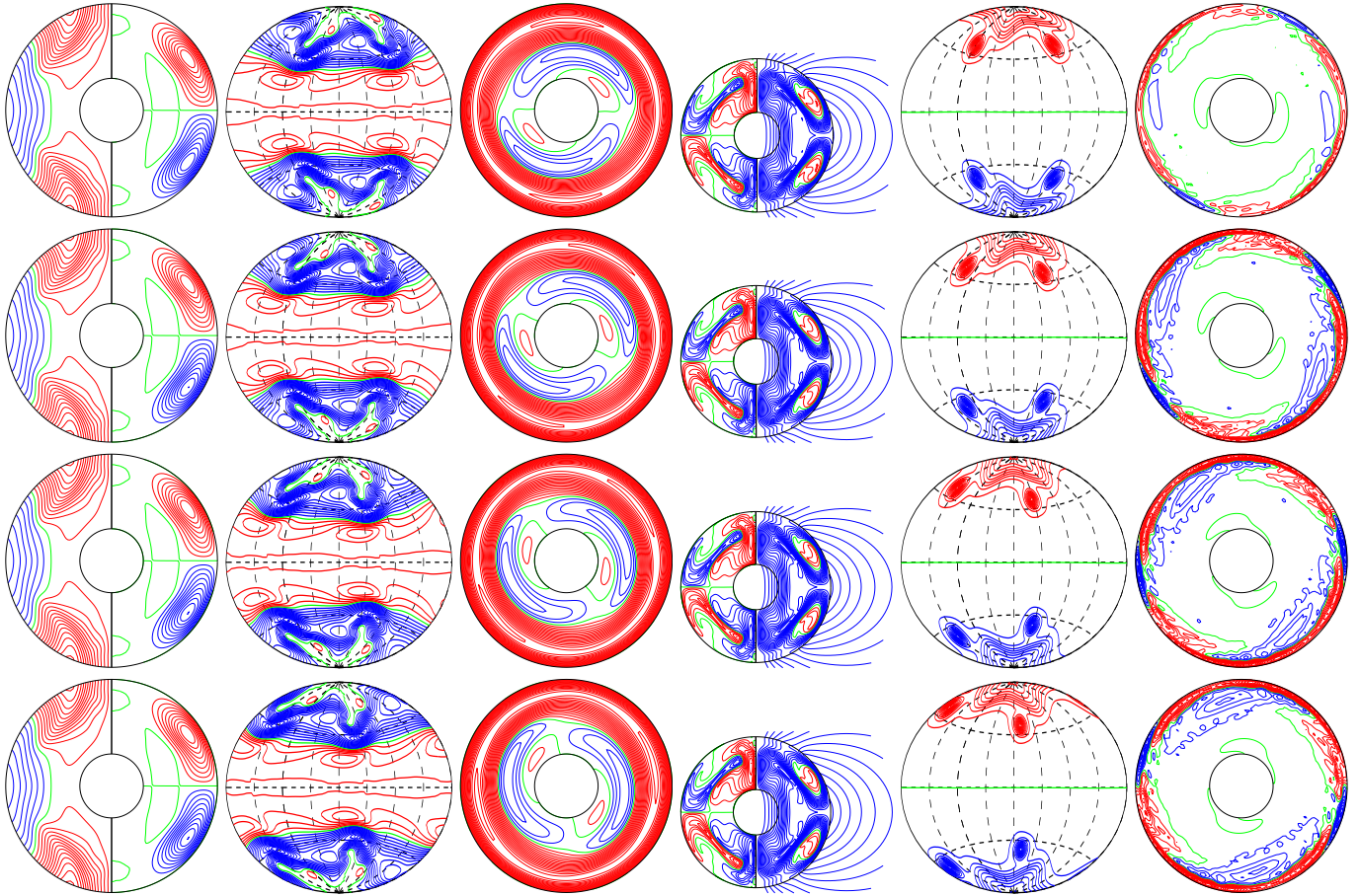
a.e03p01t025r-50000m2p16n2N2z17e4s
