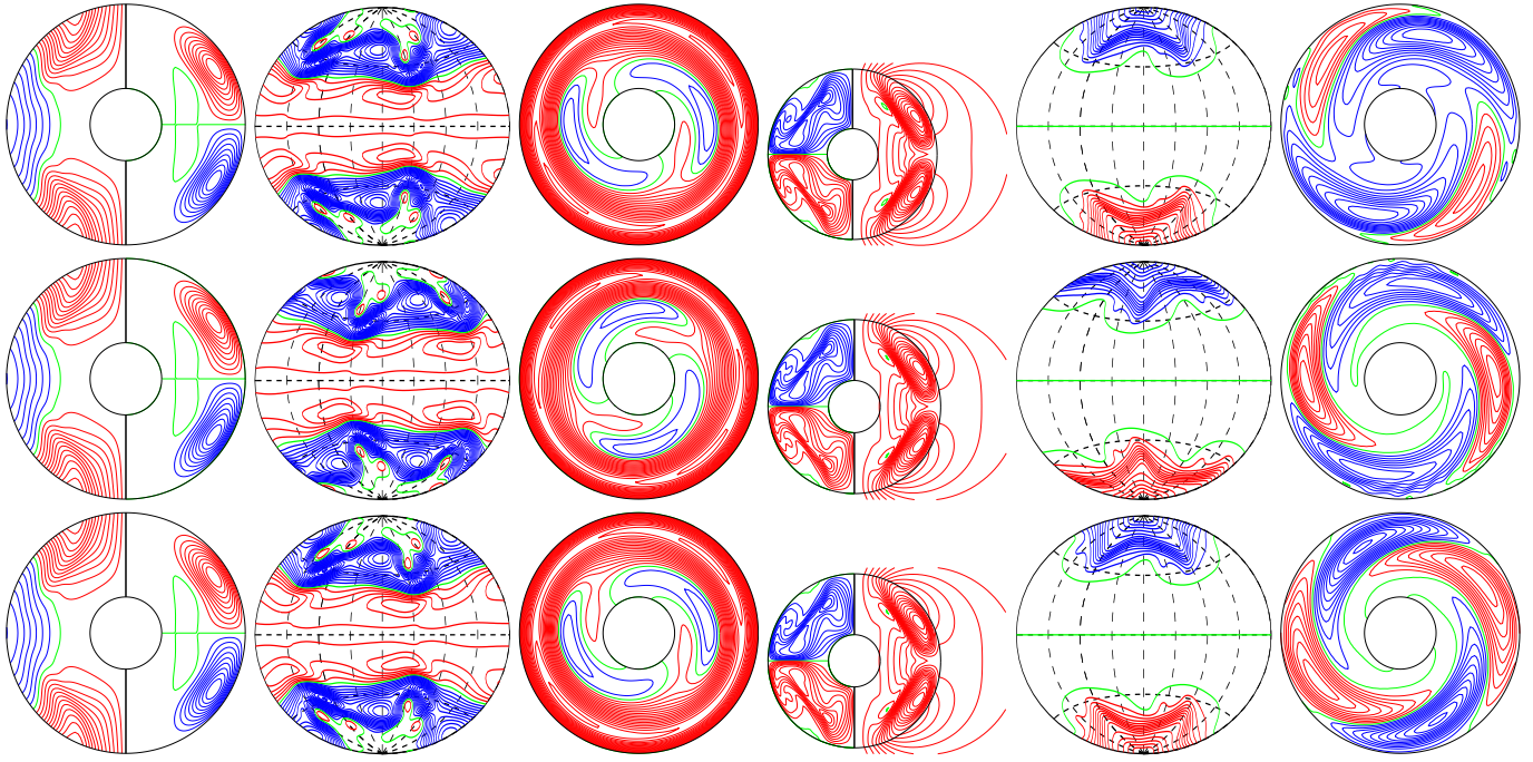
a.e03p008t03r-50000m2p5n2N2z20e4s E_{kin}
