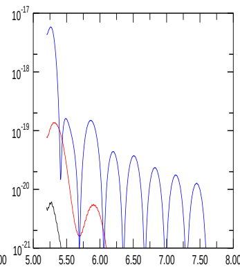
E_{\text{magn, quadr.}}
