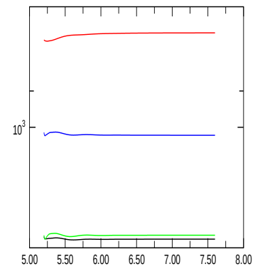
E_{\text{magn, dip.}}
