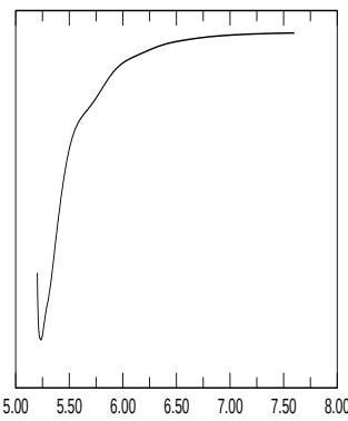
E_{\text{magn, quadr.}}
