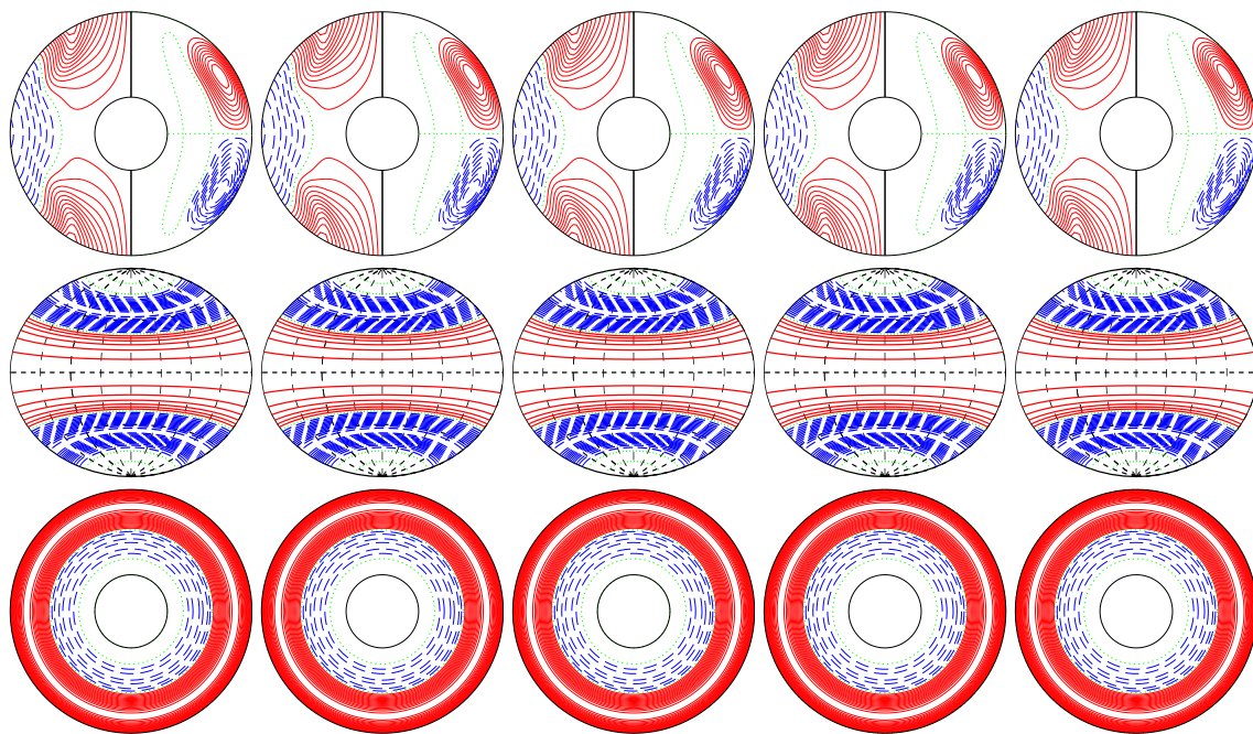
a.e03p005t03r-50000m1n2N2z14e4 E_{\text{kin}}
