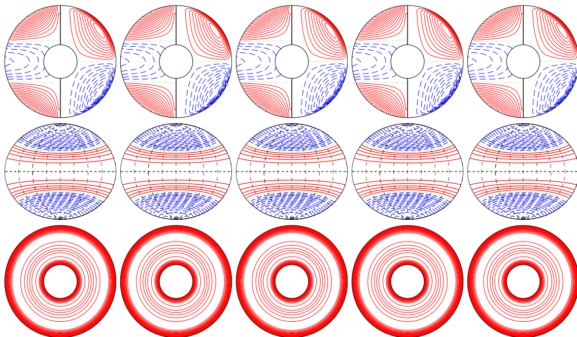
a.e03p005t06r-50000m1n2N2z1e3 E_{\text{kin}}
