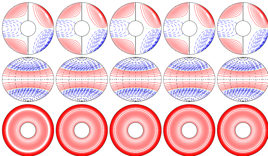
a.e03p005t03r-50000m1n2N2z1e4 E_{\text{kin}}
