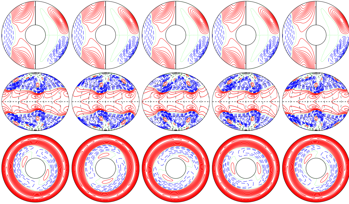
a.e03p005t03r-50000m1n2N2z20e4 E_{\text{kin}}
