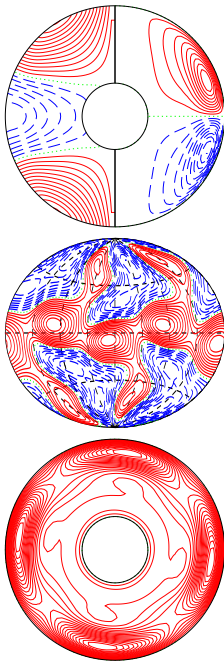
a.e03p005t06r-50000m1n2N2z25e4a E_{\text{kin}}
