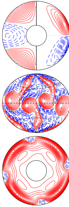
a.e03p005t06r-50000m1n2N2z30e4a E_{\text{kin}}
