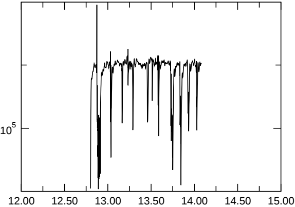
E_{kin,asymm.}
