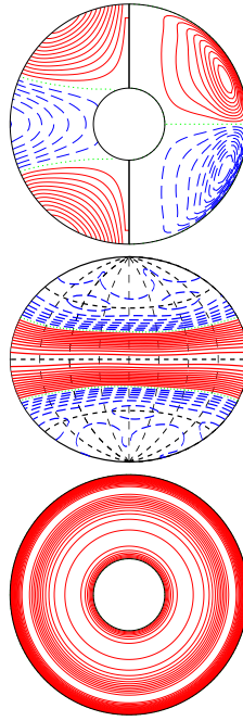
a.e03p005t06r-50000m1n2N2z20e4a E_{\text{kin}}
