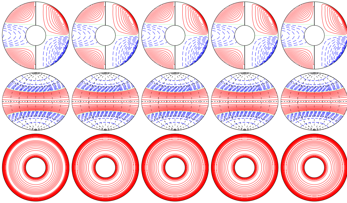
a.e03p005t06r-50000m1n2N2z10e4 E_{\text{kin}}
