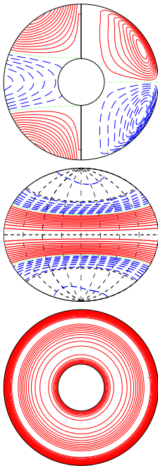
a.e03p005t06r-50000m1n2N2z14e4a E_{\text{kin}}
