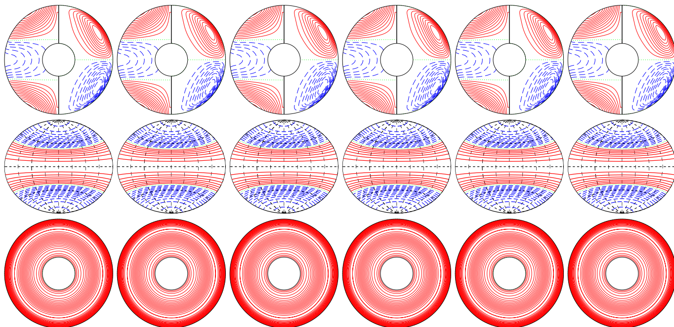
a.e03p005t03r-50000m1n2N2z1e4 E_{\text{kin}}
