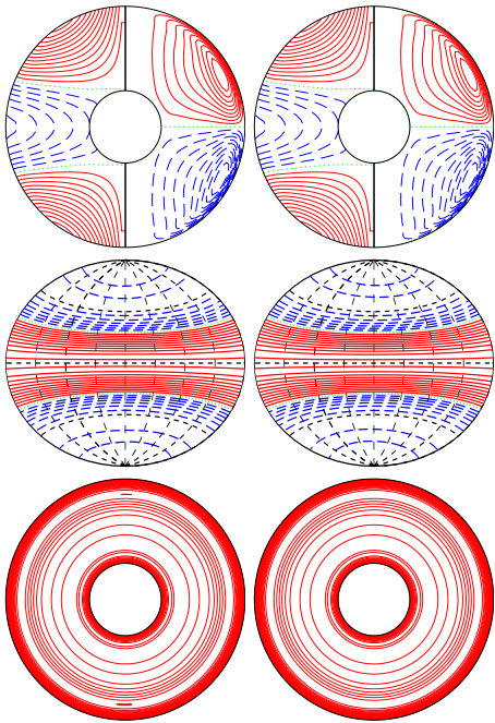
a.e03p005t1r-50000m1n2N2z34e4 E_{kin}
