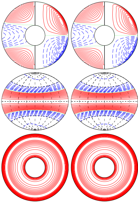
a.e03p005t06r-50000m1n2N2z14e4a E_{kin}
