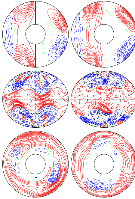
a.e03p001t06r-50000m1n2N2z9e5 E_{\text{kin}}
