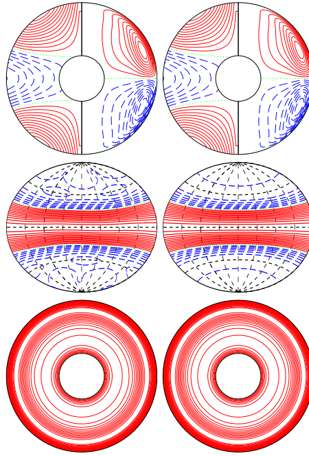
a.e03p005t06r-50000m1n2N2z20e4a E_{\text{kin}}
