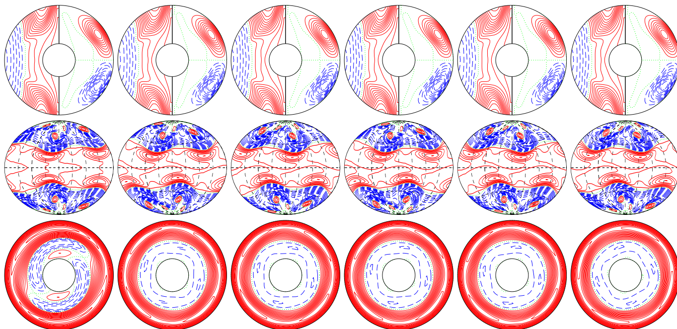
a.e03p005t03r-50000m1n2N2z30e4 E_{\text{kin}}
