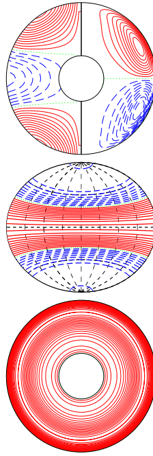
a.e03p005t03r-50000m1n2N2z4e4 E_{\text{kin}}
