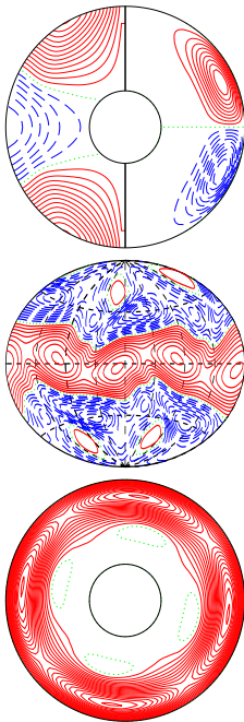
a.e03p005t03r-50000m1n2N2z12e4b E_{\text{kin}}
