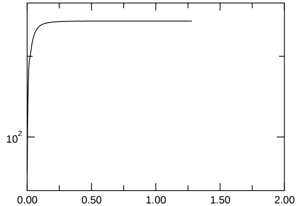
E_{kin,asymm.}
