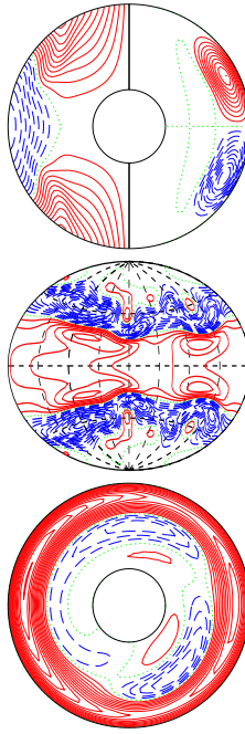
a.e03p005t06r-50000m1n2N2z32e4a E_{\text{kin}}
