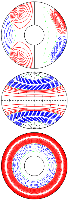
a.e03p005t03r-50000m1n2N2z14e4a E_{\text{kin}}
