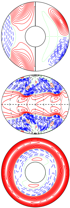
a.e03p005t03r-50000m1n2N2z18e4a E_{\text{kin}}
