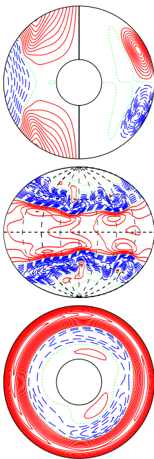
a.e03p005t06r-50000m1n2N2z31e4a E_{\text{kin}}
