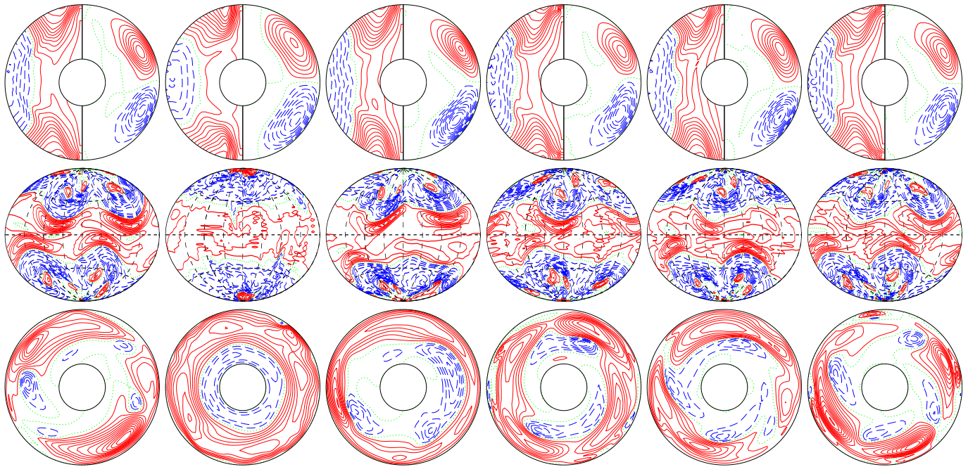
a.e03p001t06r-50000m1n2N2z9e5 E_{\text{kin}}
