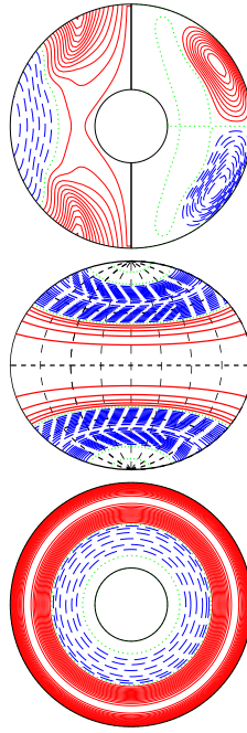
a.e03p005t03r-50000m1n2N2z16e4b E_{\text{kin}}
