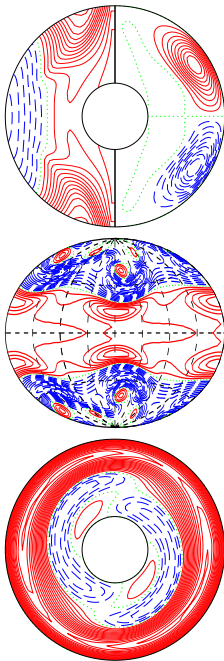
a.e03p005t03r-50000m1n2N2z28e4b E_{kin}
