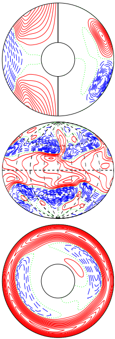
a.e03p005t06r-50000m1n2N2z33e4a E_{\text{kin}}
