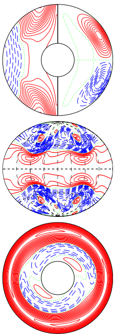
a.e03p005t03r-50000m1n2N2z23e4b E_{\text{kin}}
