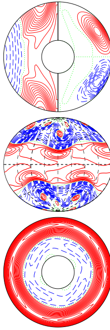
a.e03p005t03r-50000m1n2N2z28e4a E_{\text{kin}}
