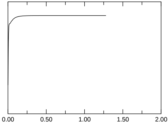
E_{kin,asymm.}
