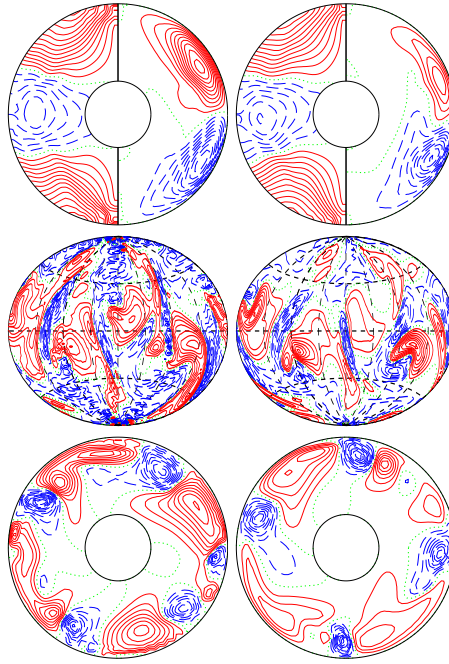
a.e03p003t1r-50000m1n2N2z13e5 E_{\text{kin}}
