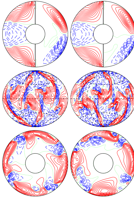
a.e03p002t1r-50000m1n2N2z13e5b E_{\text{kin}}
