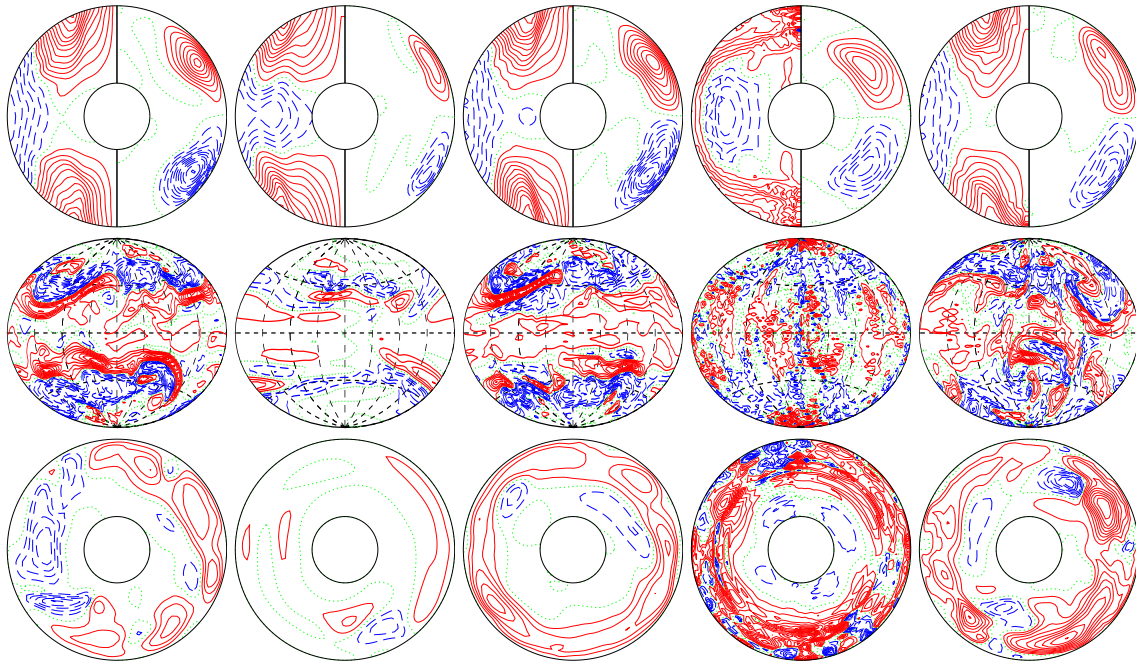
a.e03p002t1r-50000m1n2N2z17e5 E_{kin}
