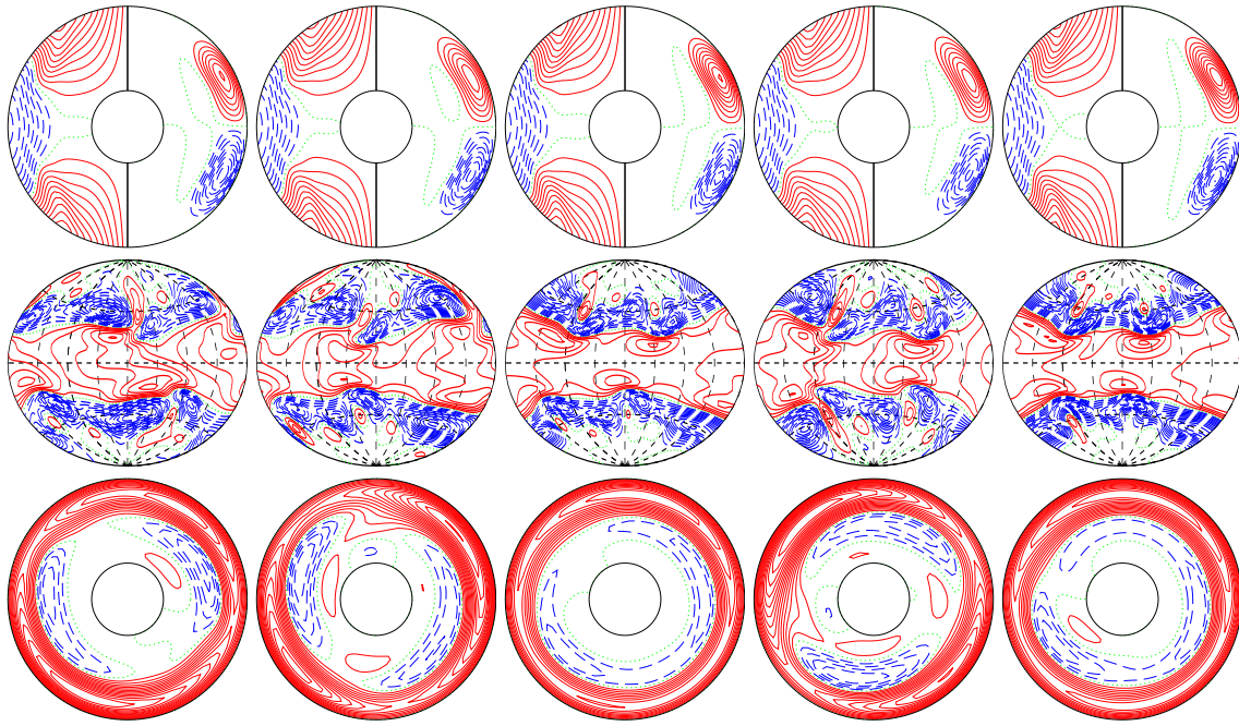
a.e03p005t06r-50000m1n2N2z33e4a E_{\text{kin}}
