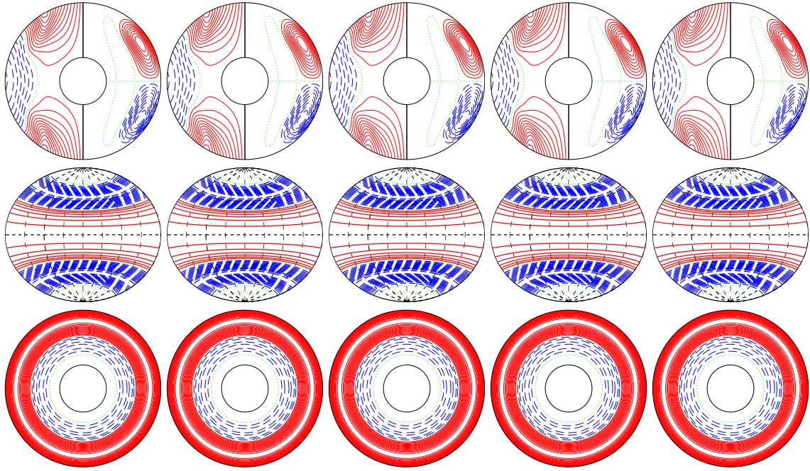
a.e03p005t03r-50000m1n2N2z14e4a E_{\text{kin}}
