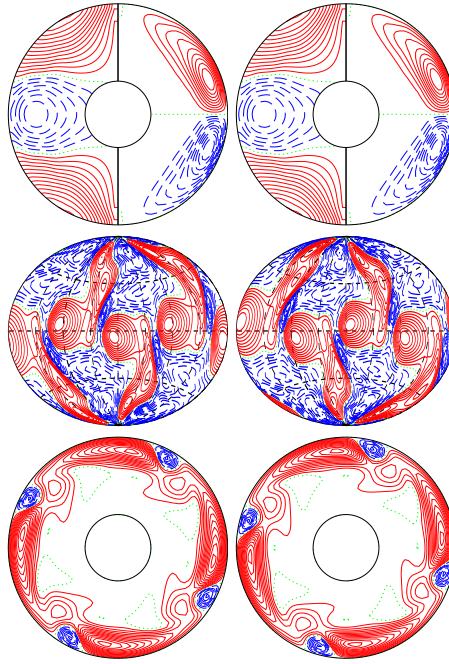
a.e03p003t1r-50000m1n2N2z9e5 E_{\text{kin}}
