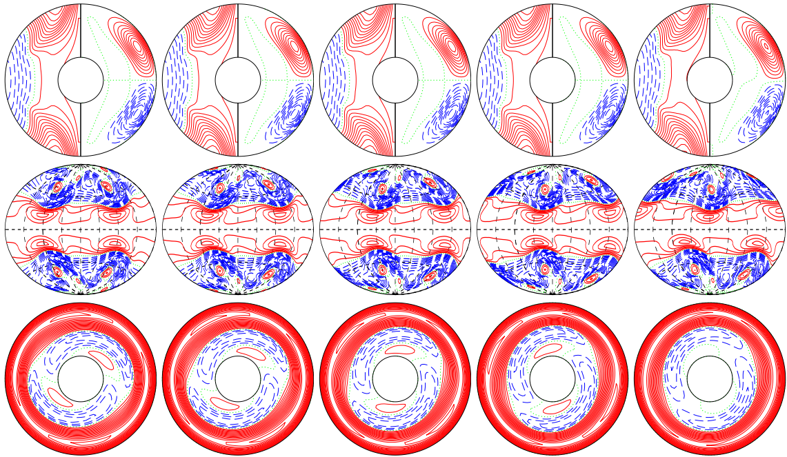
a.e03p005t03r-50000m1n2N2z23e4b E_{\text{kin}}
