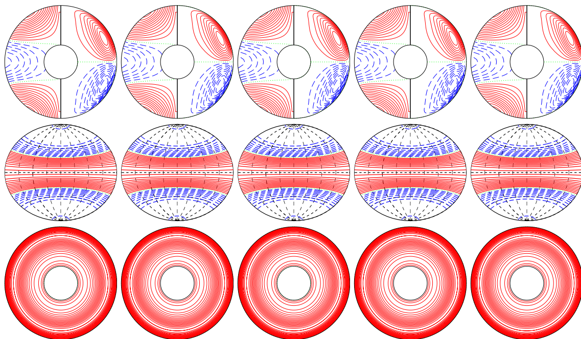
a.e03p005t03r-50000m1n2N2z4e4 E_{\text{kin}}
