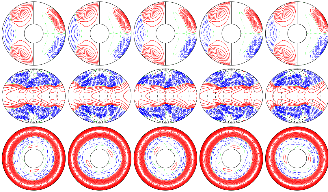
a.e03p005t03r-50000m1n2N2z16e4a E_{\text{kin}}
