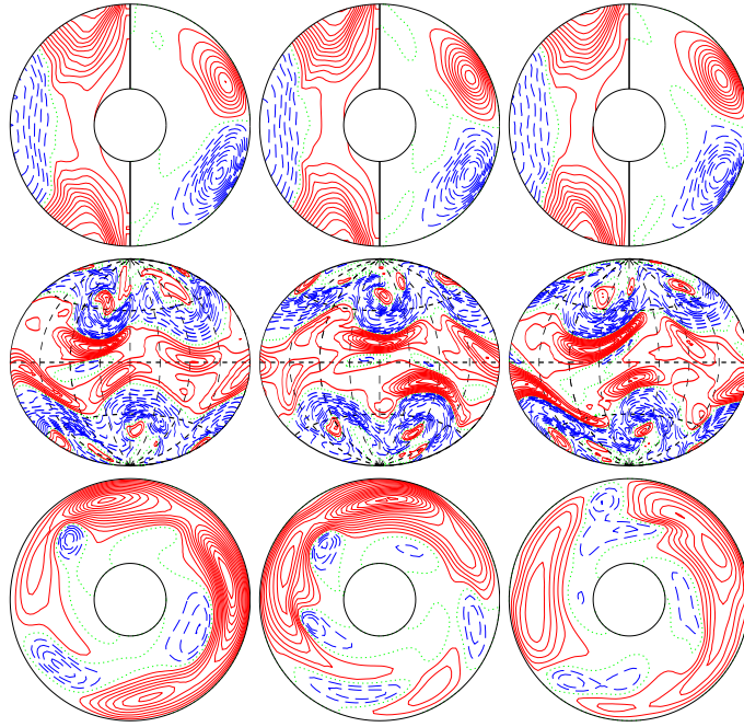
a.e03p002t06r-50000m1n2N2z9e5 E_{\text{kin}}
