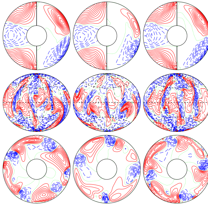
a.e03p003t1r-50000m1n2N2z13e5 E_{\text{kin}}
