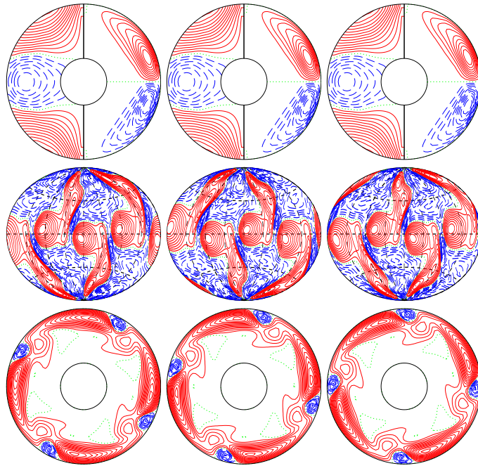
a.e03p003t1r-50000m1n2N2z9e5 E_{\text{kin}}
