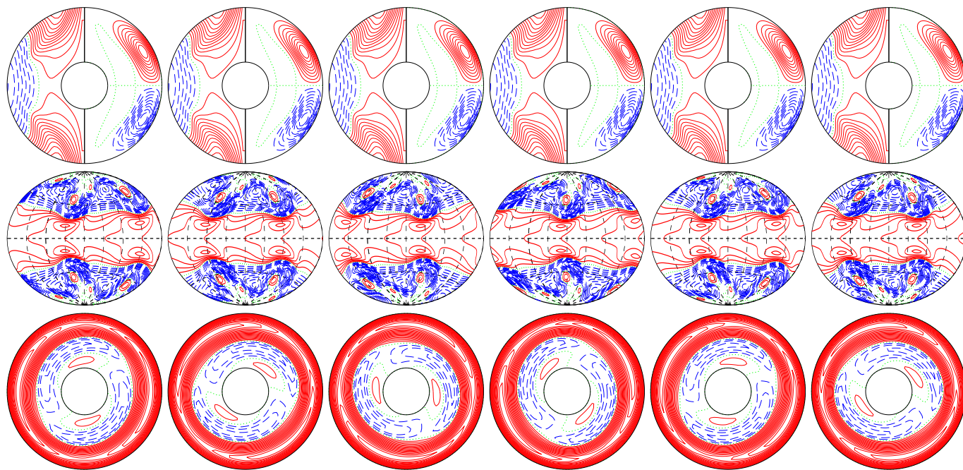
a.e03p005t03r-50000m1n2N2z20e4 E_{\text{kin}}
