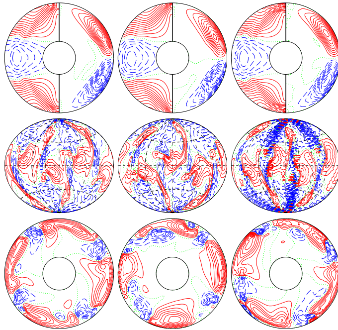
a.e03p002t1r-50000m1n2N2z13e5b E_{\text{kin}}
