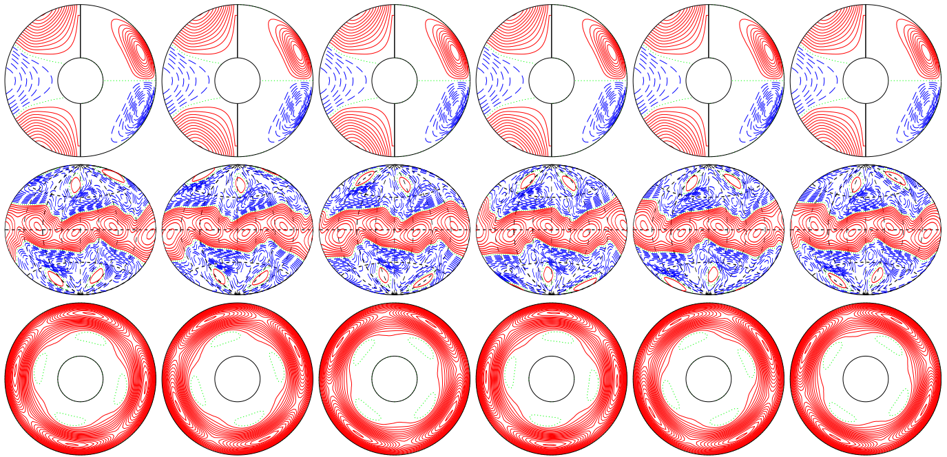
a.e03p005t03r-50000m1n2N2z12e4b E_{\text{kin}}
