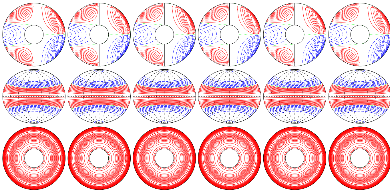
a.e03p005t03r-50000m1n2N2z4e4 E_{\text{kin}}
