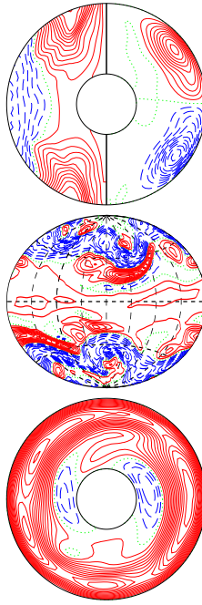
a.e03p003t06r-50000m1n2N2z9e5 E_{\text{kin}}
