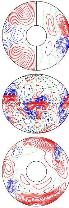
a.e03p003t1r-50000m1n2N2z15e5 E_{\text{kin}}
