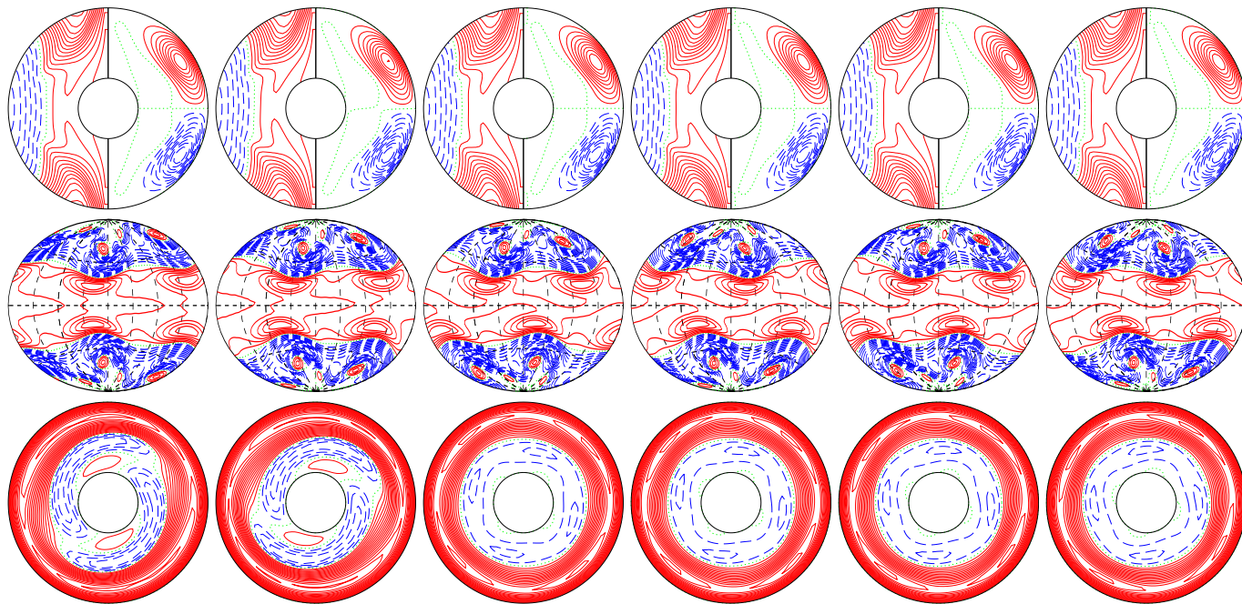
a.e03p005t03r-50000m1n2N2z28e4b E_{\text{kin}}
