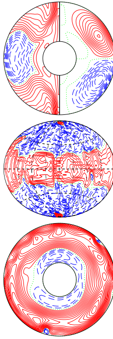
a.e03p003t06r-50000m1n2N2z13e5 E_{\text{kin}}
