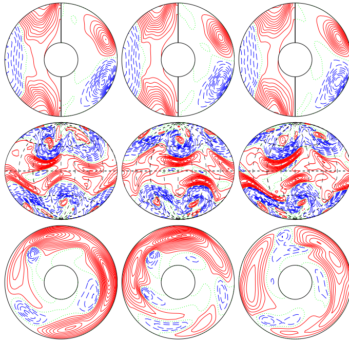
a.e03p002t06r-50000m1n2N2z9e5 E_{\text{kin}}
