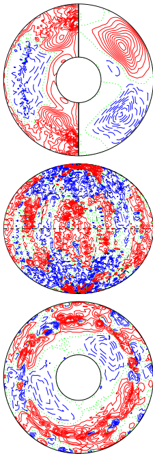
a.e03p003t06r-50000m1n2N2z17e5 E_{\text{kin}}
