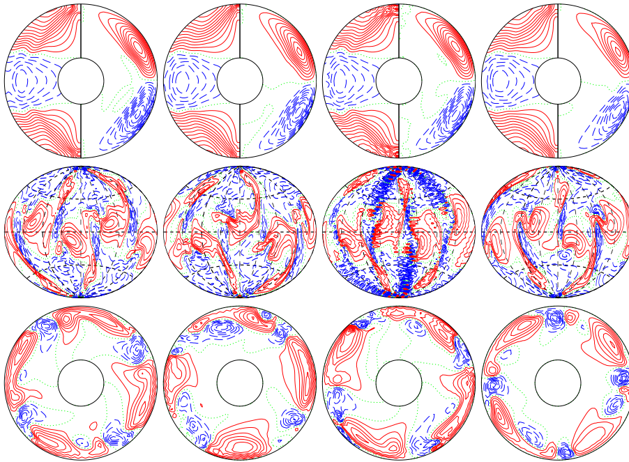
a.e03p002t1r-50000m1n2N2z13e5b E_{\text{kin}}
