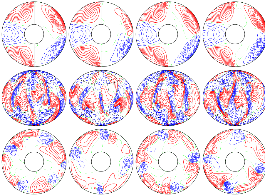
a.e03p003t1r-50000m1n2N2z13e5 E_{\text{kin}}
