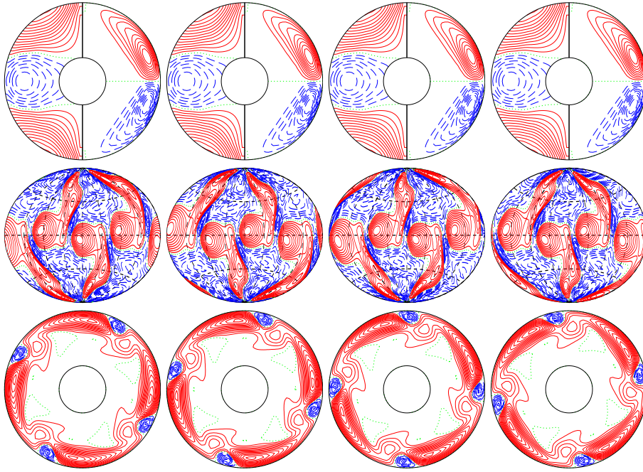
a.e03p003t1r-50000m1n2N2z9e5 E_{\text{kin}}
