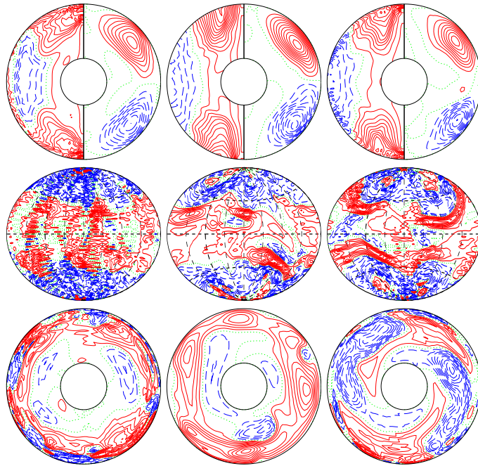
a.e03p002t06r-50000m1n2N2z13e5 E_{\text{kin}}
