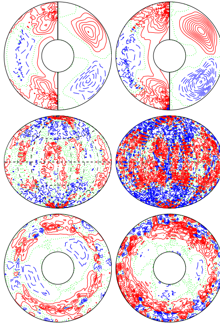
a.e03p003t06r-50000m1n2N2z17e5 E_{\text{kin}}
