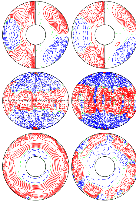
a.e03p003t06r-50000m1n2N2z13e5 E_{\text{kin}}
