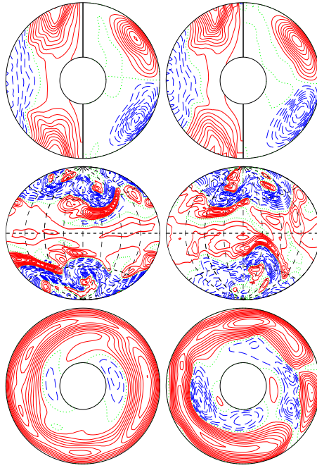
a.e03p003t06r-50000m1n2N2z9e5 E_{\text{kin}}
