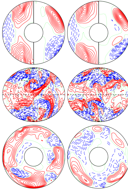
a.e03p003t1r-50000m1n2N2z16e5 E_{\text{kin}}
