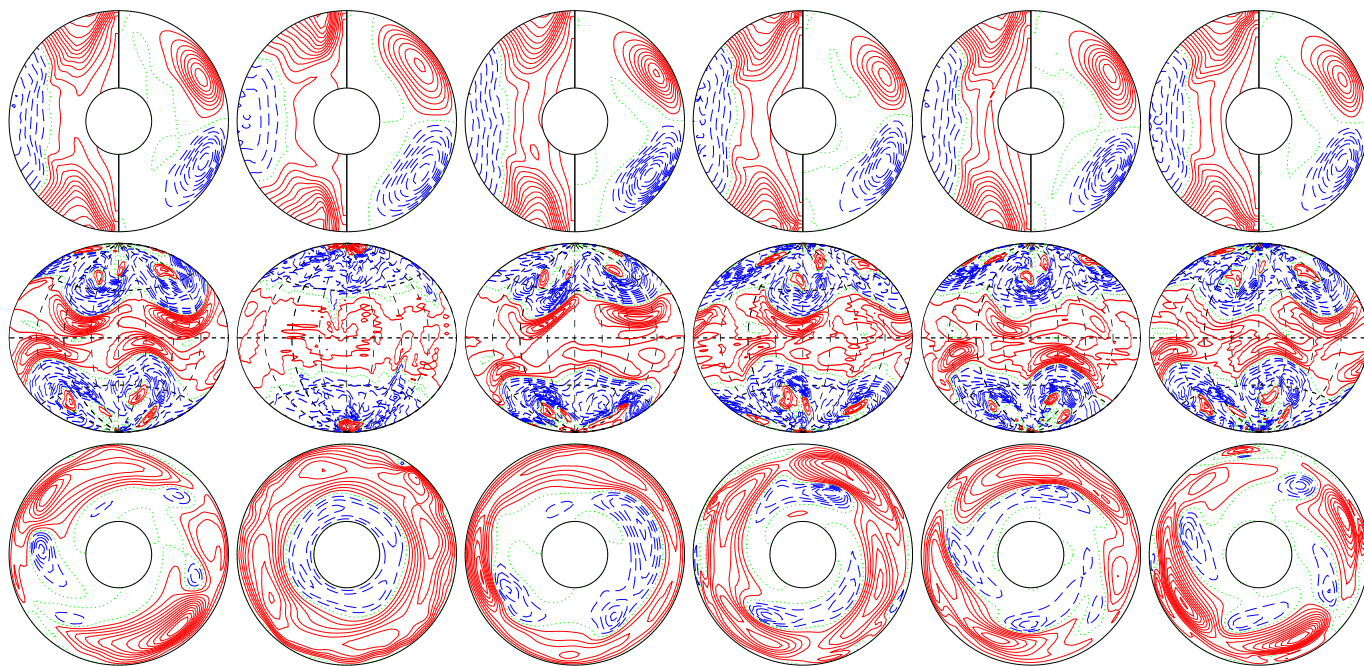
a.e03p001t06r-50000m1n2N2z9e5 E_{\text{kin}}
