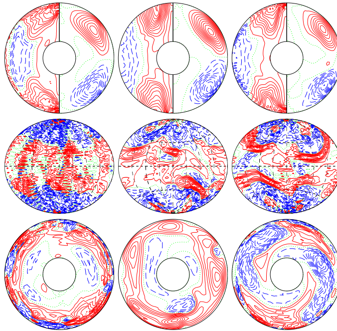
a.e03p002t06r-50000m1n2N2z13e5 E_{\text{kin}}
