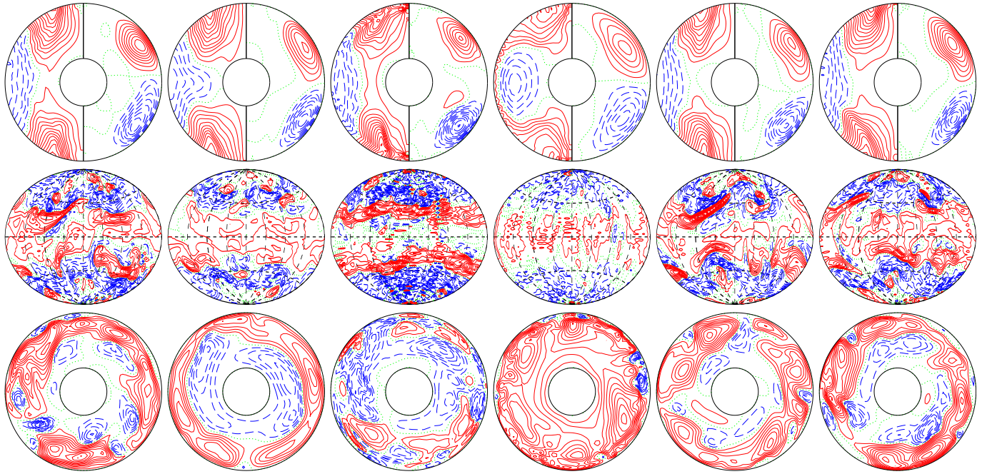
a.e03p002t1r-50000m1n2N2z17e5 E_{\text{kin}}
