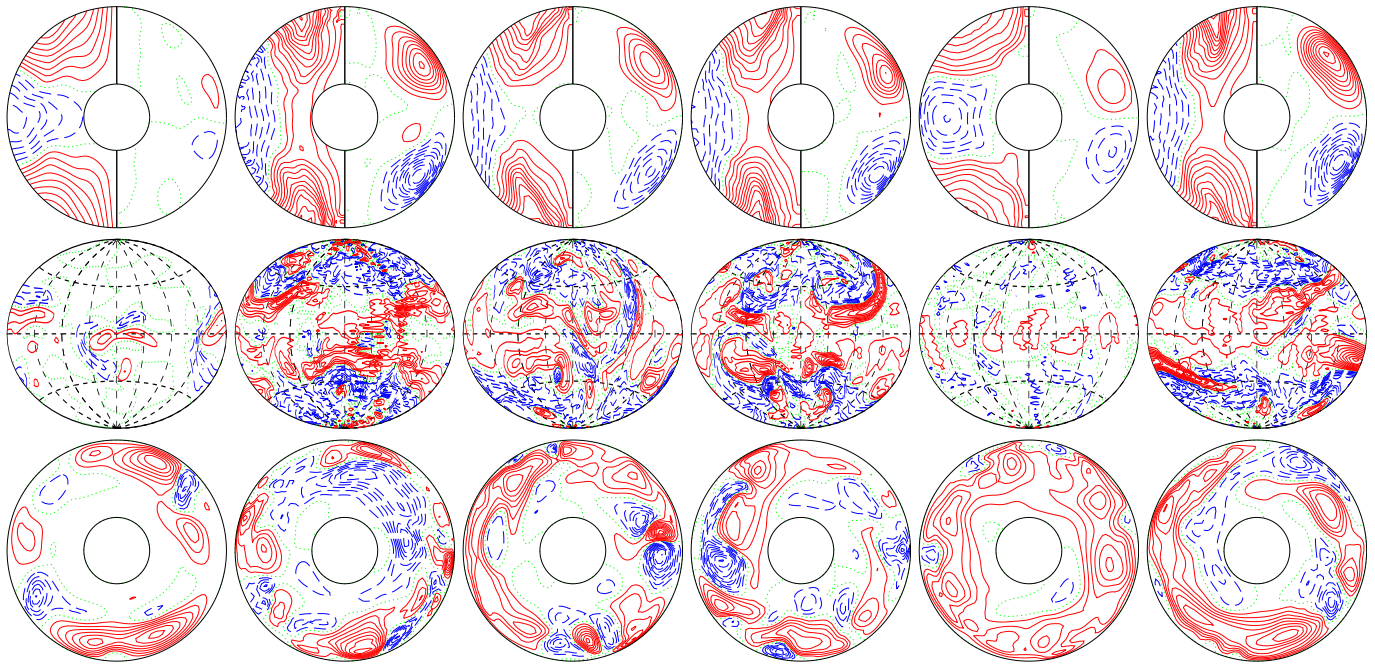
a.e03p003t1r-50000m1n2N2z15e5 E_{\text{kin}}
