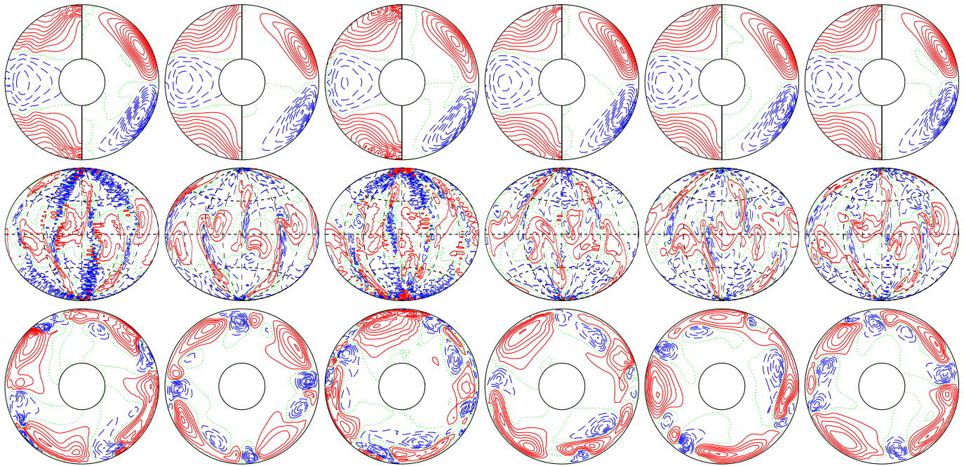
a.e03p002t1r-50000m1n2N2z13e5b E_{\text{kin}}
