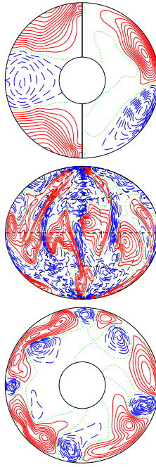
a.e03p003t1r-50000m1n2N2z12e5b E_{\text{kin}}
