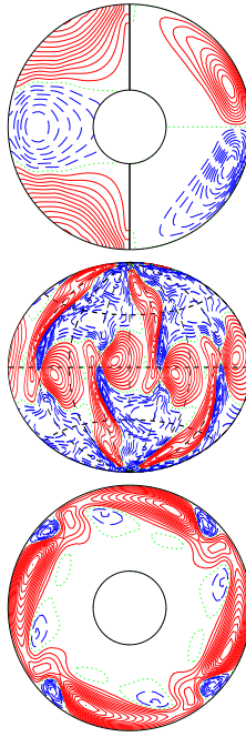
a.e03p003t1r-50000m1n2N2z10e5b E_{\text{kin}}
