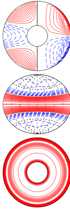
a.e03p003t1r-50000m1n2N2z5e5a E_{\text{kin}}
