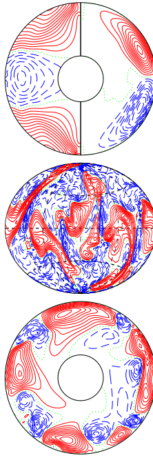
a.e03p003t1r-50000m1n2N2z11e5b E_{\text{kin}}
