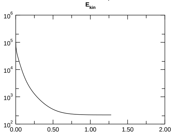
a.e03p003t1r-50000m1n2N2z5e4a
