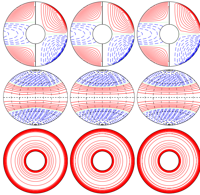
a.e03p003t1r-50000m1n2N2z5e4a E_{\text{kin}}
