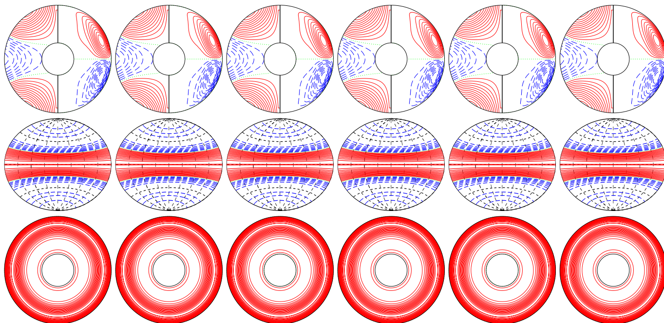
a.e03p005t03r-50000m1n2N2z8e4 E_{\text{kin}}
