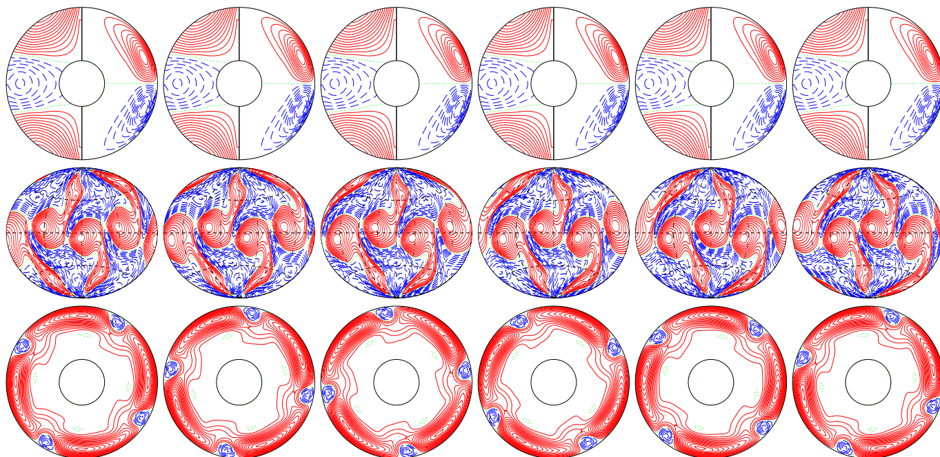
a.e03p005t06r-50000m1n2N2z33e4a E_{\text{kin}}
