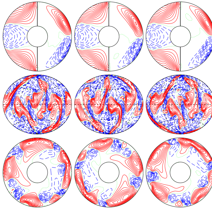
a.e03p003t1r-50000m1n2N2z11e5b E_{\text{kin}}
