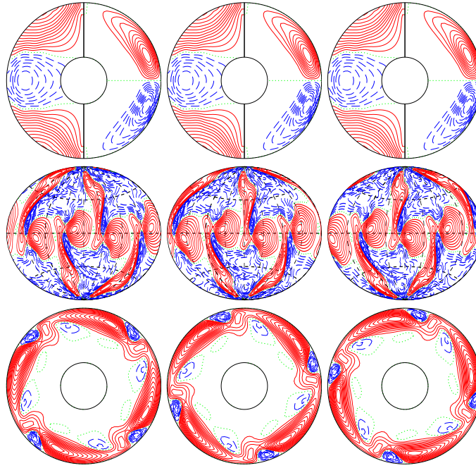
a.e03p003t1r-50000m1n2N2z10e5b E_{\text{kin}}
