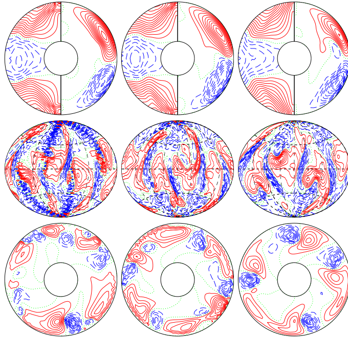
a.e03p003t1r-50000m1n2N2z13e5b E_{\text{kin}}
