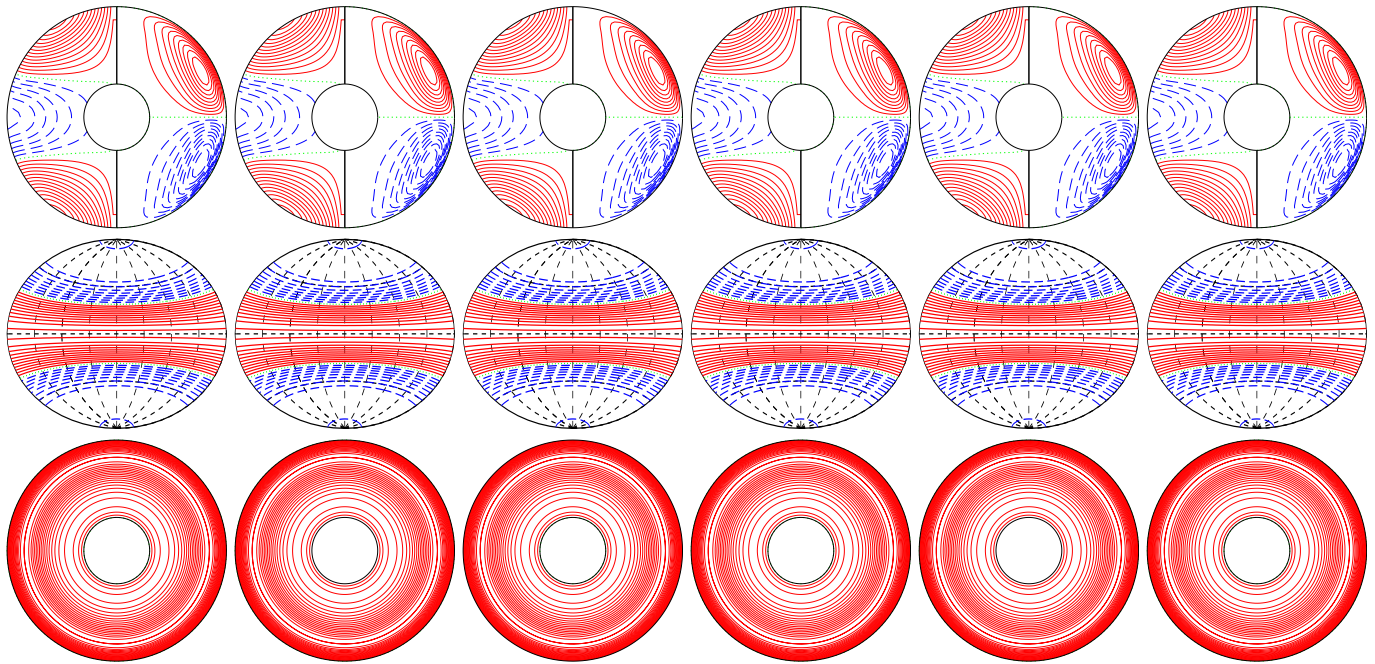
a.e03p005t03r-50000m1n2N2z4e4 E_{\text{kin}}
