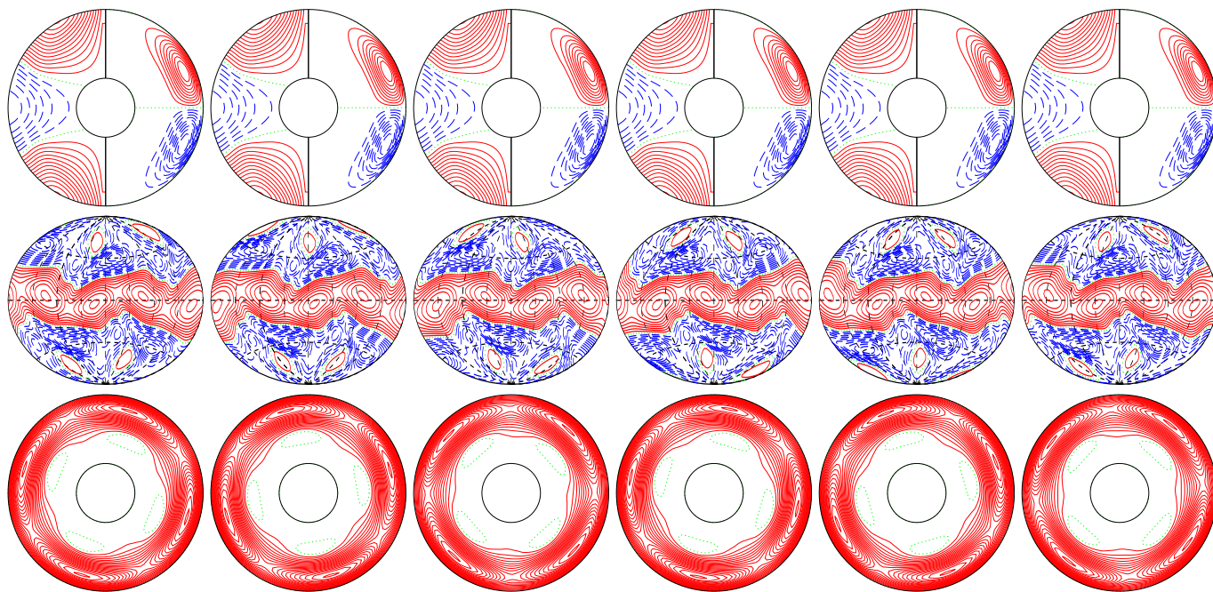
a.e03p005t03r-50000m1n2N2z12e4b E_{\text{kin}}
