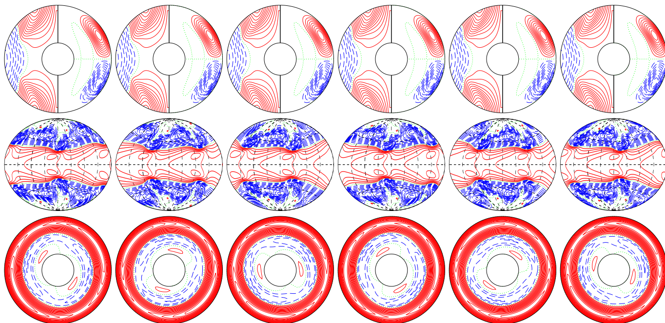
a.e03p005t03r-50000m1n2N2z16e4a E_{\text{kin}}
