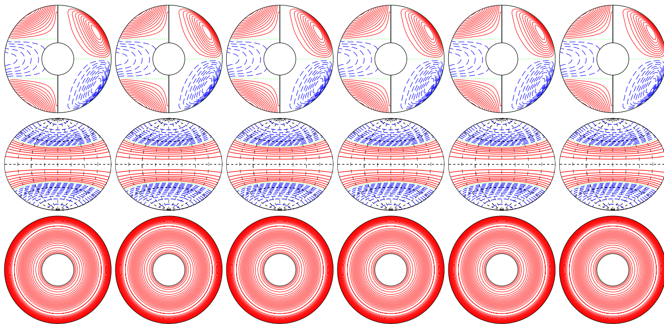
a.e03p005t03r-50000m1n2N2z1e4 E_{\text{kin}}
