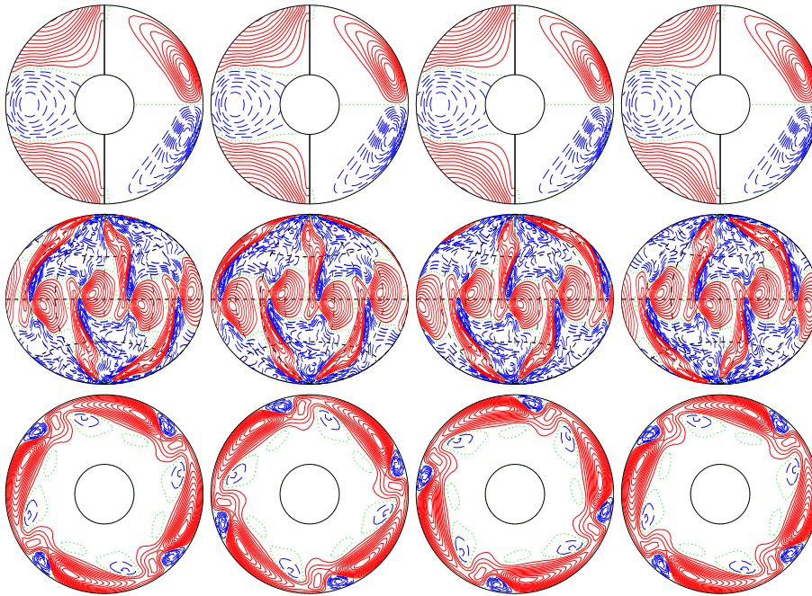
a.e03p003t1r-50000m1n2N2z10e5b E_{\text{kin}}
