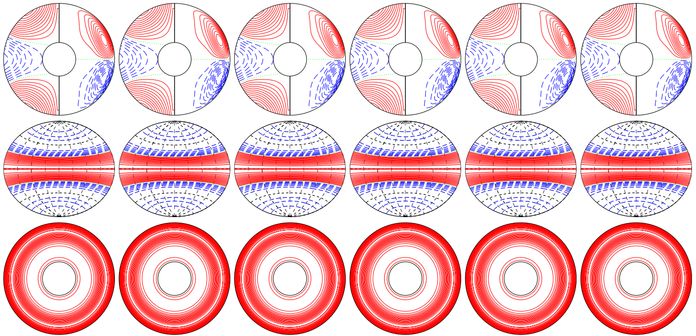
a.e03p005t03r-50000m1n2N2z8e4 E_{\text{kin}}
