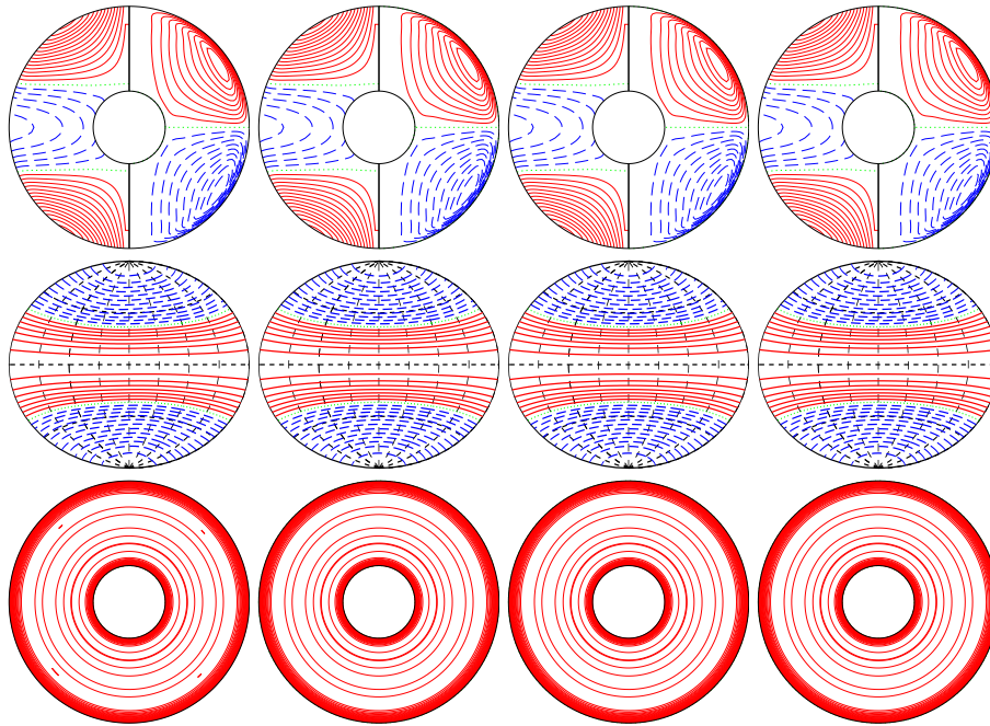
a.e03p003t1r-50000m1n2N2z1e5a E_{\text{kin}}
