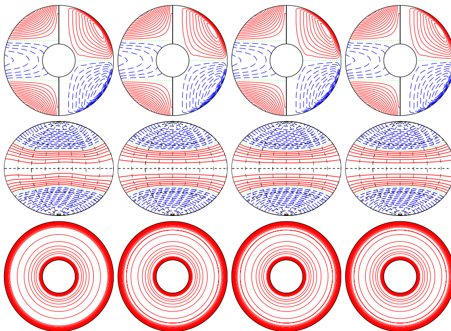
a.e03p003t1r-50000m1n2N2z5e4a E_{\text{kin}}
