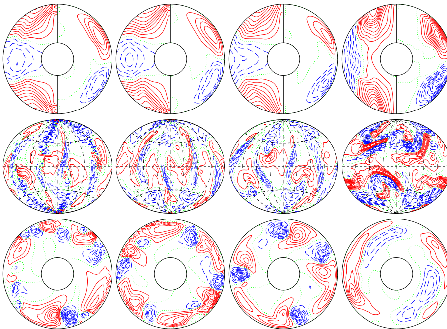
a.e03p003t1r-50000m1n2N2z13e5b E_{\text{kin}}
