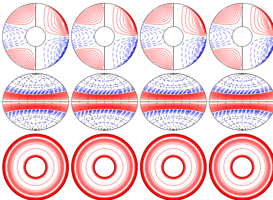
a.e03p003t1r-50000m1n2N2z5e5a E_{\text{kin}}
