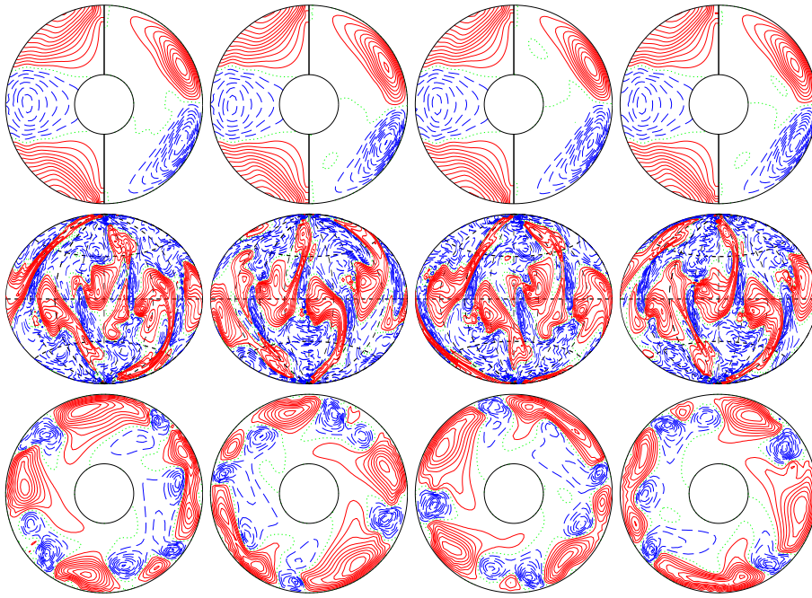
a.e03p003t1r-50000m1n2N2z11e5b E_{\text{kin}}
