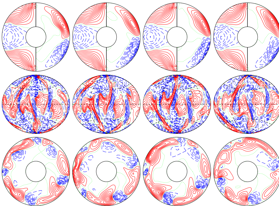
a.e03p003t1r-50000m1n2N2z12e5b E_{\text{kin}}
