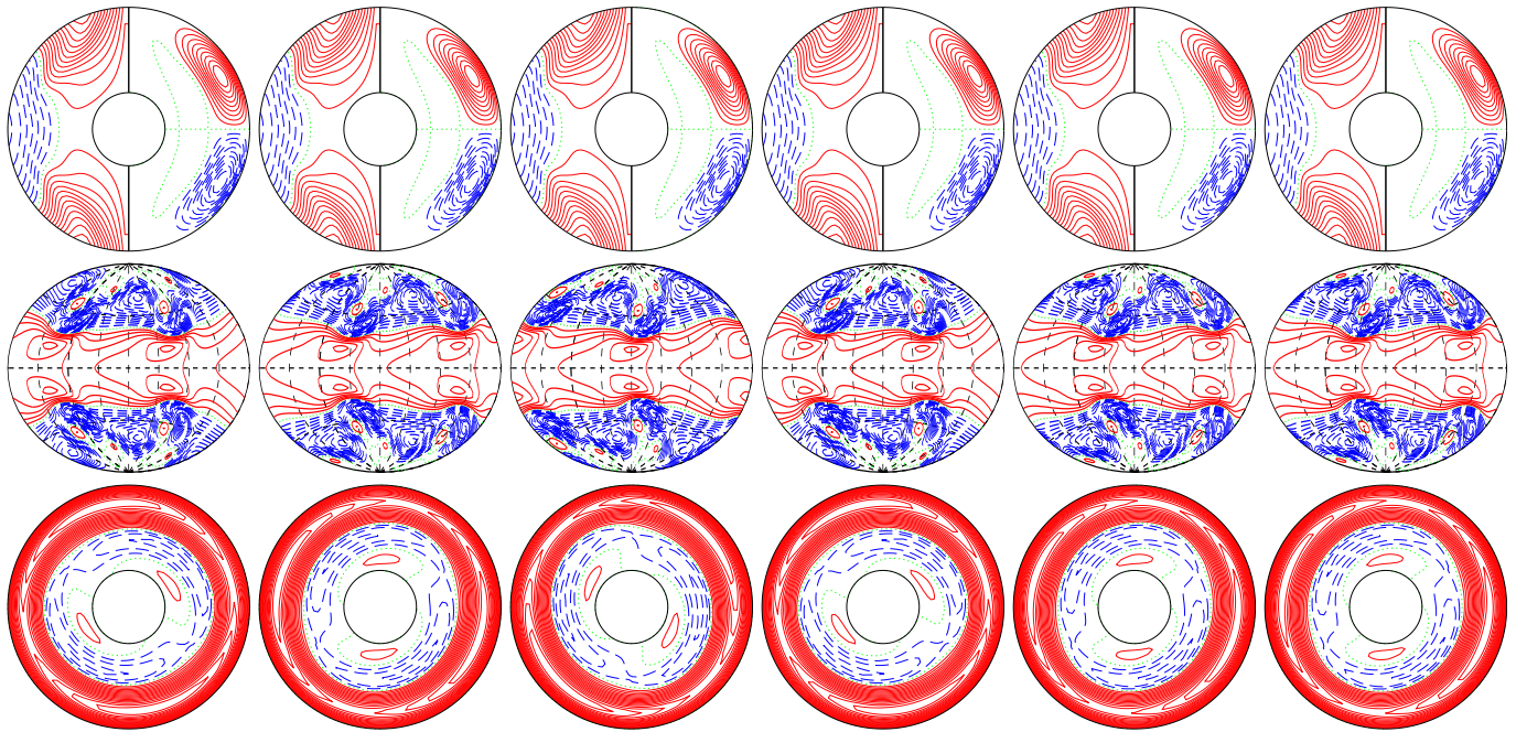
a.e03p005t03r-50000m1n2N2z18e4a E_{\text{kin}}
