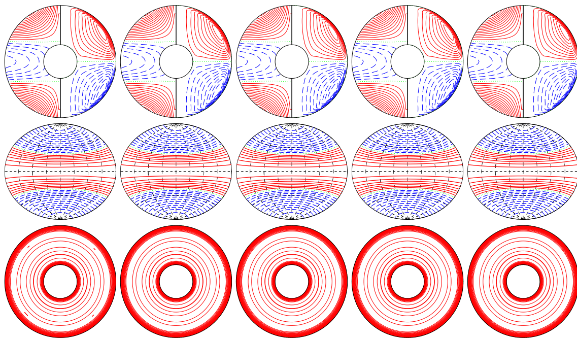
a.e03p003t1r-50000m1n2N2z1e5a E_{\text{kin}}
