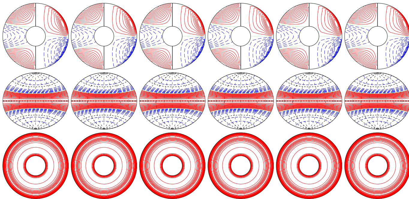
a.e03p003t1r-50000m1n2N2z5e5a E_{kin}
