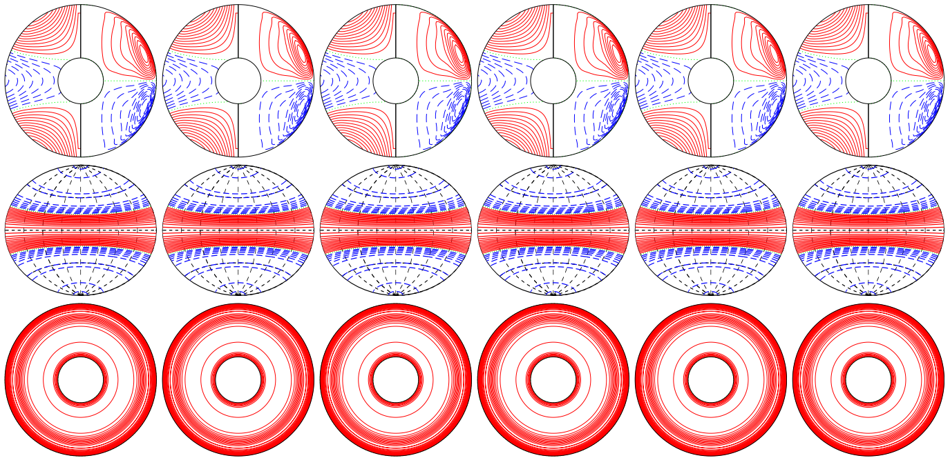
a.e03p003t1r-50000m1n2N2z6e5b E_{\text{kin}}
