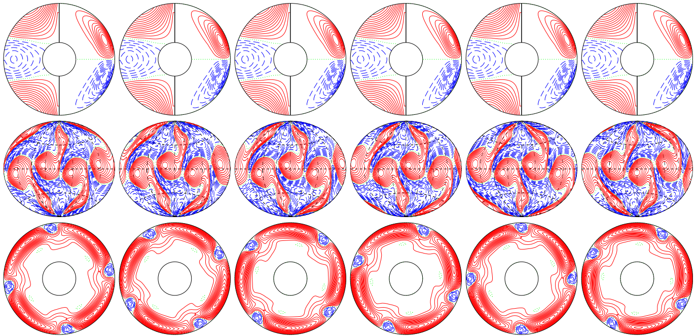
a.e03p005t06r-50000m1n2N2z33e4a E_{\text{kin}}
