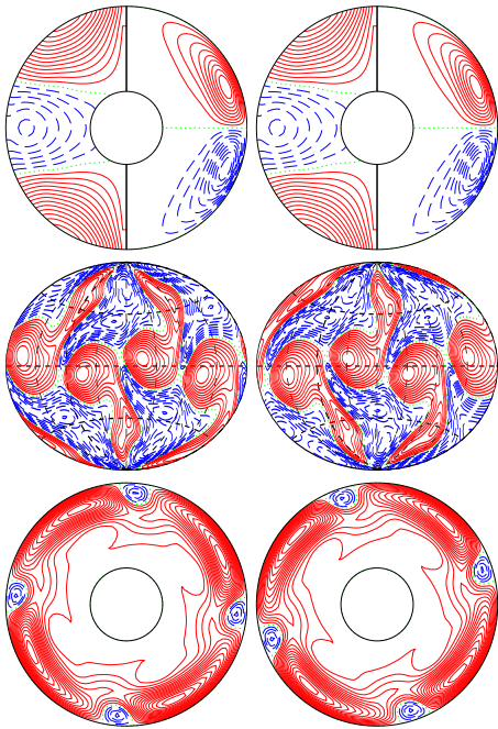
a.e03p005t06r-50000m1n2N2z31e4aA E_{\text{kin}}
