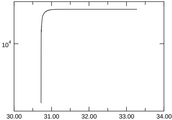
E_{kin,asymm.}
