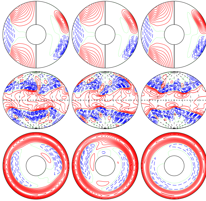
a.e03p005t06r-50000m1n2N2z33e4A E_{\text{kin}}
