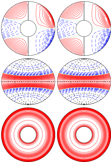
a.e03p005t06r-50000m1n2N2z23e4b E_{kin}
