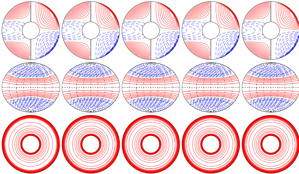
a.e03p003t1r-50000m1n2N2z5e4a E_{\text{kin}}
