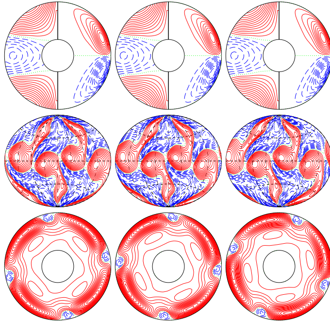
a.e03p005t06r-50000m1n2N2z30e4A E_{\text{kin}}
