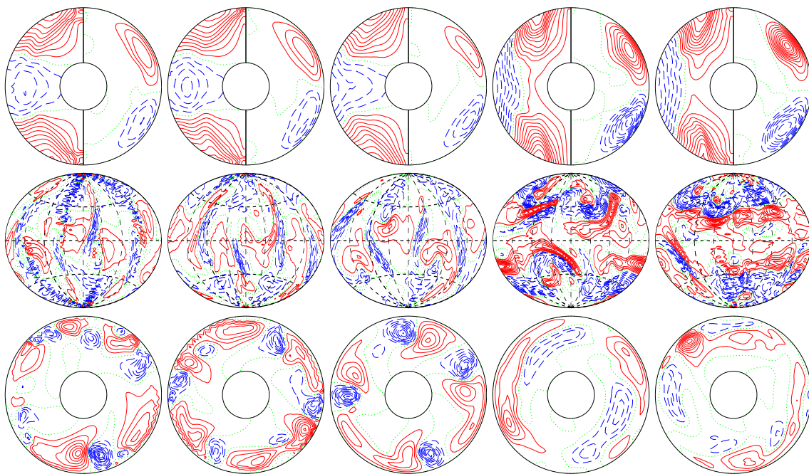
a.e03p003t1r-50000m1n2N2z13e5b E_{kin}
