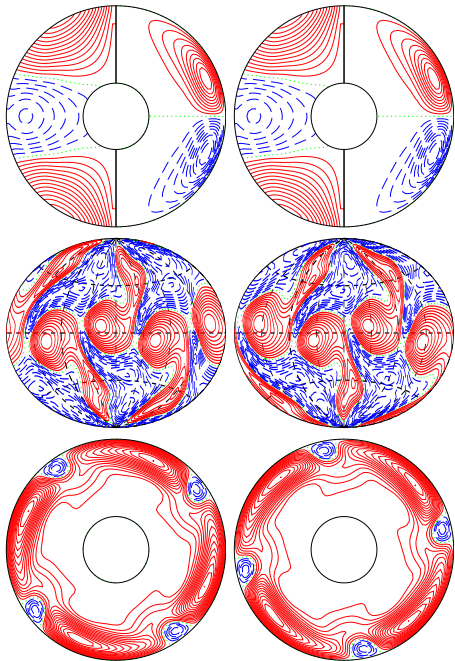
a.e03p005t06r-50000m1n2N2z32e4aA E_{\text{kin}}
