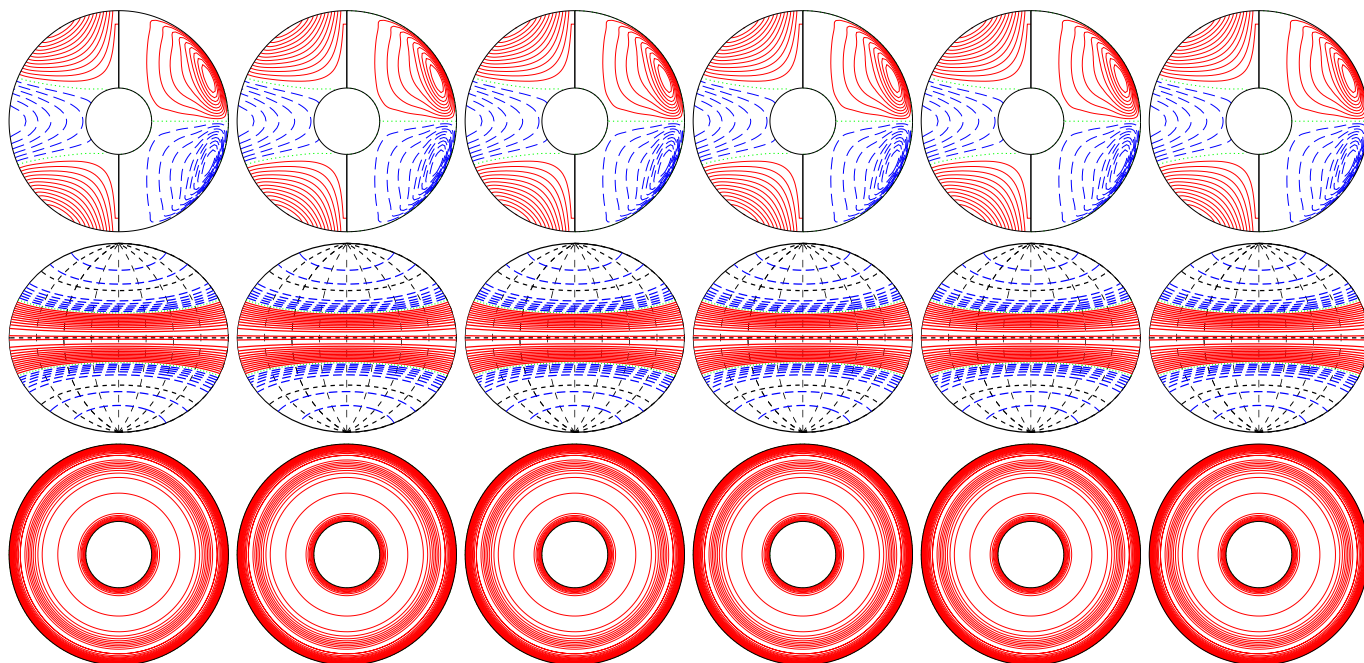
a.e03p003t1r-50000m1n2N2z5e5a E_{\text{kin}}
