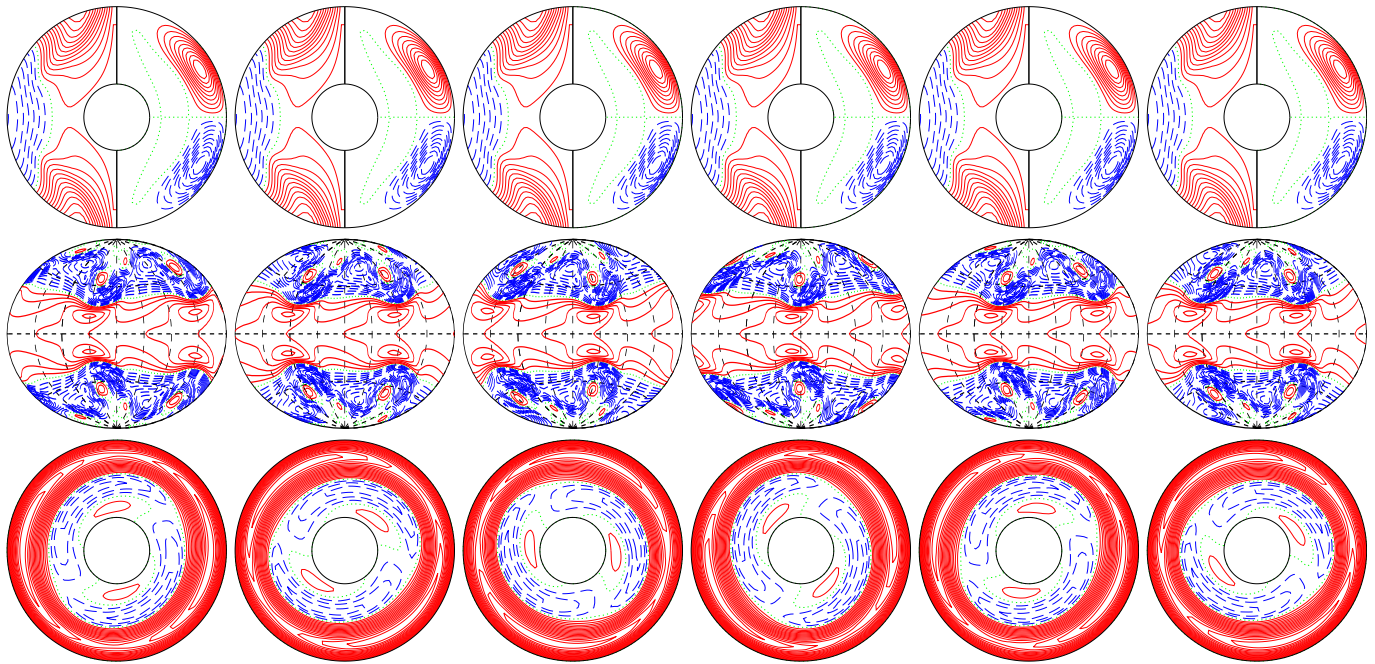
a.e03p005t03r-50000m1n2N2z20e4 E_{\text{kin}}
