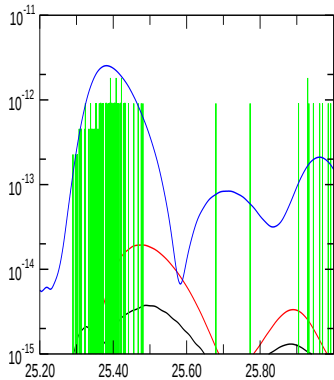
E_{kin,asymm.}
