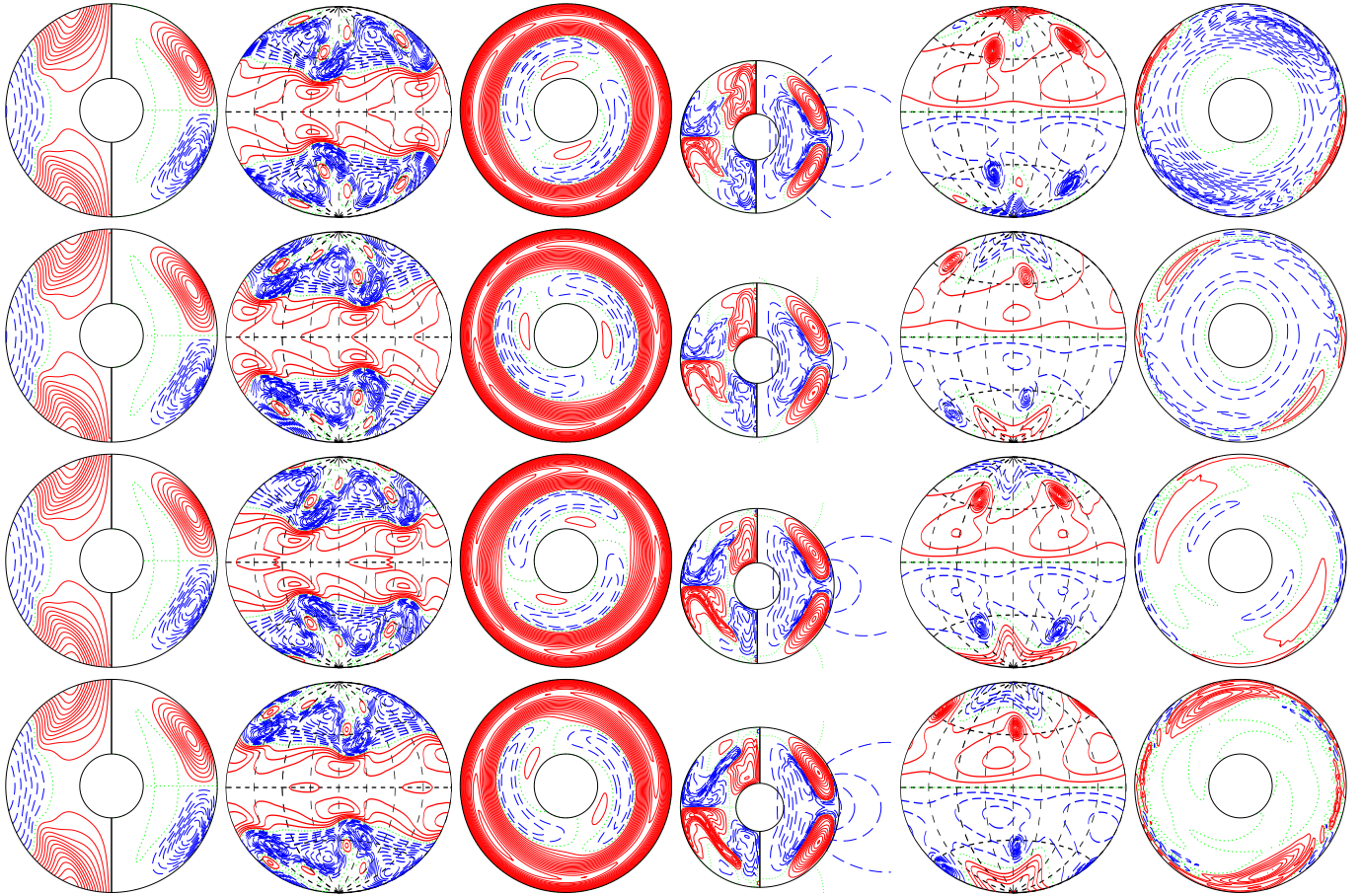
a.e03p005t03r-50000m2p14n2N2z20e4 E_{kin}
