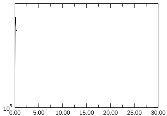
E_{kin,asymm.}
