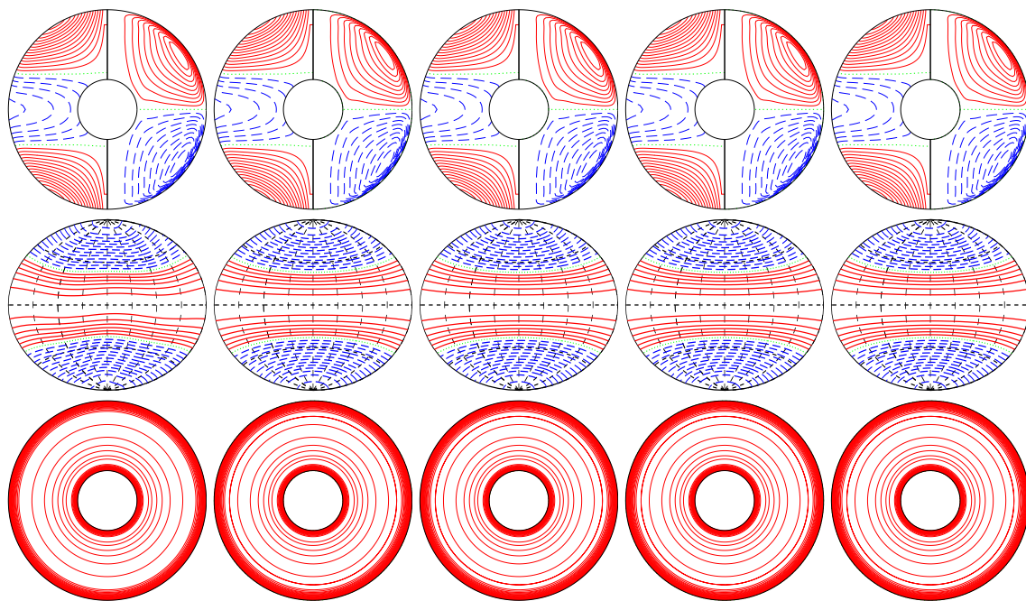
a.e03p003t1r-50000m1n2N2z5e4a E_{\text{kin}}
