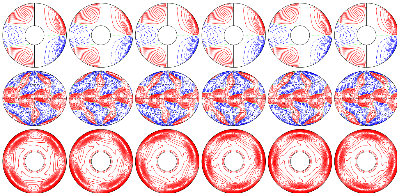
a.e03p005t06r-50000m1n2N2z25e4a E_{\text{kin}}
