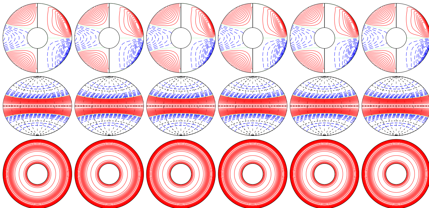
a.e03p005t06r-50000m1n2N2z23e4a E_{\text{kin}}
