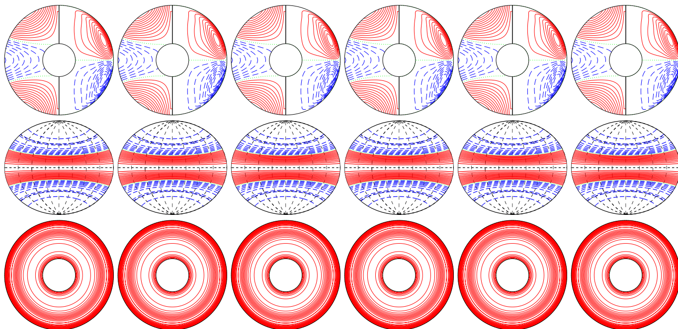
a.e03p005t06r-50000m1n2N2z21e4a E_{\text{kin}}
