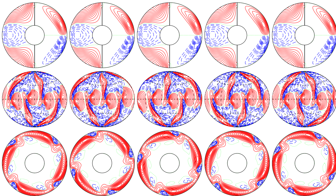
a.e03p003t1r-50000m1n2N2z10e5b E_{kin}
