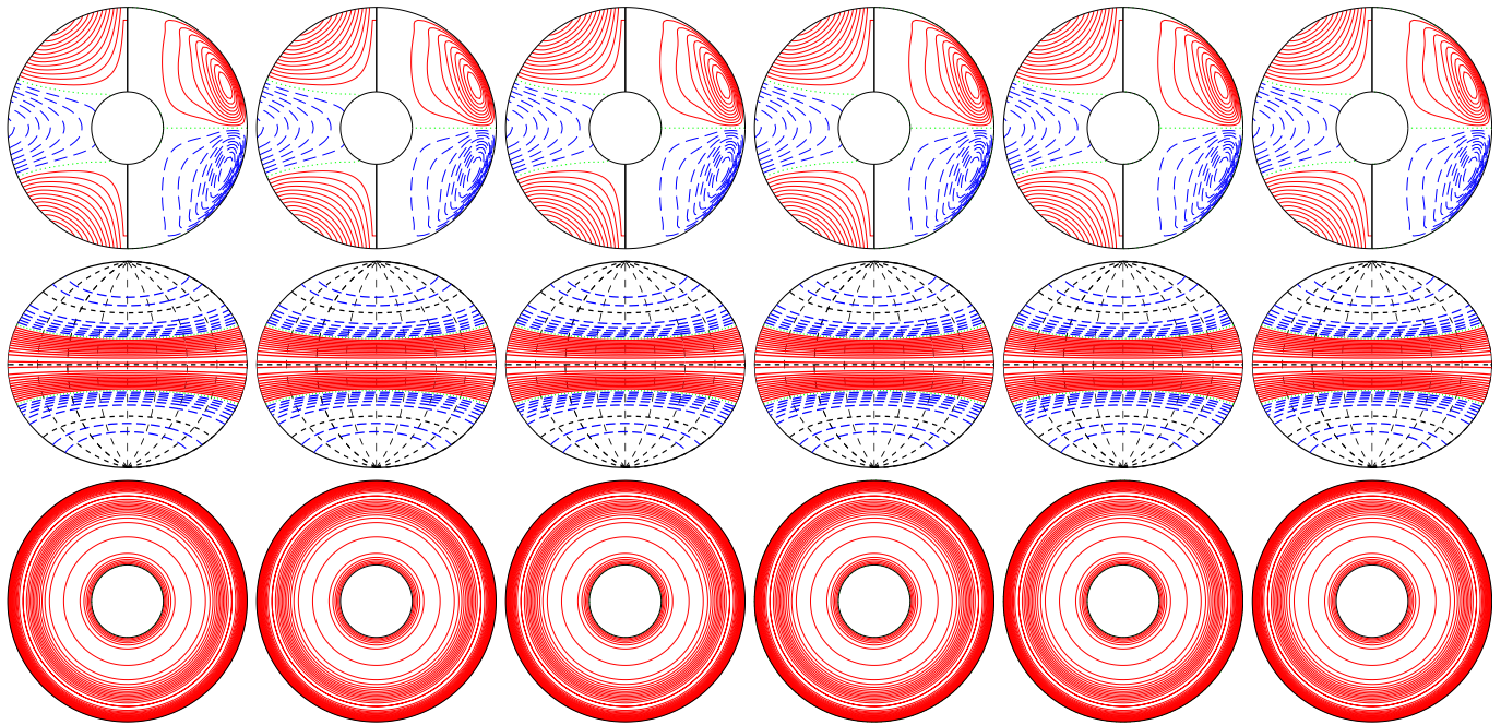
a.e03p005t06r-50000m1n2N2z23e4b E_{\text{kin}}
