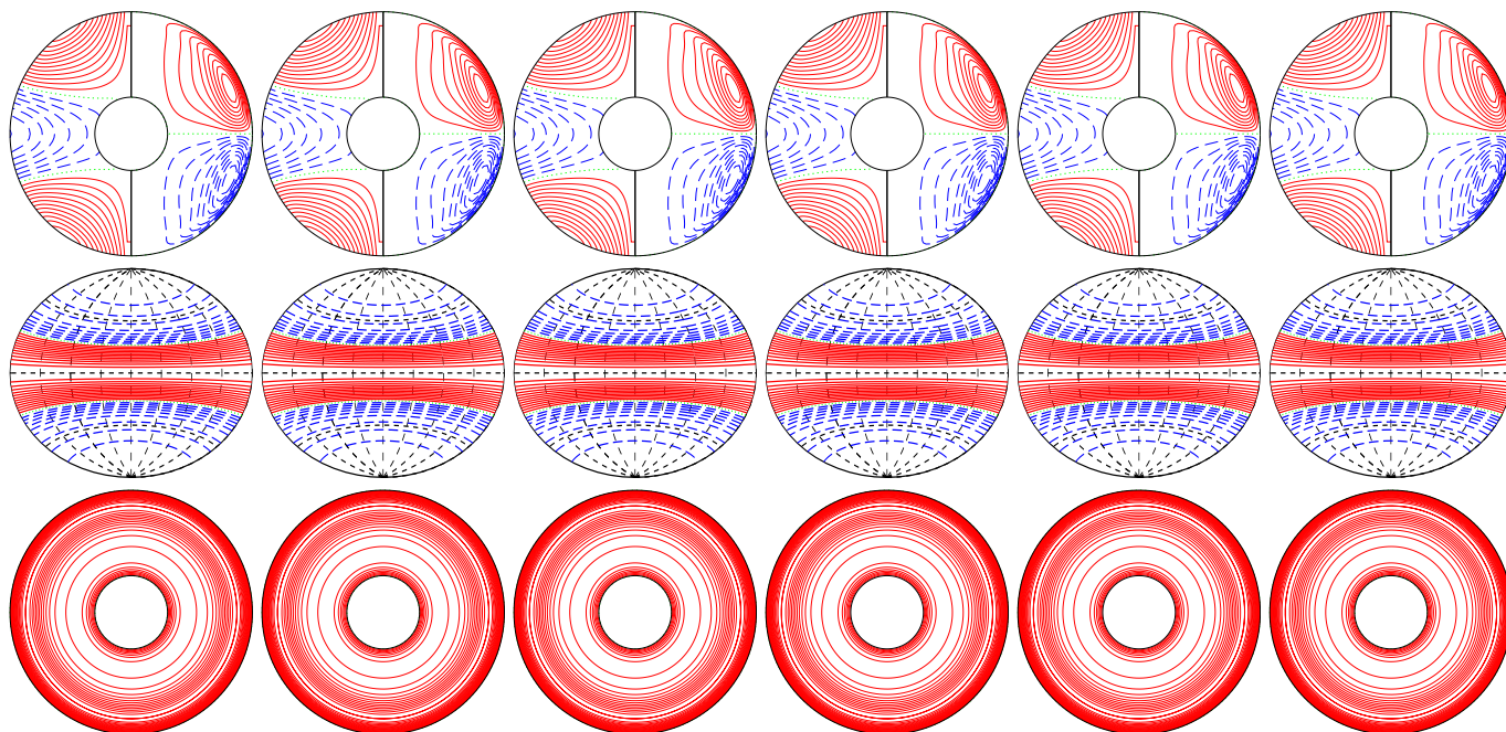
a.e03p005t06r-50000m1n2N2z20e4a E_{\text{kin}}
