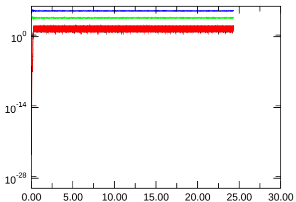
E_{kin,asymm.}
