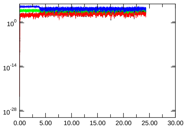
E_{kin,asymm.}
