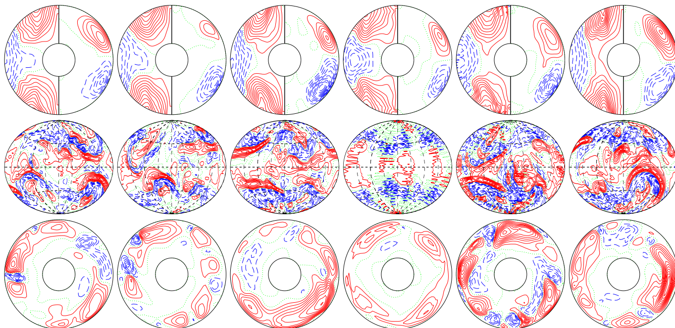
a.e03p003t1r-50000m1n2N2z15e5 E_{\text{kin}}
