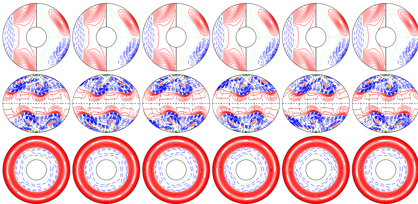
a.e03p005t03r-50000m1n2N2z23e4b E_{\text{kin}}
