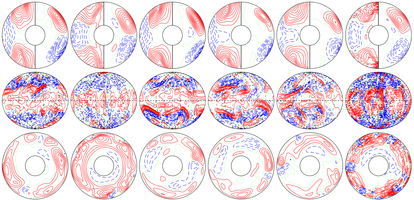
a.e03p003t1r-50000m1n2N2z16e5 E_{\text{kin}}
