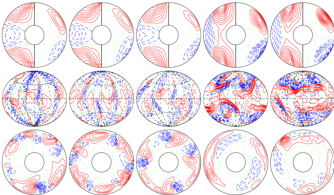
a.e03p003t1r-50000m1n2N2z13e5b E_{kin}
