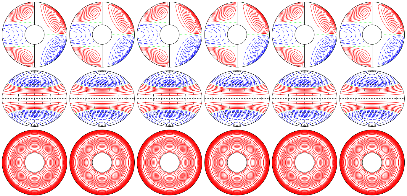
a.e03p005t03r-50000m1n2N2z1e4 E_{\text{kin}}
