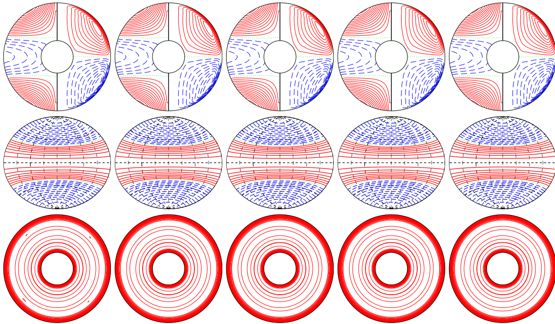
a.e03p003t1r-50000m1n2N2z1e5a E_{\text{kin}}
