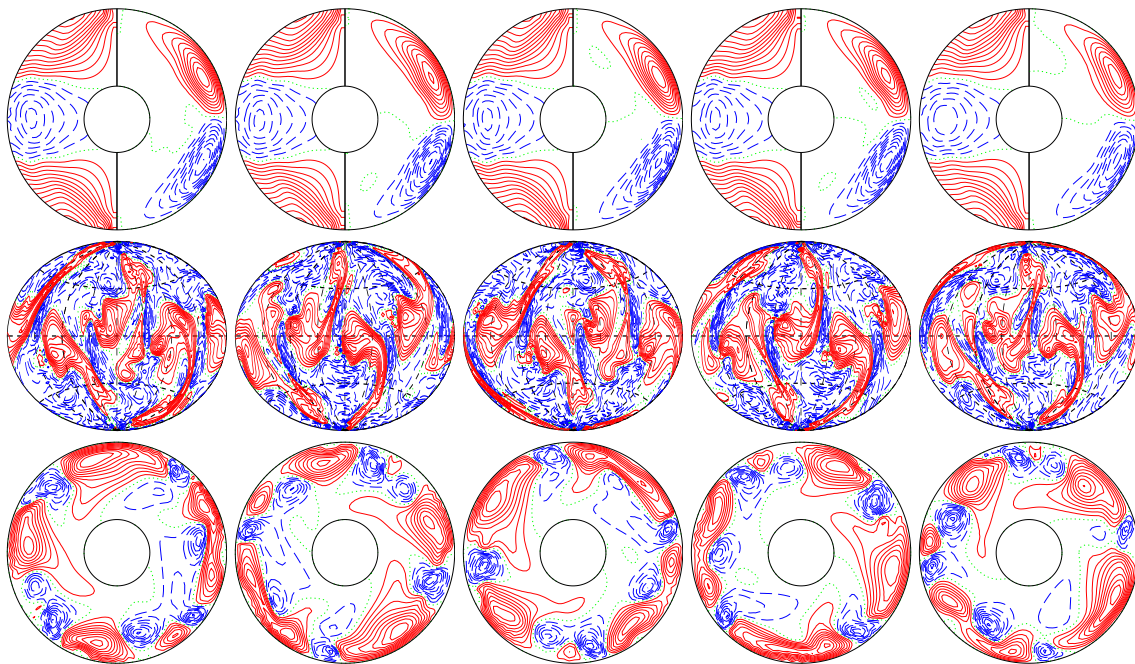
a.e03p003t1r-50000m1n2N2z11e5b E_{kin}
