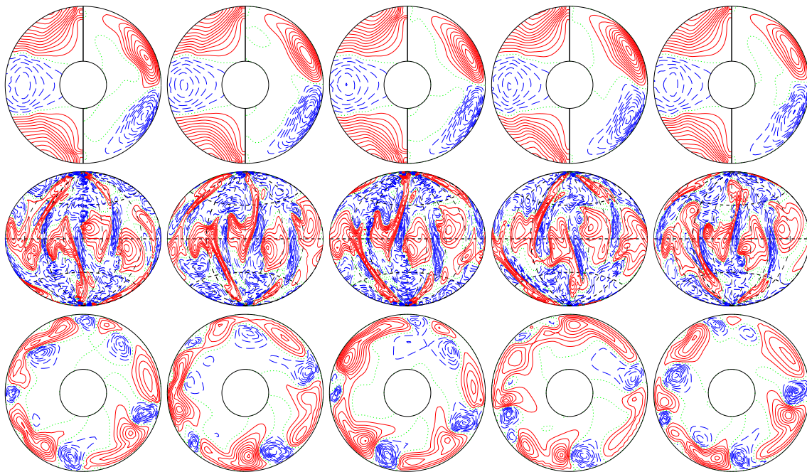
a.e03p003t1r-50000m1n2N2z12e5b E_{\text{kin}}
