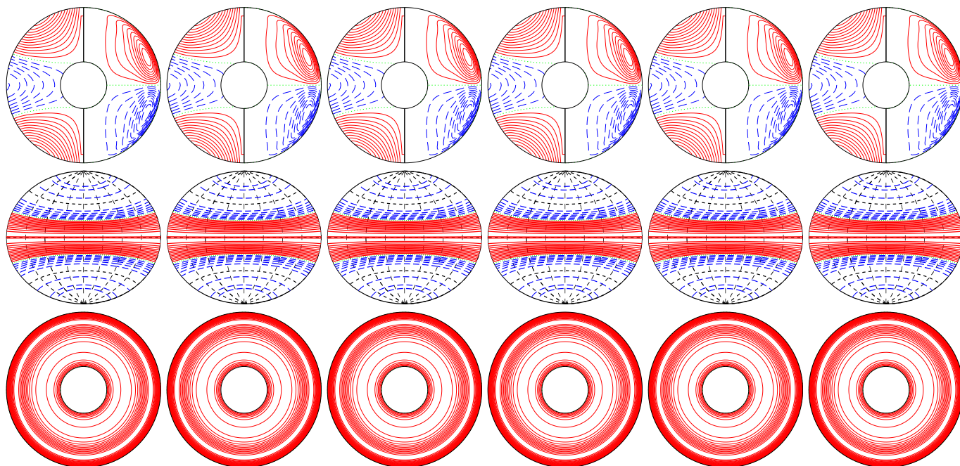
a.e03p005t06r-50000m1n2N2z22e4a E_{\text{kin}}
