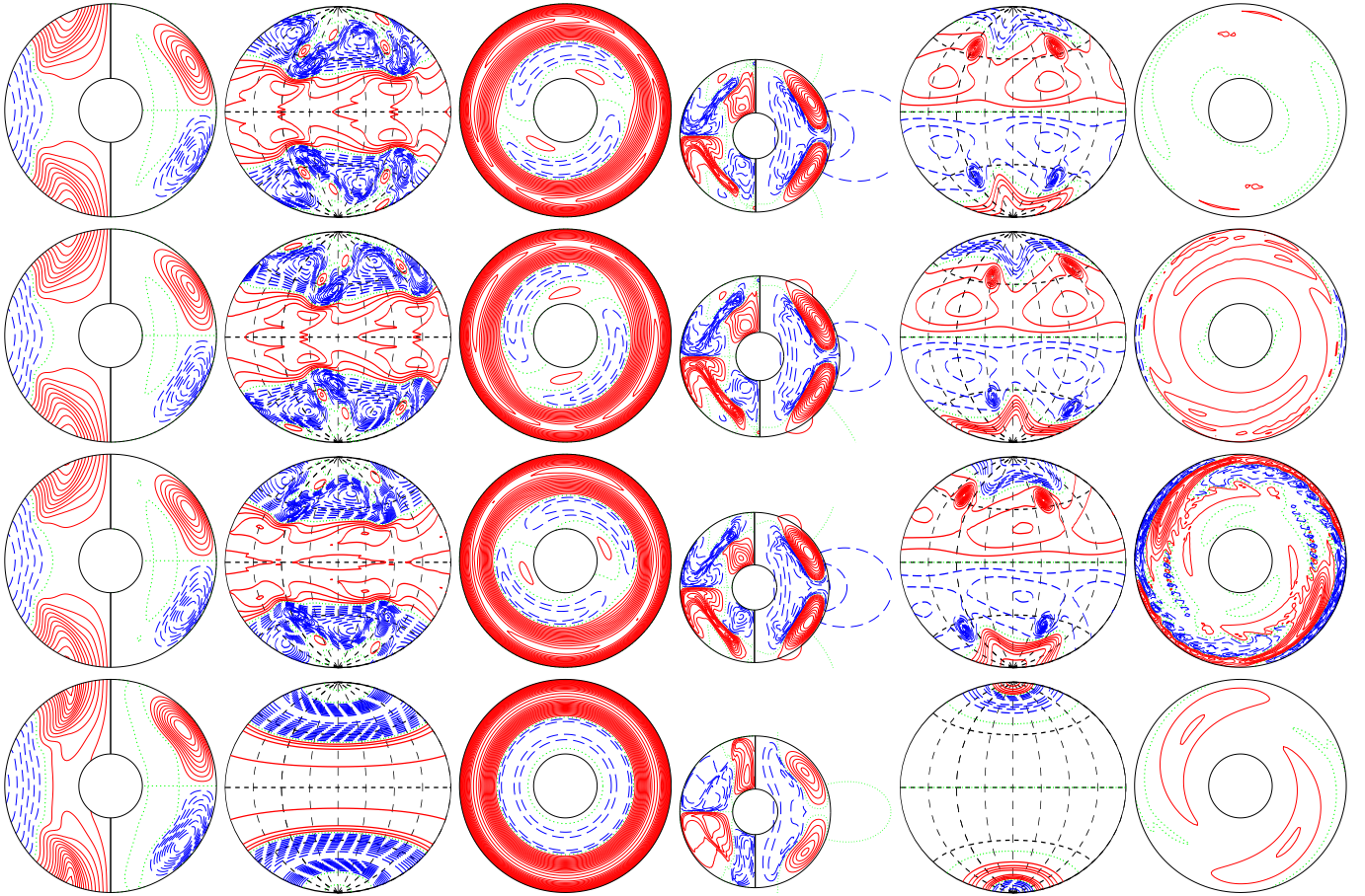
a.e03p005t03r-50000m2p14n2N2z20e4 E_{\text{kin}}
