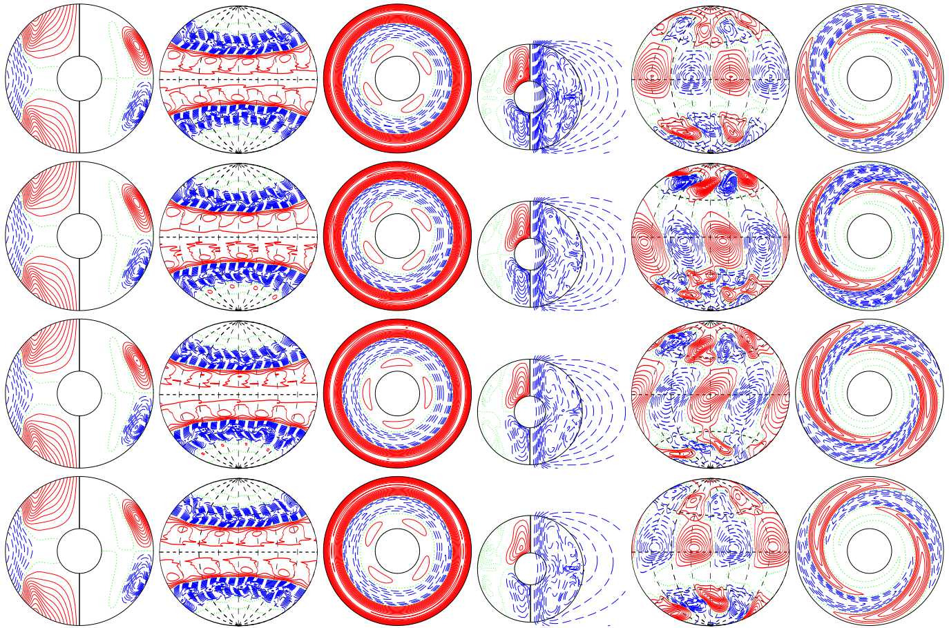
a.e03p005t06r-50000m2p16n2N2z32e4 E_{\text{kin}}
