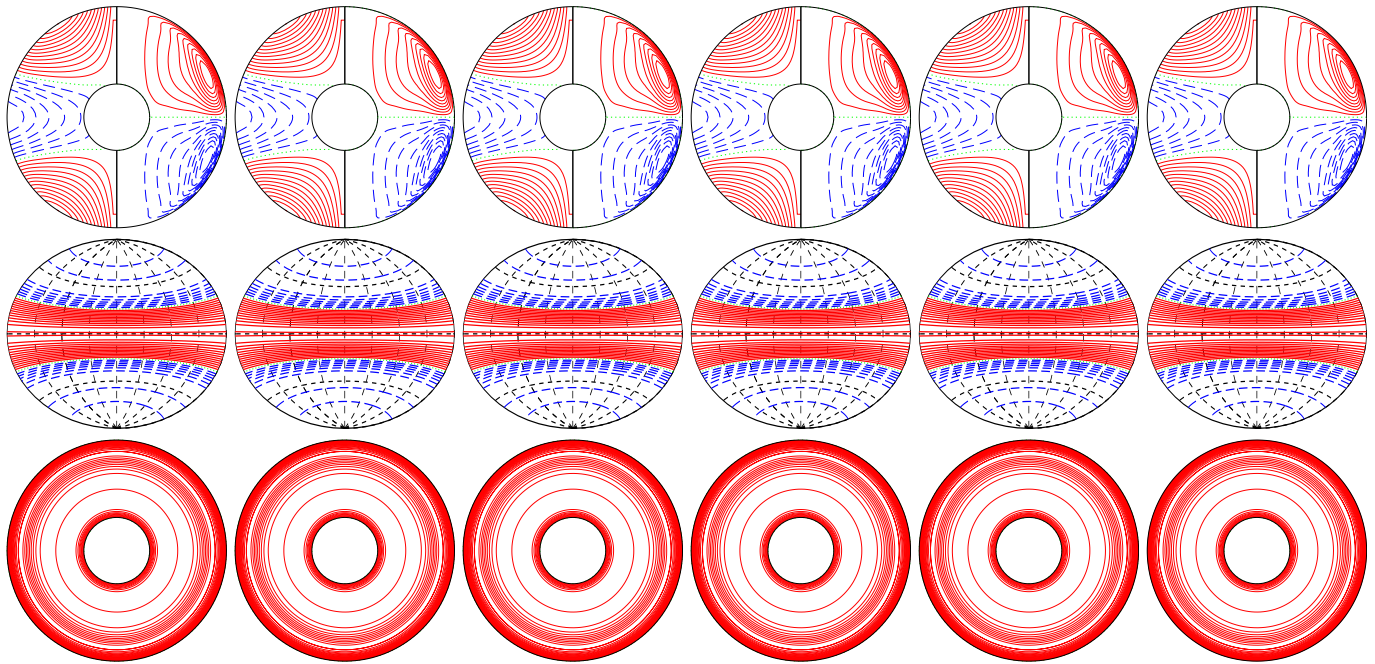
a.e03p003t1r-50000m1n2N2z5e5a E_{\text{kin}}
