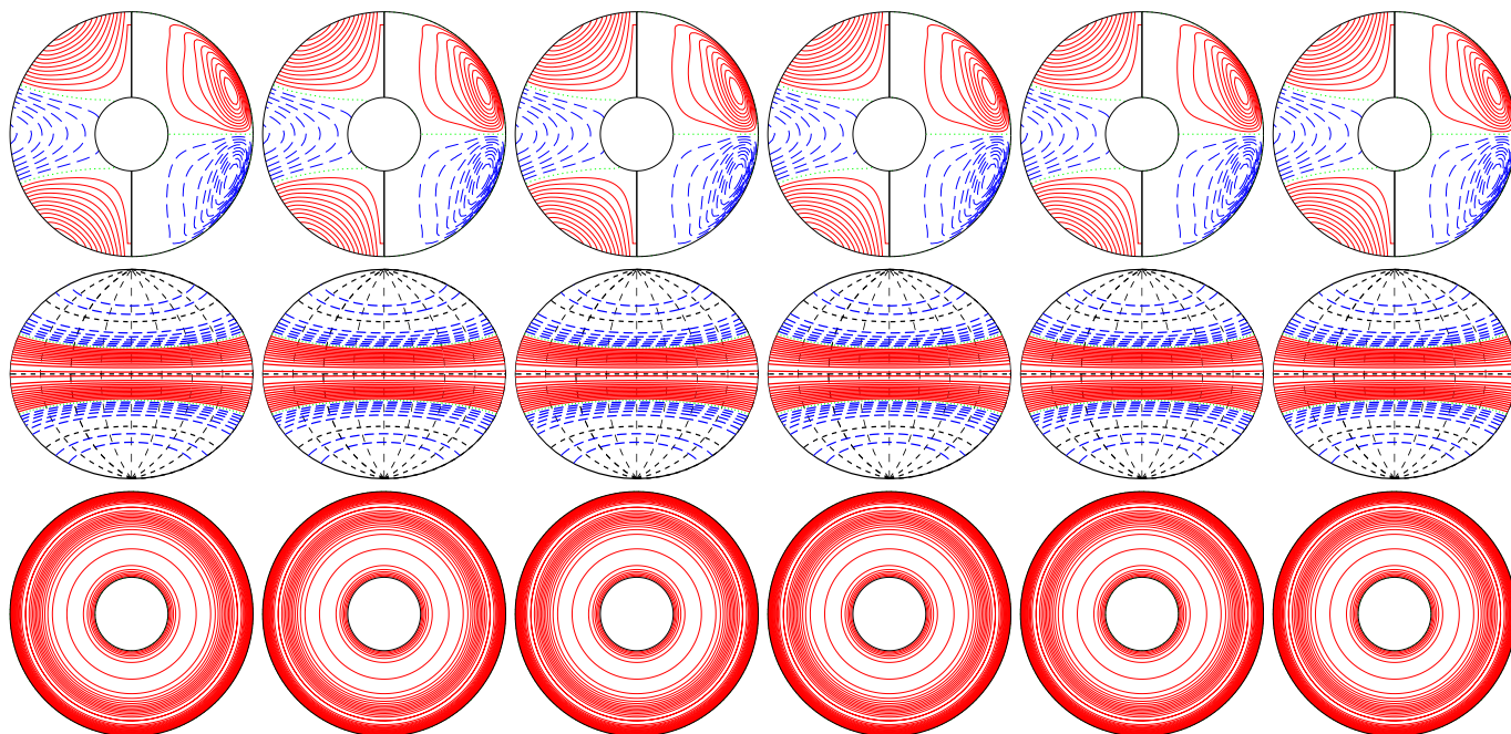
a.e03p005t06r-50000m1n2N2z23e4b E_{\text{kin}}
