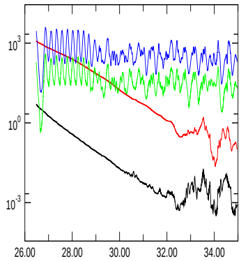
E_{\text{magn, dip.}}
