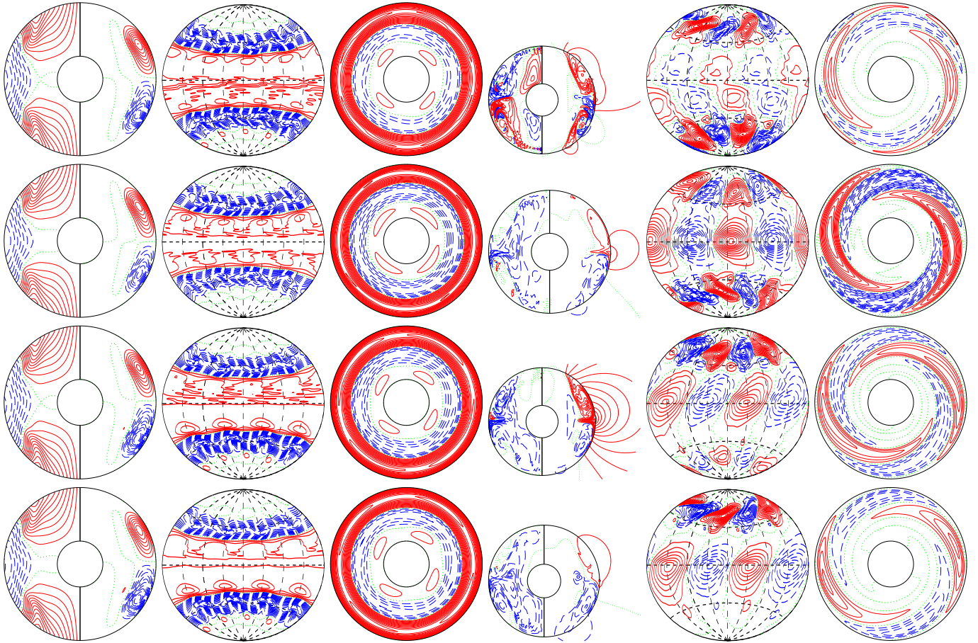
a.e03p005t06r-50000m2p16n2N2z32e4 E_{\text{kin}}
