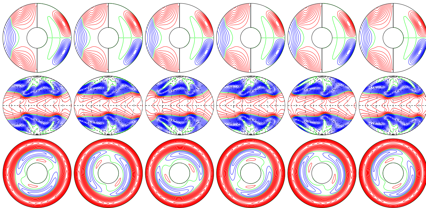
a.e03p01t03r-50000m1n2N2z14e4bb E_{\text{kin}}
