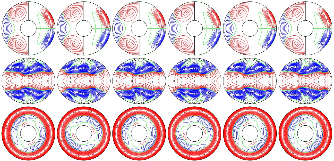
a.e03p01t03r-50000m1n2N2z13.5e4b E_{\text{kin}}
