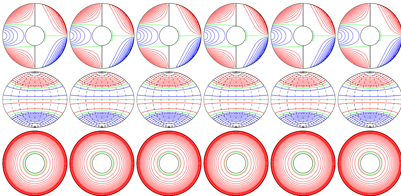
a.e03p1t10r-10m1n2N3z1e6 E_{\text{kin}}
