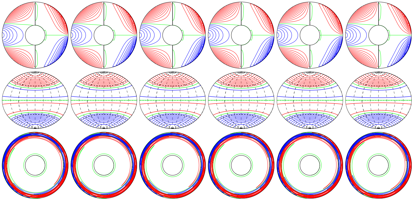
a.e03p1t10r-10m1n2N3z0995e7 E_{\text{kin}}
