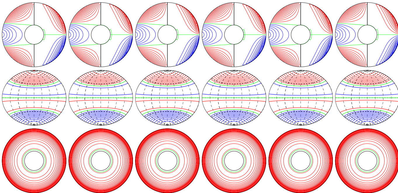
a.e03p1t10r-10m1n2N3z099e7 E_{\text{kin}}
