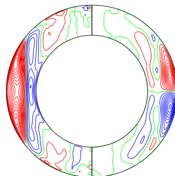
\bar{u}_\phi & merid circulation (mer) (time-average 14.55815 to 14.59315)
